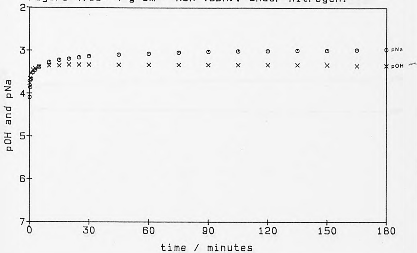
Figure 4.15: 4 g dm -3 NaX (BDH). Under nitrogen.
