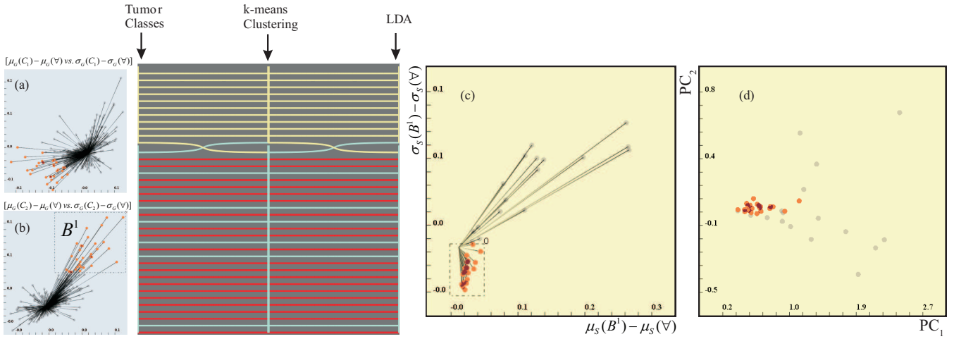
Figure 6: Through deviation plots (a) [\mu_G(C_1) - \mu_G(\forall), \sigma_G(C_1) - \sigma_G(\forall)] and (b) [\mu_G(C_2) - \mu_G(\forall), \sigma_G(C_2) - \sigma_G(\forall)] , a user can spot genes that are significantly expressed for classes C_1 and C_2 respectively. After performing a brush selection in (b), having significant values with respect to class C_2 , we perform k -means clustering and LDA and produce them into the Categorical View. The deviation plot on samples (c) shows statistics on the samples [\mu_S(B^1) - \mu_S(\forall), \sigma_S(B^1) - \sigma_S(\forall)] while the Dynamic PCA plot displays projection of samples onto two principal components ( PC_1, PC_2 ) computed only by means of the genes in brush (b). We brush a small group of tightly placed in samples in (c) and through the linked views, we observe the highlighted samples in the categorical view. The categorical view depicts the resulting classes in the clustering and the LDA results, together with the tumor classes in the leftmost axis.
