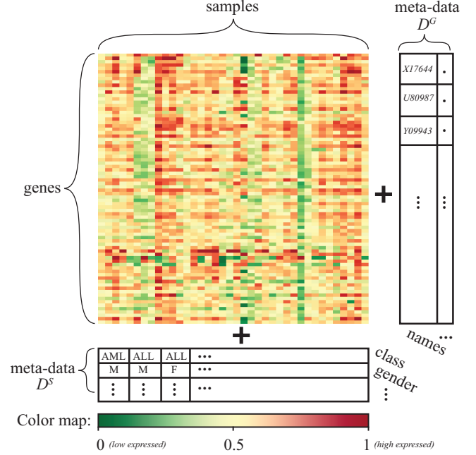
Figure 2: An illustration to depict the structure of the microarray data M . There are meta data columns associated with both the samples D^S and the genes D^G . The color map below is used to color the heat map visualization accordingly to the expression levels of the genes.
