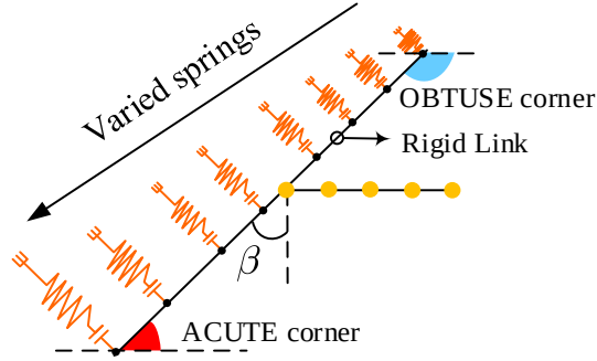
Fig. 9. Soil springs simulation for skewness
