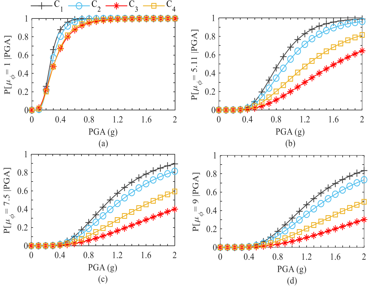
Fig. 13. Fragility curves for column curvature ductility demand considering four different structural systems with 0^\circ skew angle at (a) slight, (b) moderate, (c) extensive, and (d) complete limit states
