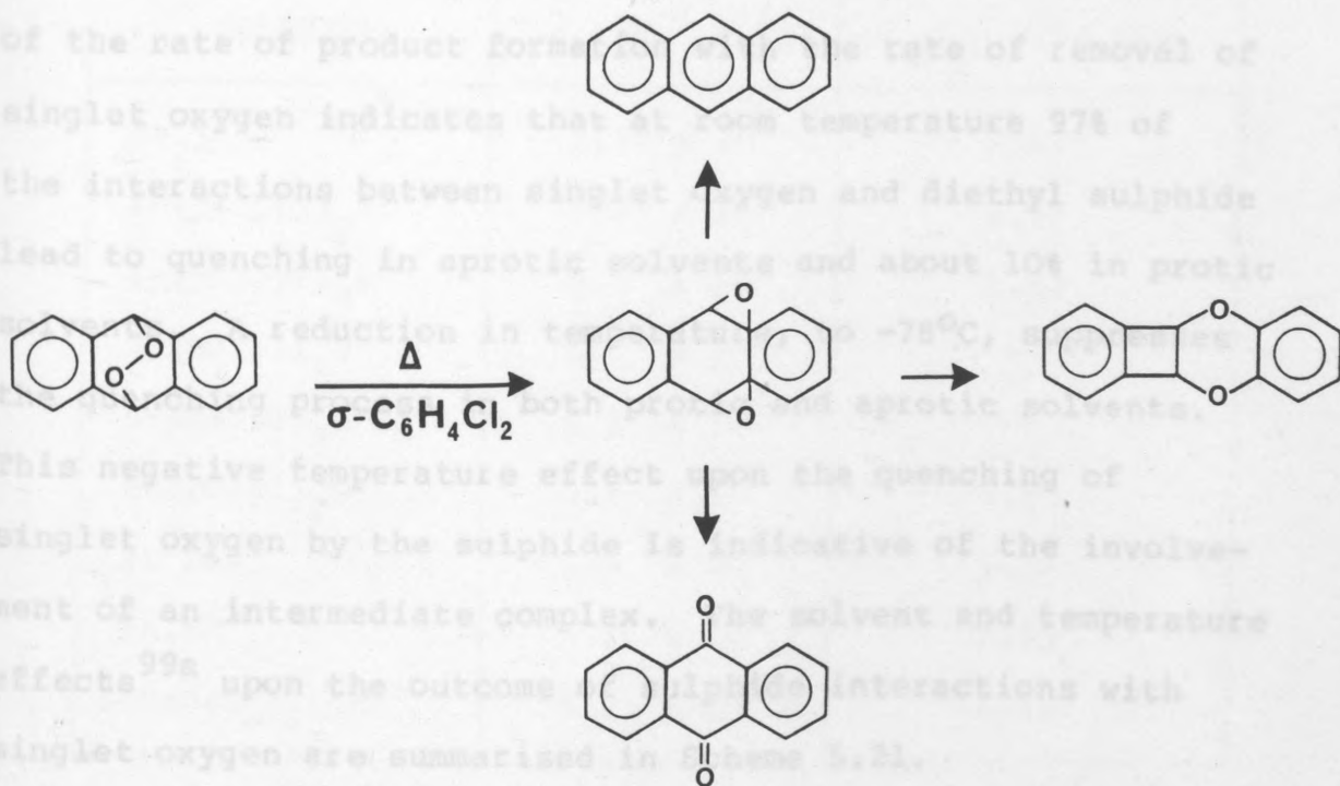
Scheme 5.20
