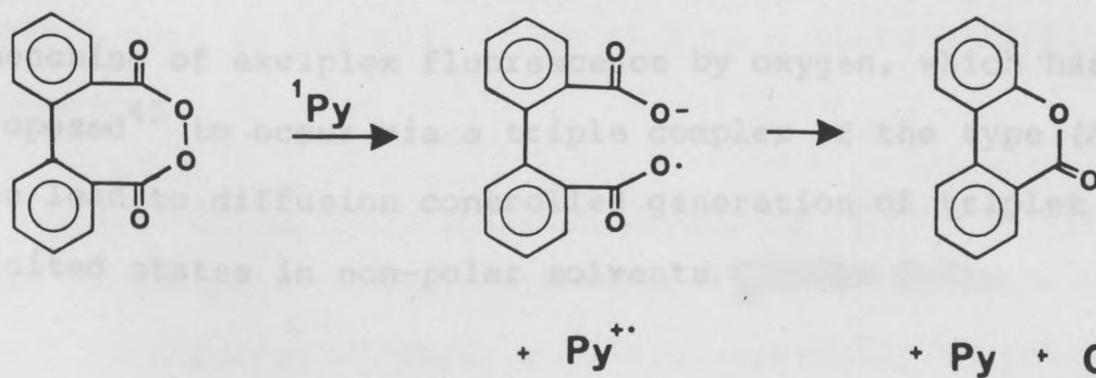
Scheme 2.7
