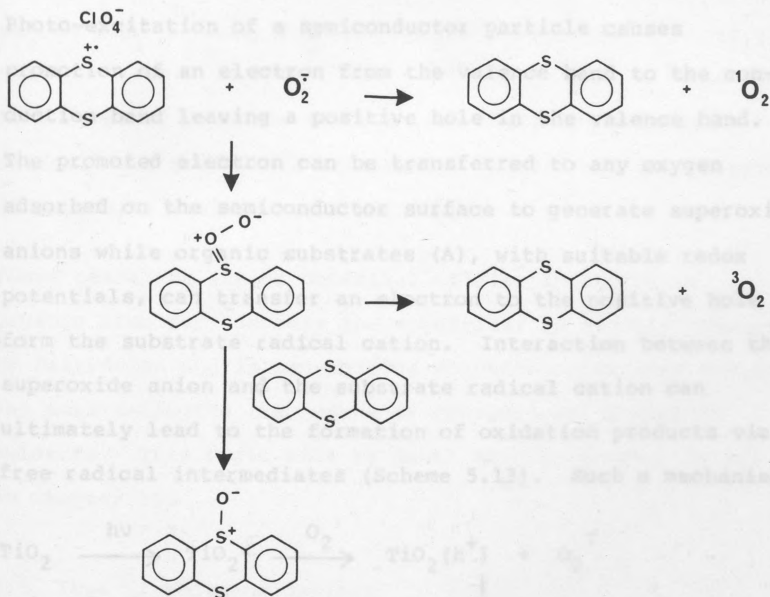
Scheme 5.12
