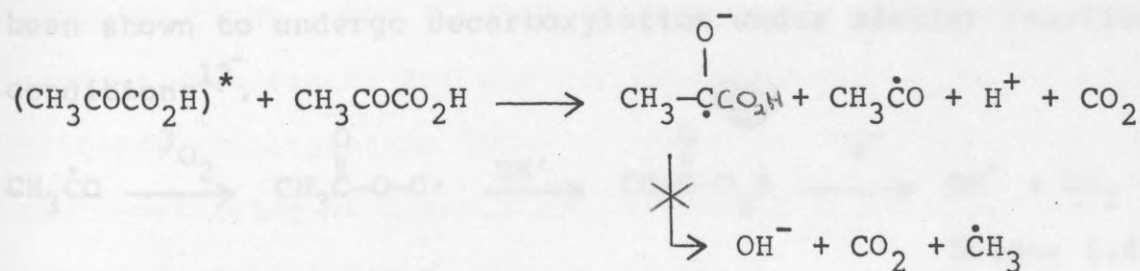
Scheme 6.4
