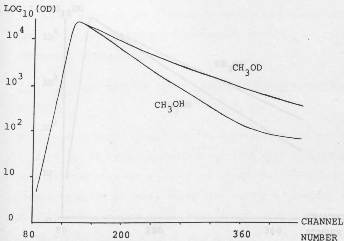
FIGURE 7.9 FLUORESCENCE DECAY CURVES FOR 1,3-DIPHENYL-2-PYRAZOLINE IN METHANOL (CH 3 OH) AND DEUTERATED METHANOL SOLUTIONS
