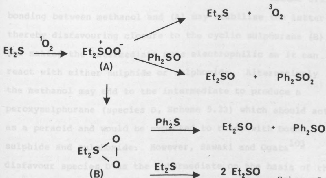
Scheme 5.22
