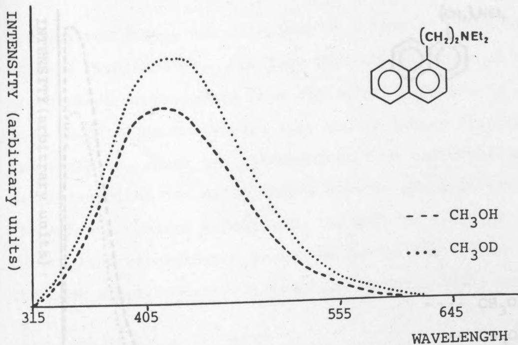
FIGURE 4.3(A) FLUORESCENCE SPECTRA OF \alpha 2E IN METHANOL ( \text{CH}_3\text{OH} ) AND DEUTERATED METHANOL ( \text{CH}_3\text{OD} ) SOLUTIONS
