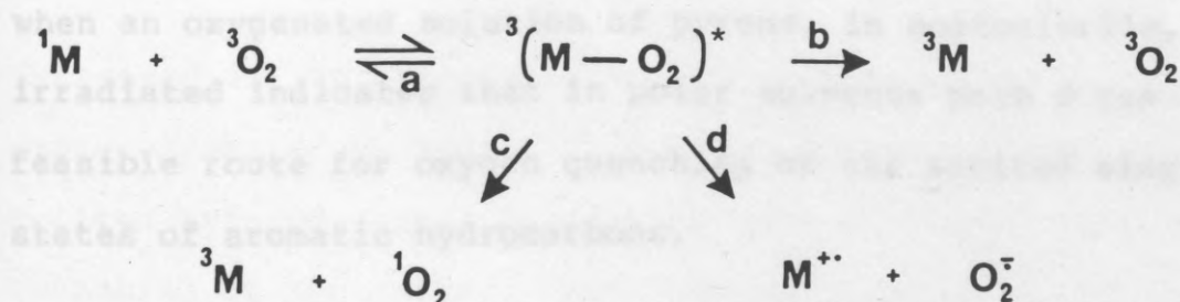
Scheme 8.1
