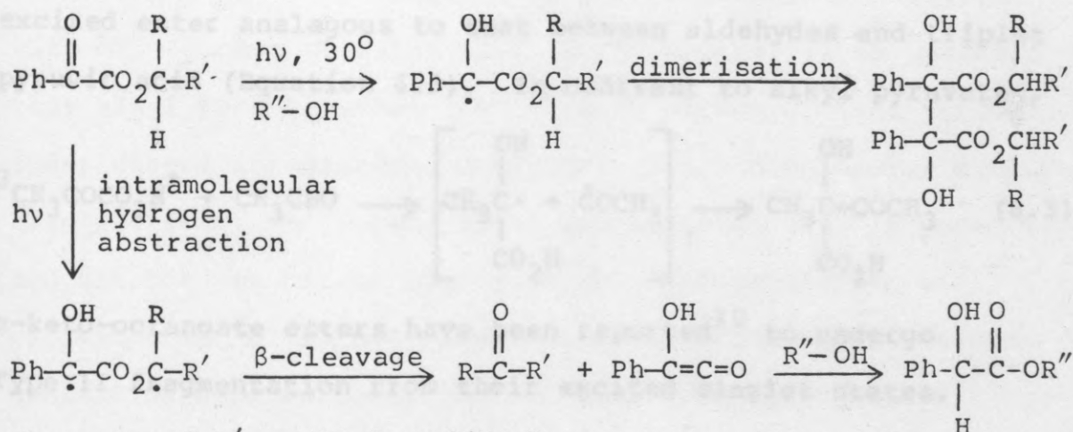
Scheme 6.13
