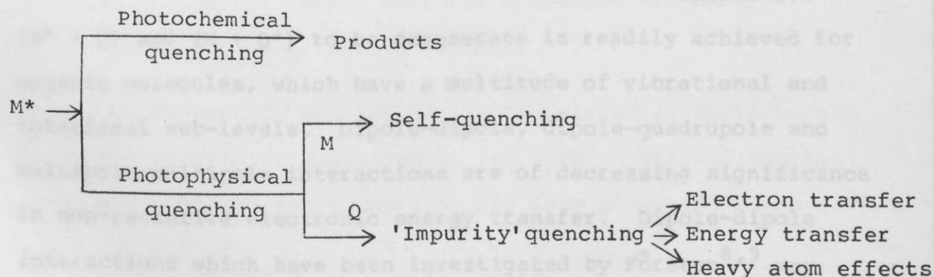
Scheme 1.1
