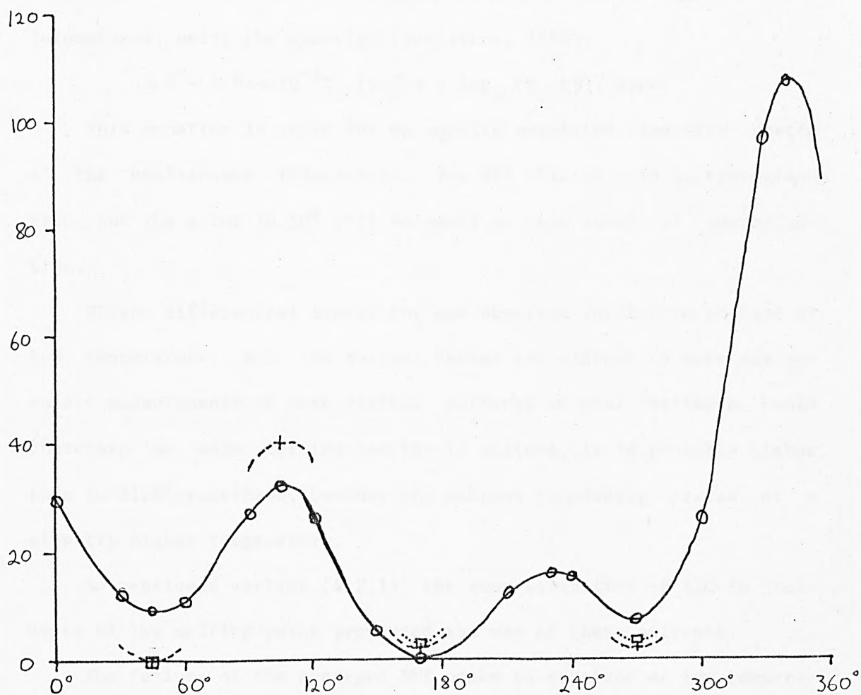
Figure 4.7. BIC potential energy surface, —○— MM2 gas-phase calculations; --+-- dichloromethane solvent; ...□... acetone solvent. The latter two are average values.
