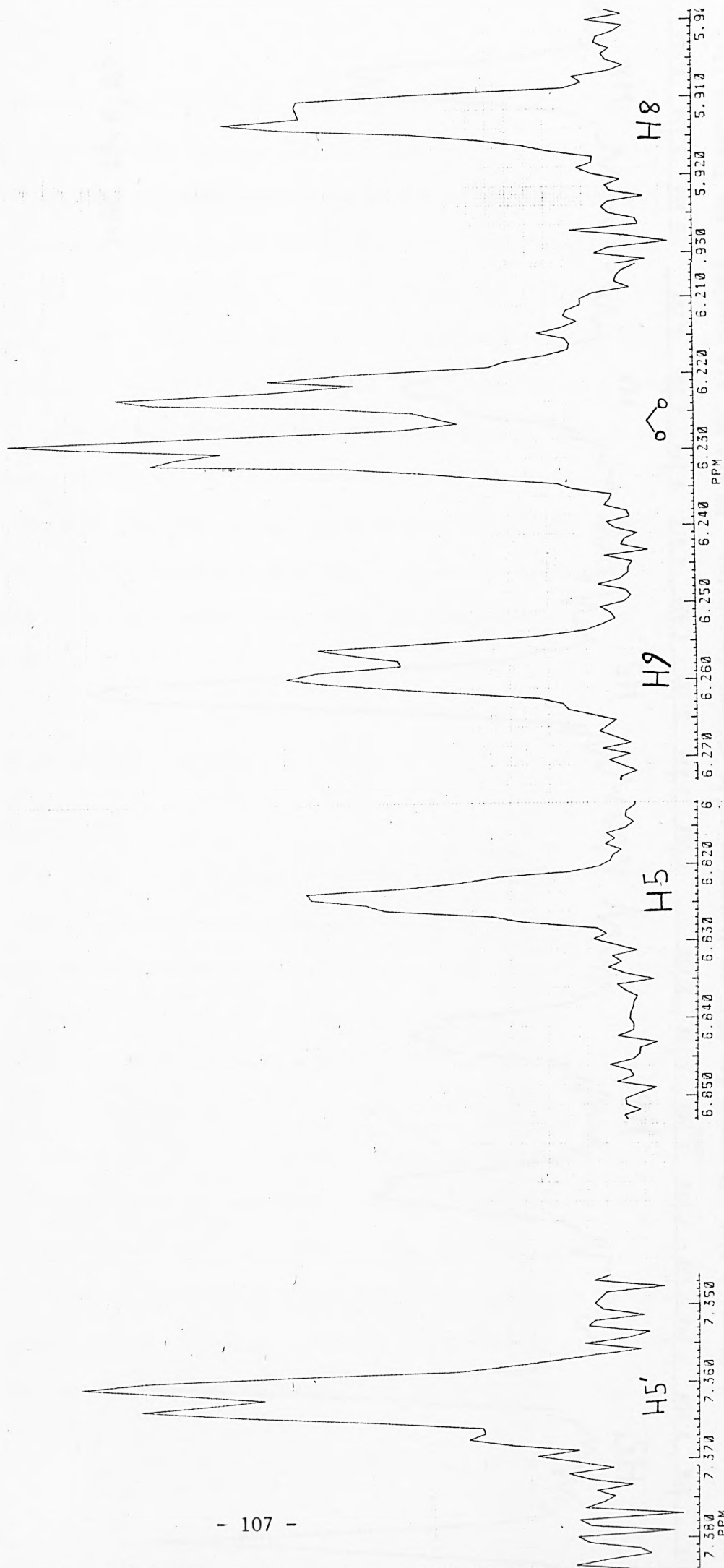
Figure 4.11a. Spin decoupling at H6' (7.16ppm) for HBIC in deuterium oxide. The apparent splitting in the H9 peak is due to noise in the spectrum (cf H5' and H8, and Figure 4.11b).
