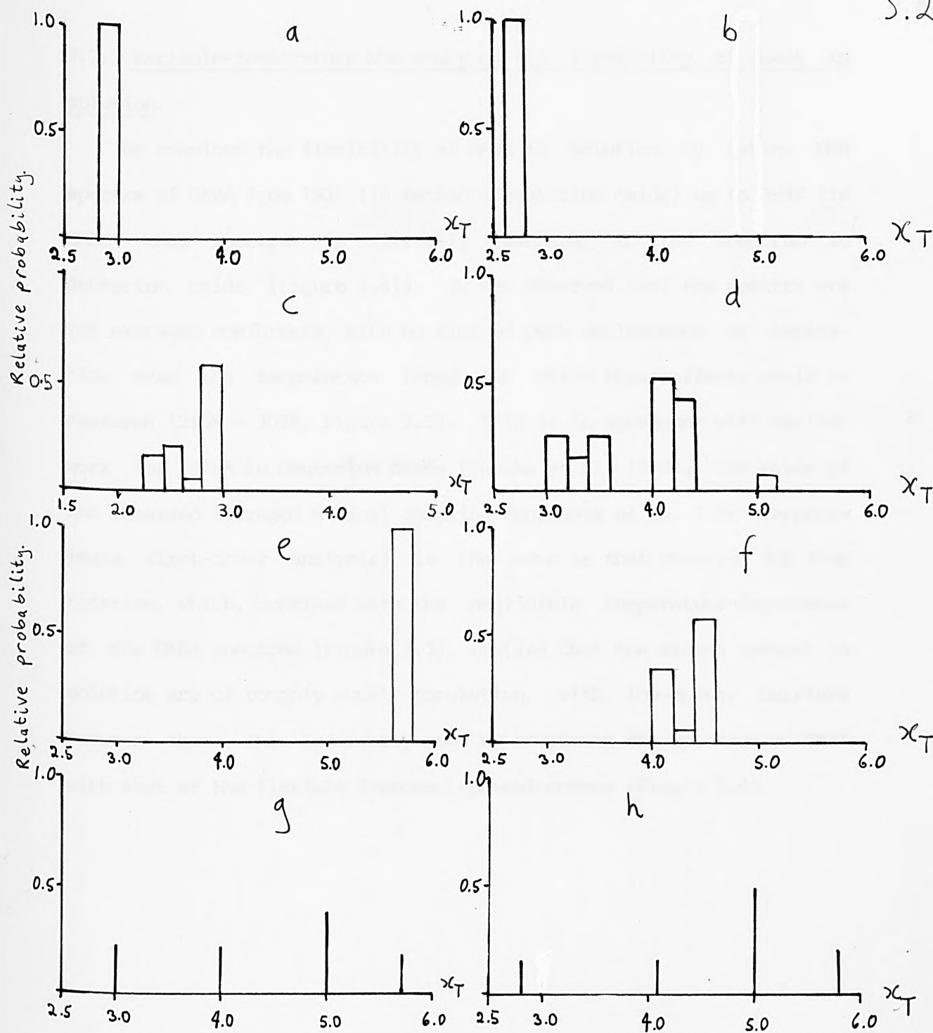
Figure 3.2. GABA x_T distributions by various methods.
