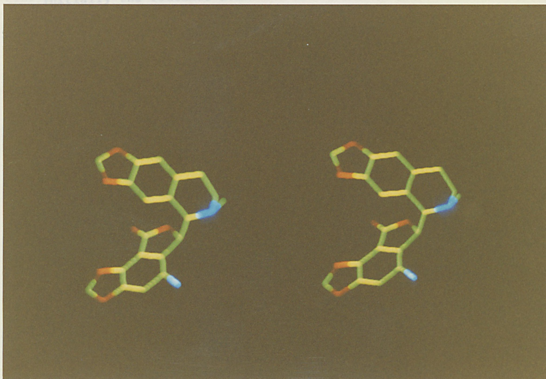
a) BIC, \theta_1=270^\circ . (The yellow colour is an artifact of the photograph.)
