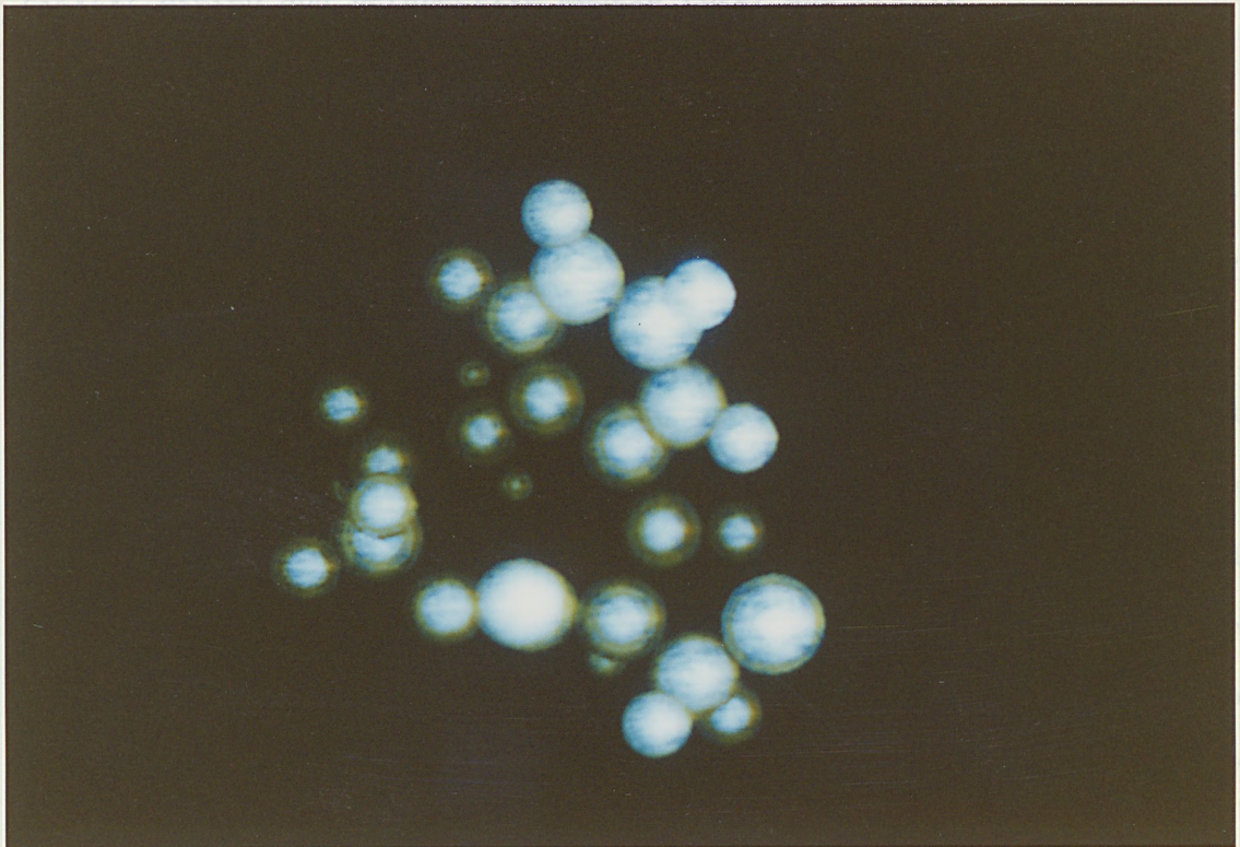
Figure 7.7. Example of space-filling model.
