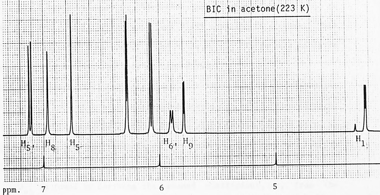
Figure 4.2 Temperature-dependence of BIC chemical shifts.
