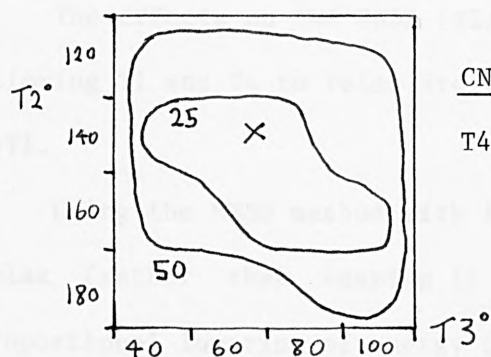
Figure 3.8. GABA SOLVEFF surfaces.
