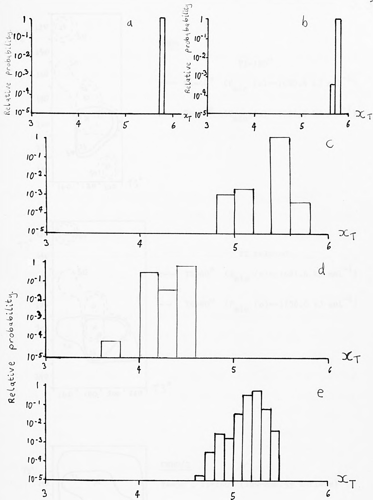
Figure 3.7. GABA x_T distributions by SOLVEFF and Hybrid methods.
