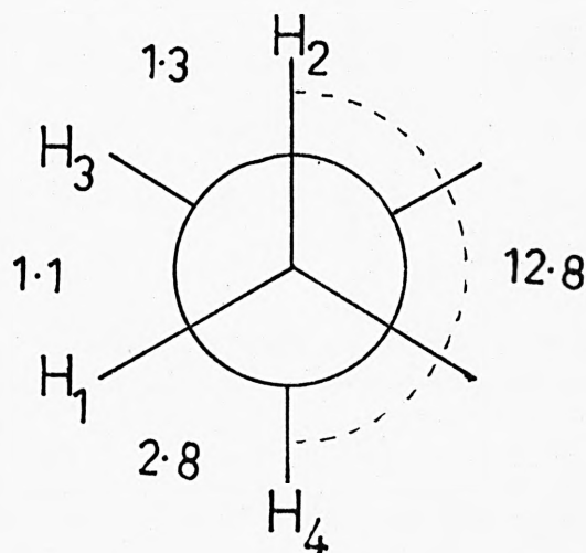
Figure 4.3. Vicinal proton coupling constants for morpholine (Hz) (Spragg, 1968).
