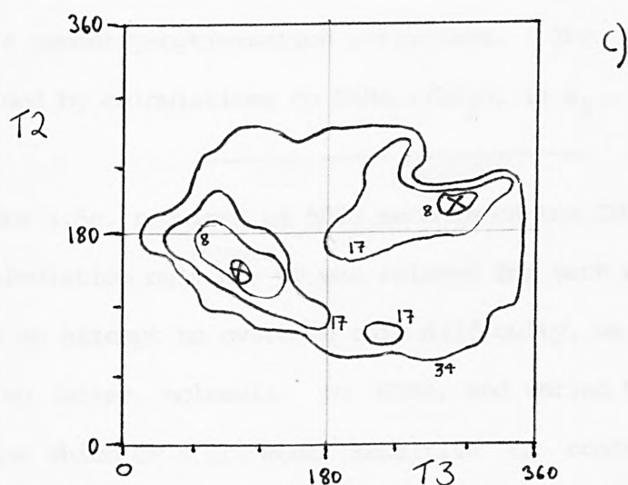
Figure 3.5 GABA Supramolecule surfaces ( \text{kJ mol}^{-1} ).
