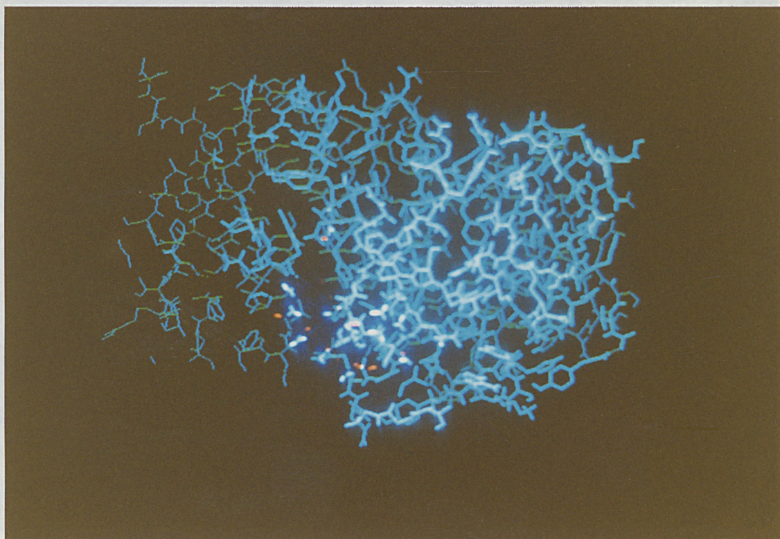
Figure 7.6. Difference between active-site and whole receptor views.
