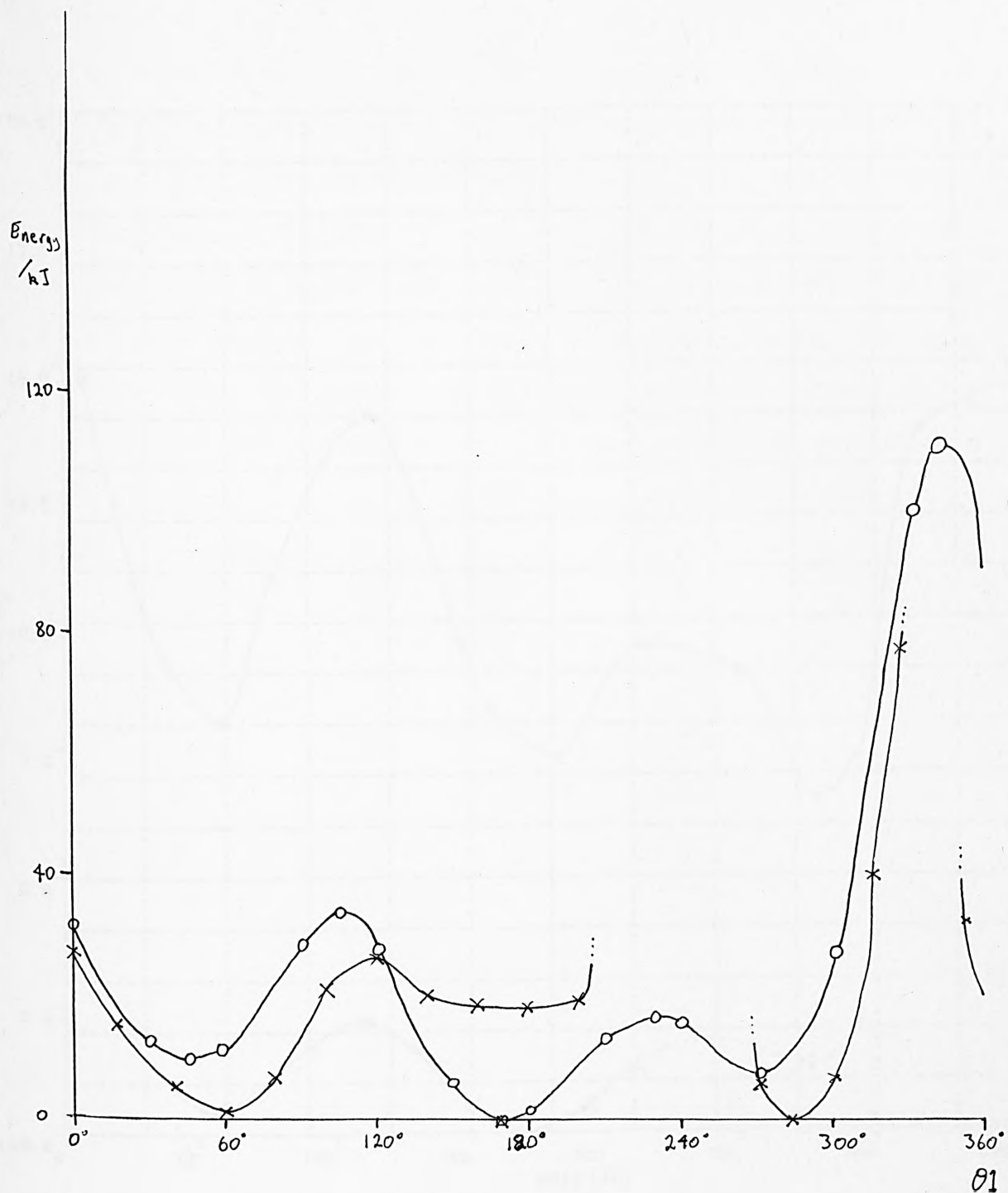
Figure 2.4 BIC and MeBIC energy-surfaces (MM2)
