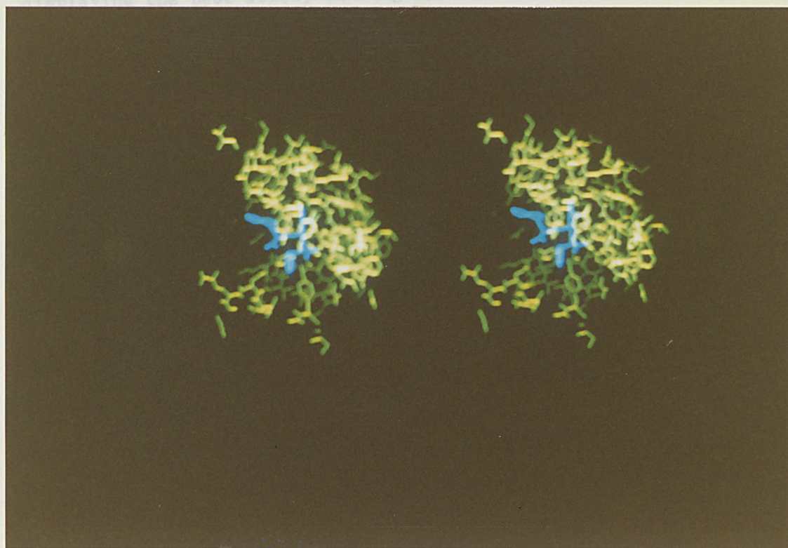
b) TLN active-site with a bound drug (CLT - see Figure 7.13).
