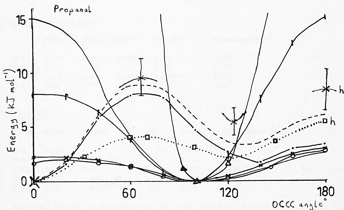
Figure 2.1. Energy surfaces calculated by various methods.
