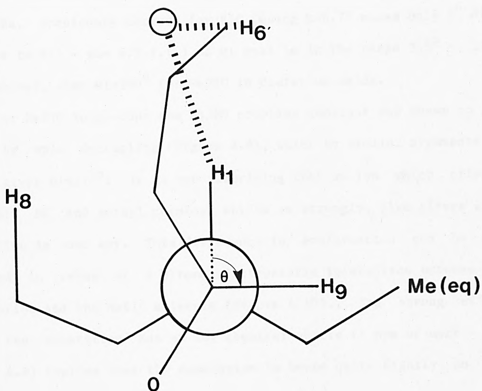
Figure 4.8 Position of the counterion in MeBIC.
