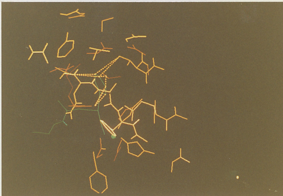
74 Figure 7.14. Close contacts around the benzene ring in BAG. The CC's shown were calculated with high sensitivity (SENS=1.0Å) and give an indication of how much room there is near a particular atom for modifying the drug. SENS can be further increased and the atoms for which no CC's are shown here further investigated.
