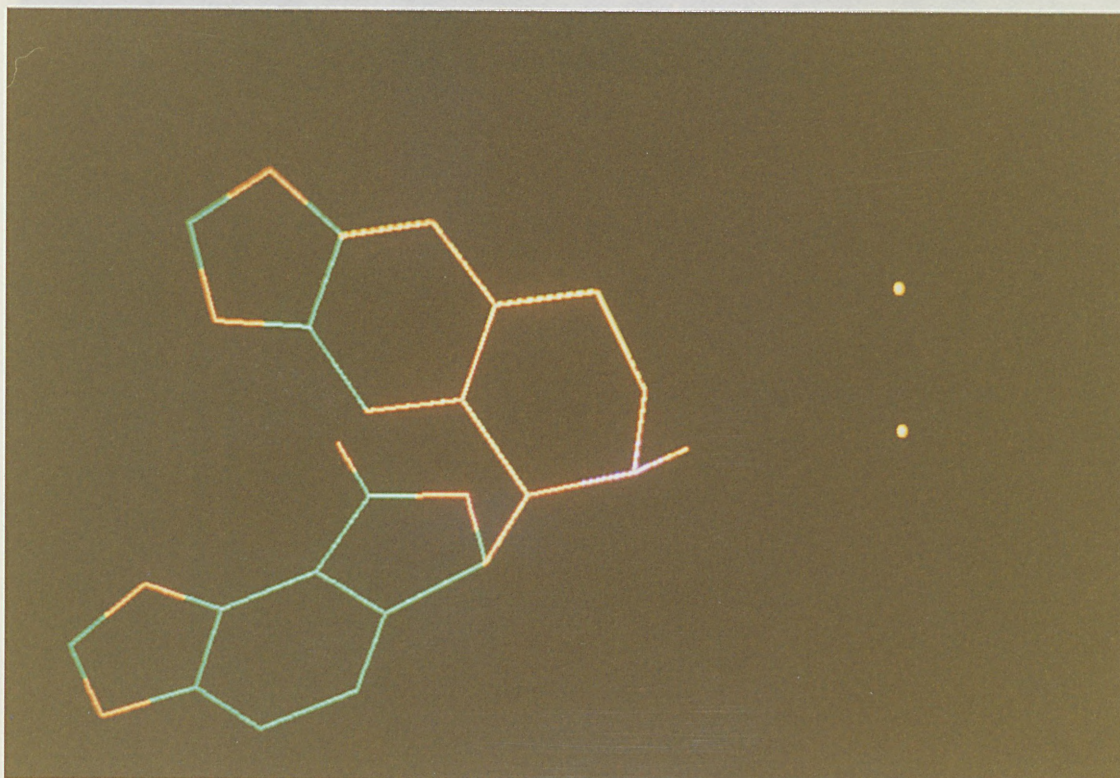
Figure 7.9a. Example of molecular fragment deletion (ED6). (see Figure 7.9b). The two pictures below show 2 paths between C5 and C8 in BIC chosen by IMDAC for possible fragment. The latter fragment was subsequently deleted (see Figure 7.9b).
