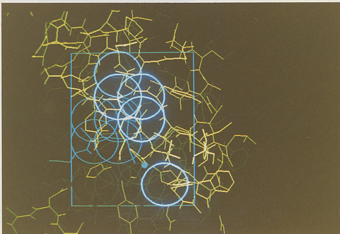
Figure 7.3. Examples of the use of the CLEFT option (OP33).
