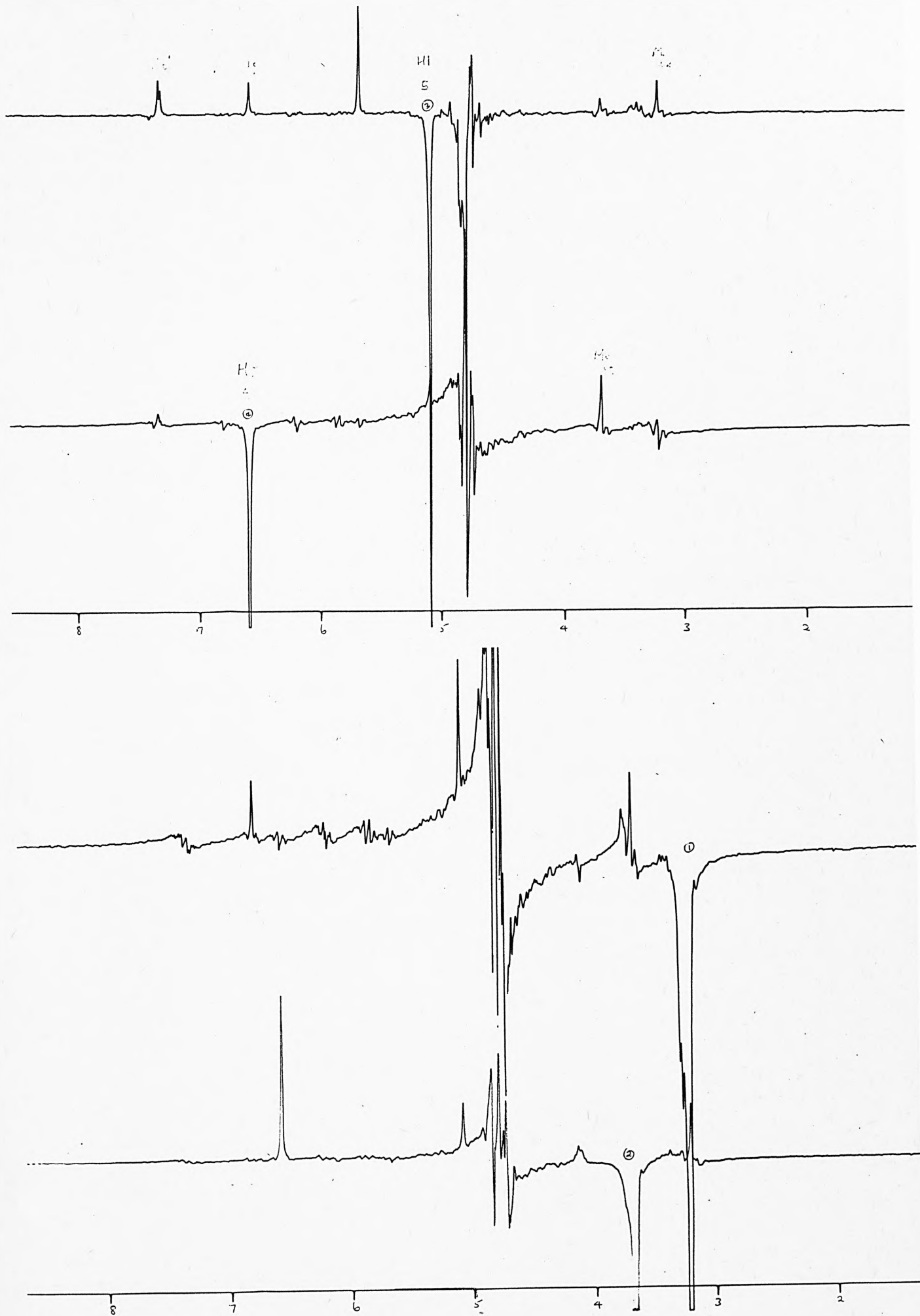
Figure A2.9. MeBIC(I) NOE effects ( D_2O ).
