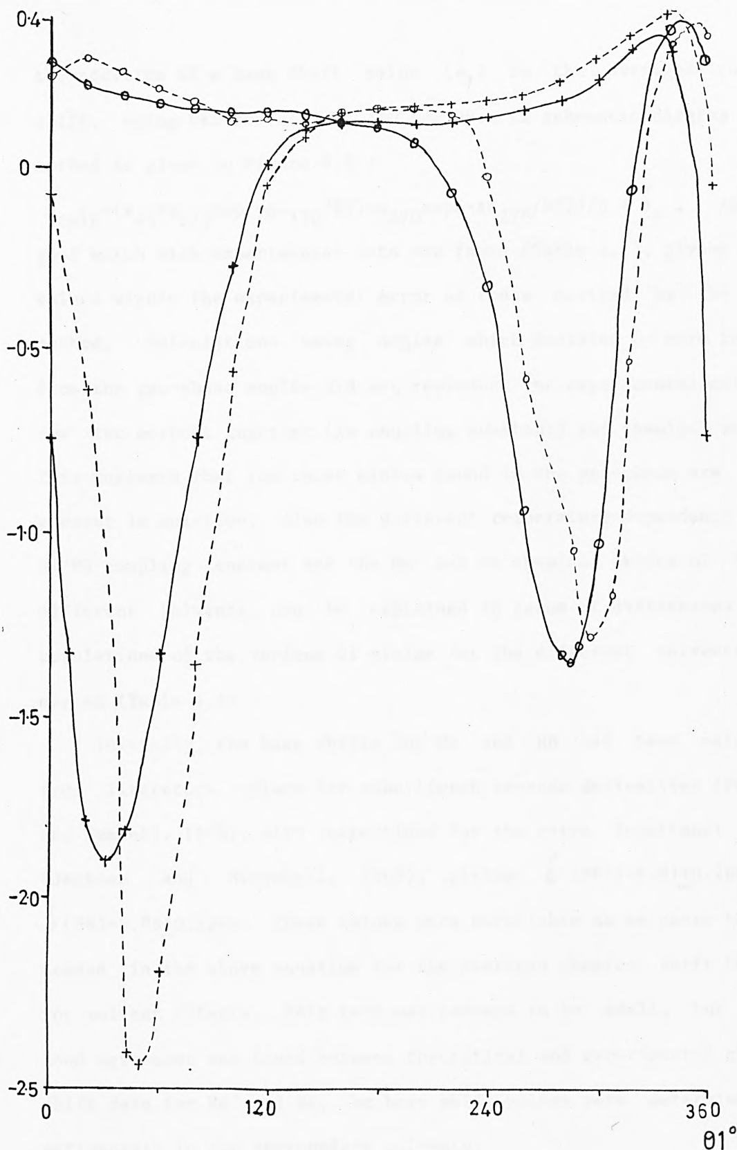
Figure 4.5. Theoretical shielding contribution for H6' and H8 in BIC. Two of the proposed solution angles are in regions of extreme shielding, which would account for the large temperature-dependence of the chemical shifts of these protons. (The third angle ( \theta_1 \approx 170^\circ ) is important in the coupling constant calculations, because of the large coupling for this angle.) (+)H6'; (o)H8; solid lines MM2 geometry; dashed lines crystal geometry.
