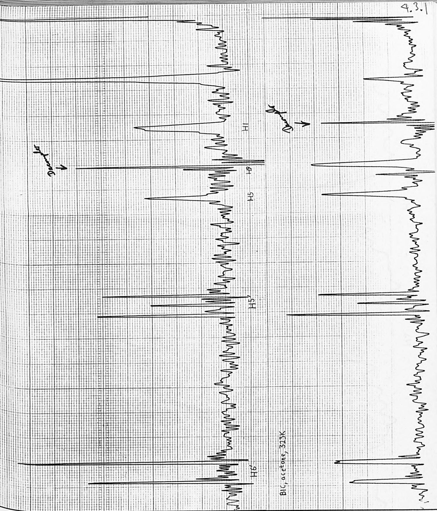
Figure 4.9. Spin decoupling on H1 and H9 for MeBIC in acetone.
