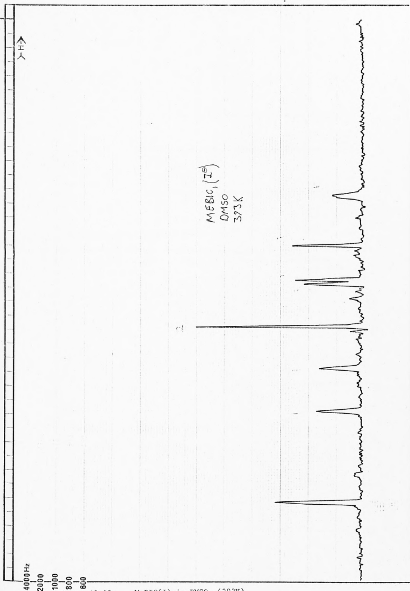
Figure A2.10a. MeBIC(I) in DMSO (393K)
