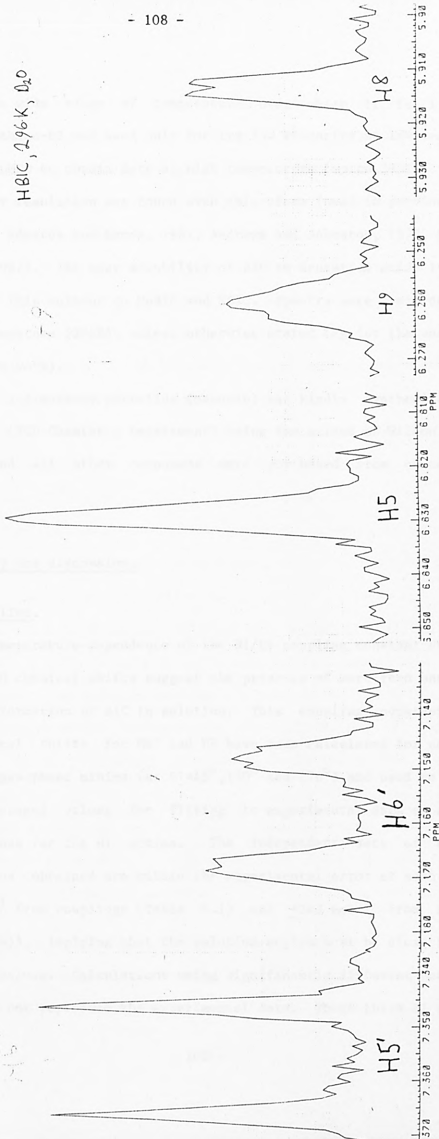
Figure 4.11b. Spectrum for HBIC in deuterium oxide without decoupling. H9 and H6' are coupled (see Figure 4.11a).
