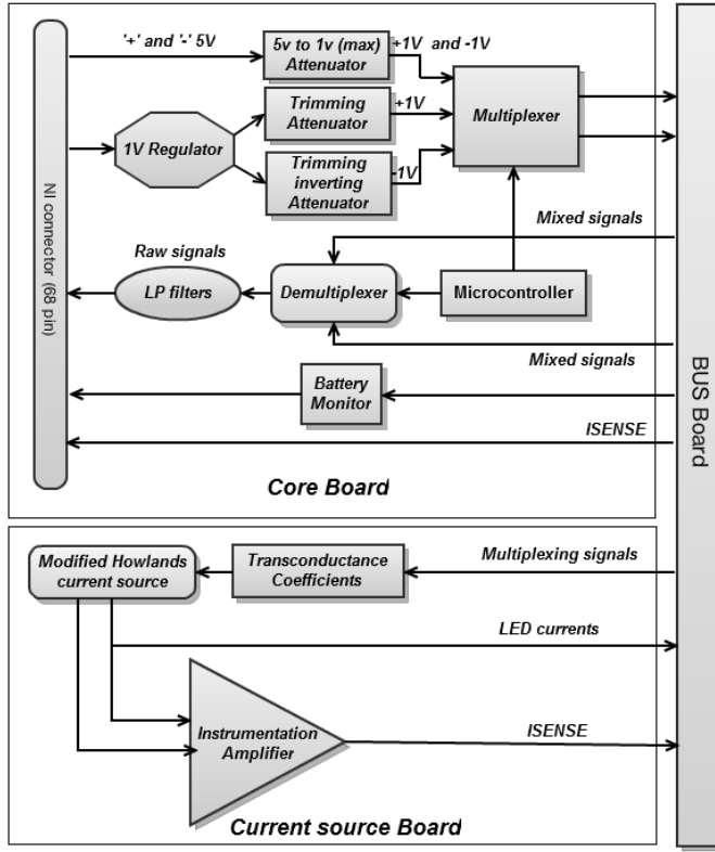
Figure 2. Flow diagram demonstrating the function of Core and current source modules
