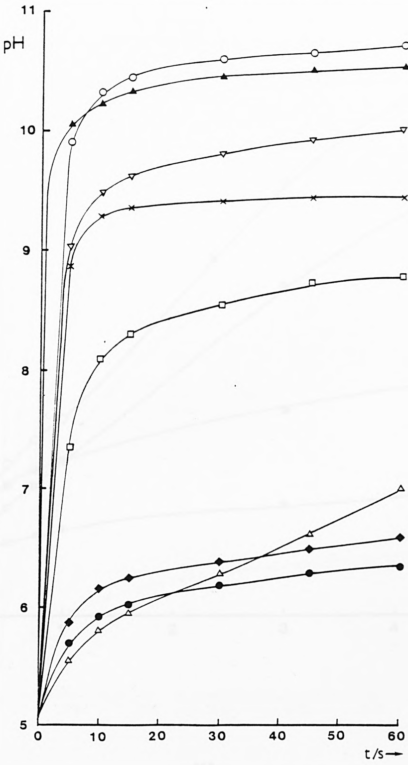
Figure 5.40 Kinetic pH responses of sodium and calcium forms of synthetic zeolites of different framework density after immersion in distilled water. Data for (○) NaA; (▲) NaZ1; (▽) NaZ2; (×) NaZ3; (□) NaZ4; (◆) NaZ5; (△) CaA; (●) CaX
