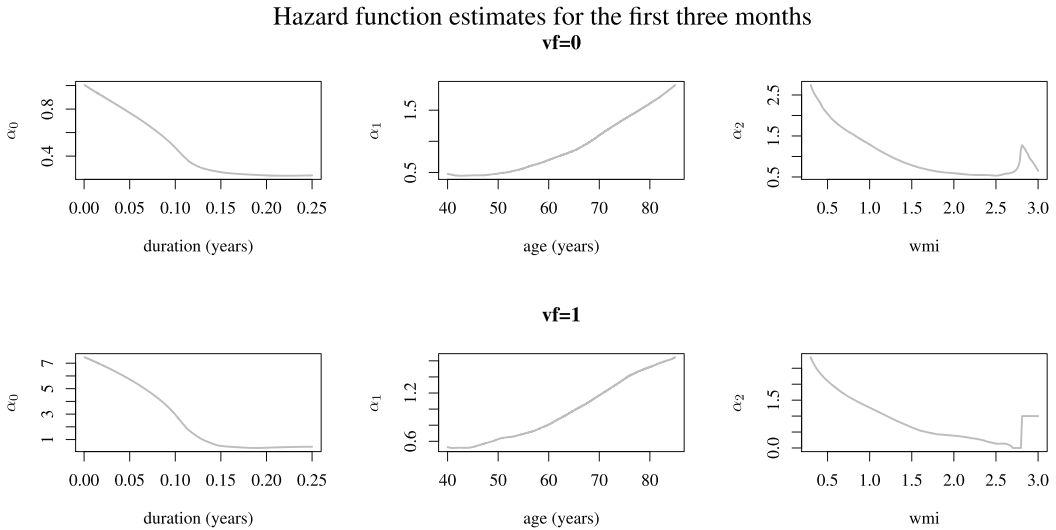
FIGURE B1 Local constant multiplicative smooth backfitting fit of (\alpha_0, \alpha_1, \alpha_2) conditional on surviving the first three months for two different strata depending on the value of \mathbf{vf} .
