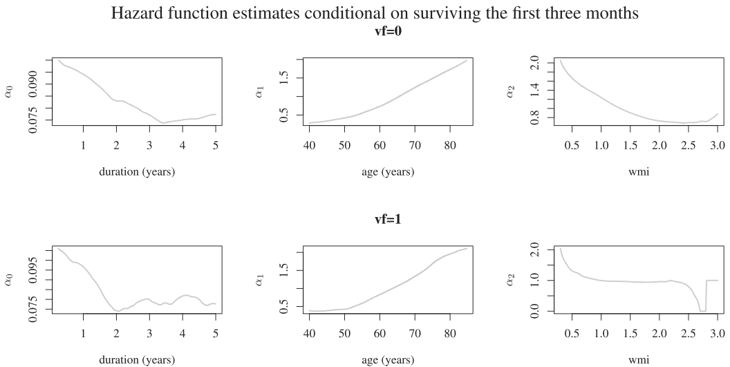
FIGURE B2 Local constant multiplicative smooth backfitting fit of (\alpha_0, \alpha_1, \alpha_2) conditional on surviving the first three months for two different strata depending on the value of \mathbf{vf} .
