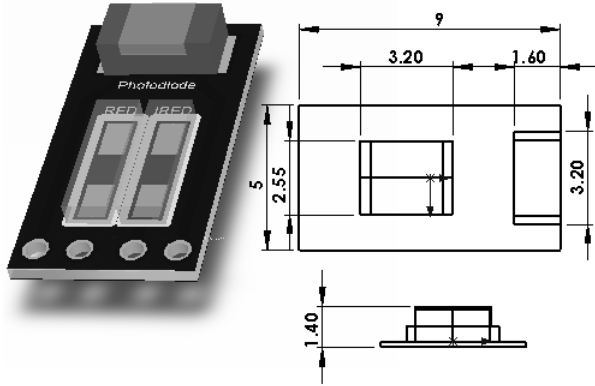
Fig. 1. Optoelectronic reflectance sensor used in the ear canal PPG/pulse oximeter probe showing the emitters and photodetector.
