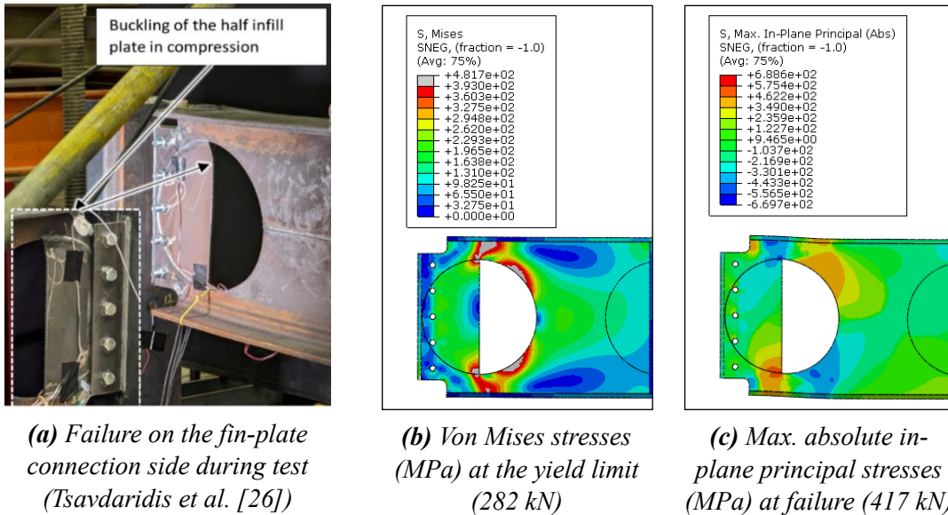
Figure 10: First failure at a shear force of 417 kN on the fin-plate connection side (Test 3)
