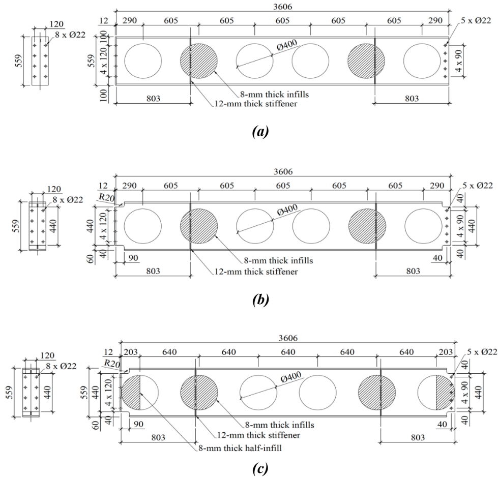
Figure 1: Details of cellular beams in the tests: (a) narrow end-post, (b) narrow end-post with notches, (c) half infill plate end-posts with notches (Tsavdaridis et al. [26])
