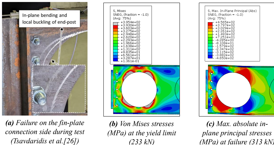
Figure 4: First failure at the shear force of 313 kN on the fin-plate connection side (Test 1)
