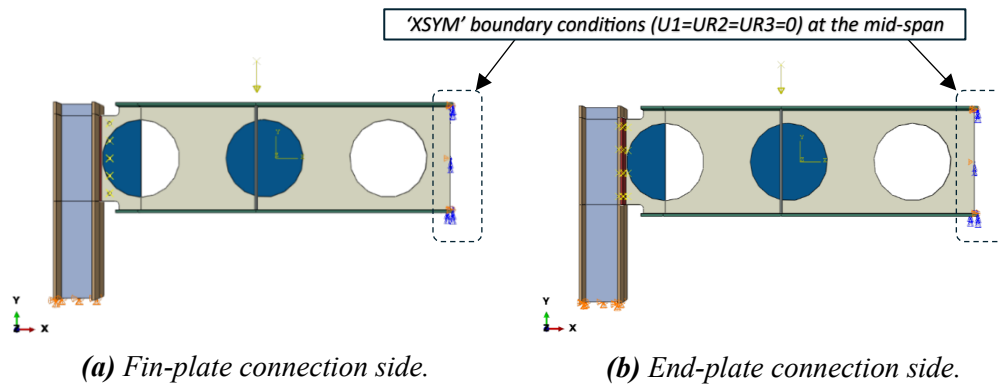
Figure 12: Isolated models for Case 3.
