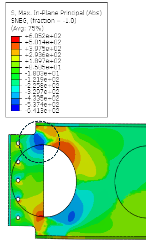
Figure 15: Max. absolute in-plane principal stresses (MPa) when buckling of the half infill plate occurred in the model with the widest notch ( h_o = 350\text{mm} and c_n = 135\text{mm} ).
