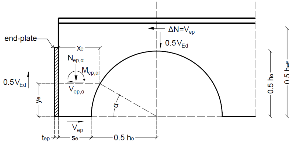
Figure A.3: Moment acting on the horizontal plane of a narrow end-post with an end-plate connection.
