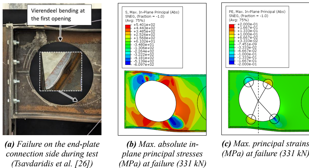
Figure 5: Second failure at the shear force of 331 kN on the end-plate connection side (Test 1)
