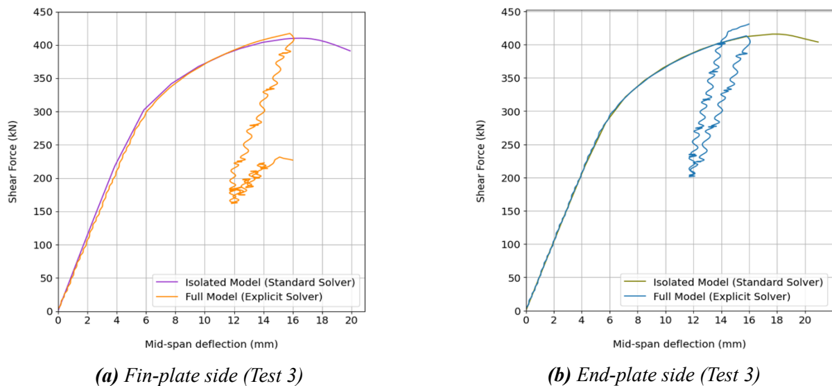
Figure 13: Shear force vs. mid-span vertical displacement curves for the models for beams with half infill plates next to the connections (Test 3).
