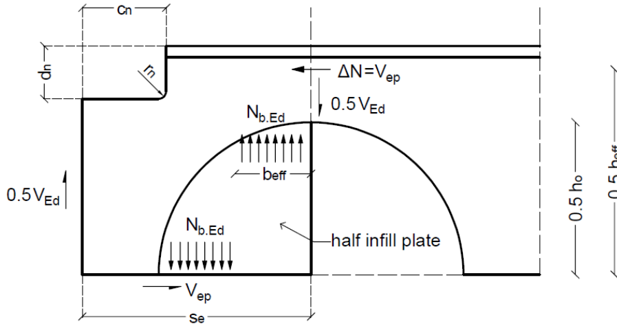
Figure A.6: Forces in end-post formed by a half infill plate.
