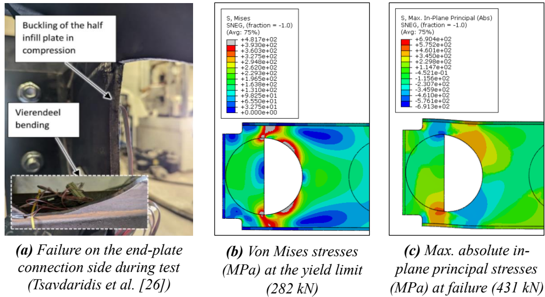
Figure 11: Second failure at a shear force of 431 kN on the end-plate connection side (Test 3)
