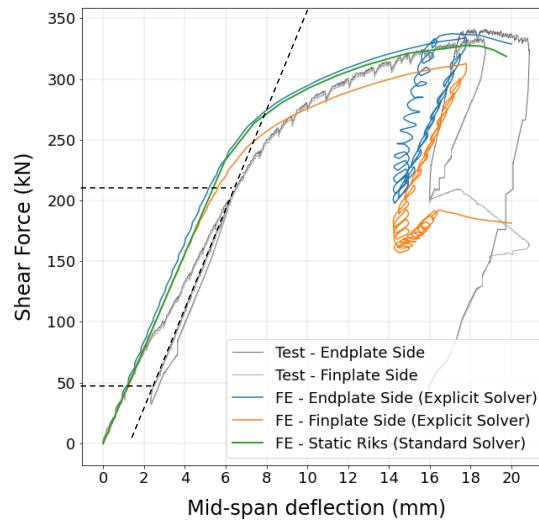
Figure 3: Shear force vs. Mid-span vertical deflection curve (Test 1)
