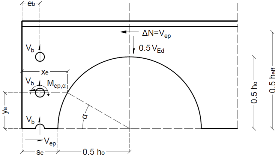
Figure A.1: Illustration of horizontal shear and bending in a narrow end-post.
