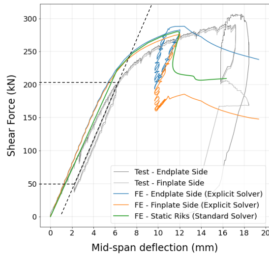
Figure 6: Shear force vs. Mid-span vertical deflection curve (Test 2)
