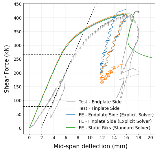
Figure 9: Shear force vs. Mid-span vertical deflection curve (Test 3)
