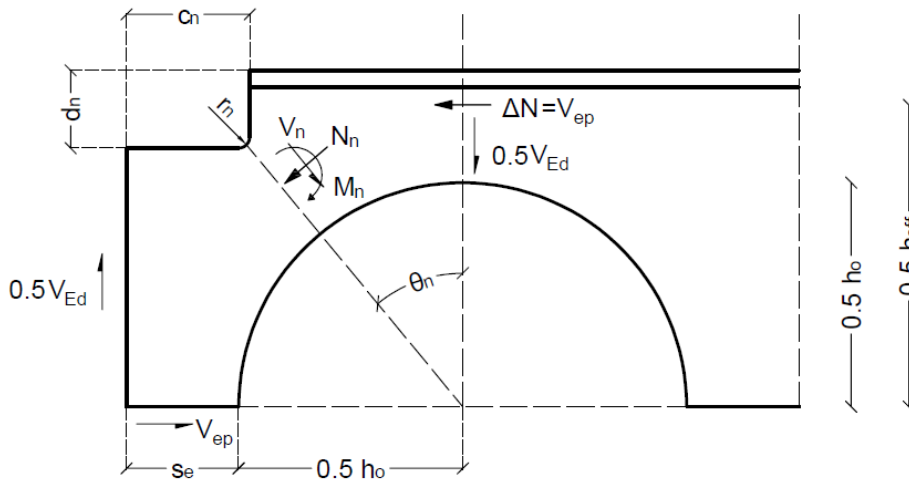
Figure A.5: Forces on the notched end-post at the centre-line of the first opening.
