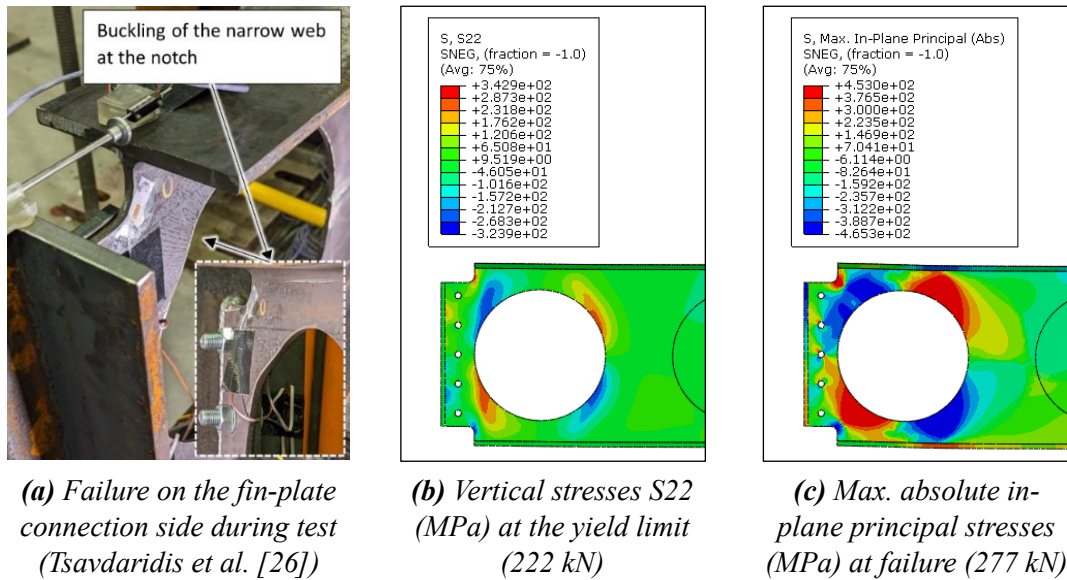
Figure 7: First failure at the shear force of 277 kN on the fin-plate connection side (Test 2)
