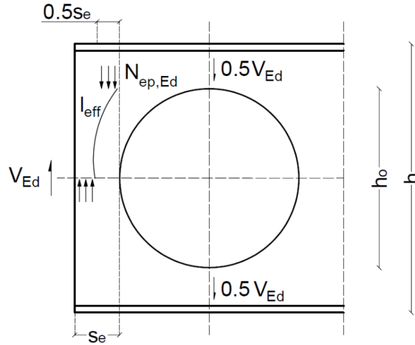
Figure A.2: Illustration of strut buckling model for an end-post in BS EN 1993-1-13 [9].
