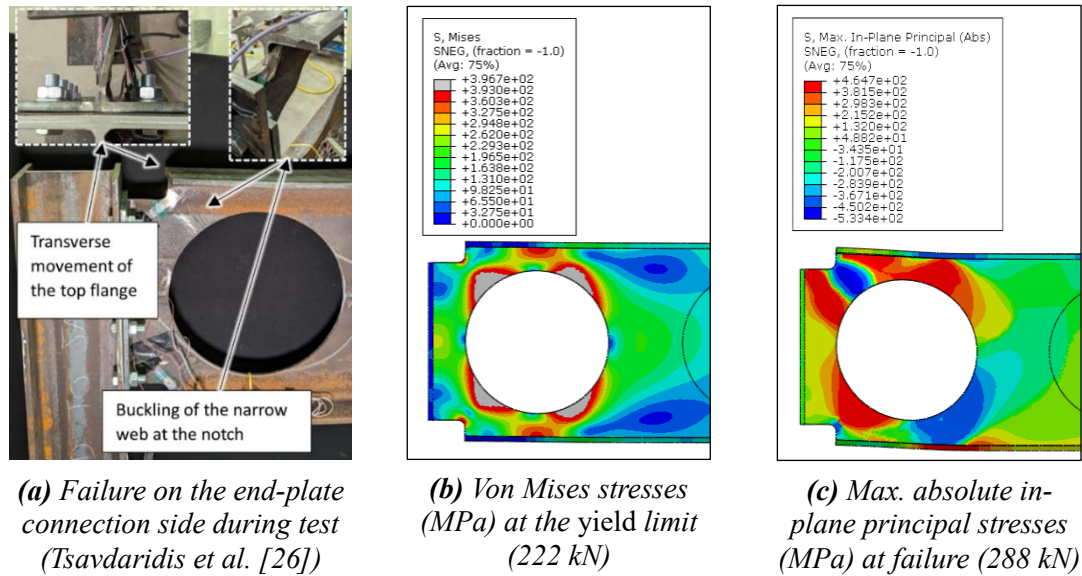
Figure 8: Second failure at the shear force of 288 kN on the end-plate connection side (Test 2)
