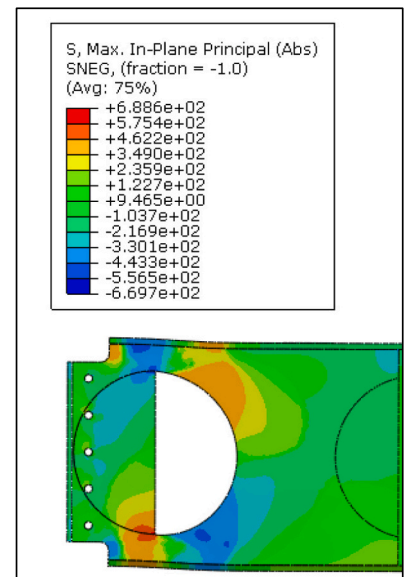
(c) Max. absolute in-plane principal stresses (MPa) at failure (417 kN)
