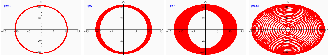
Figure 6: Classical trajectories from (4.3)-(4.6) in the (x, p_x) phase space in regime I with \Omega = -1 , \nu = 4 .
