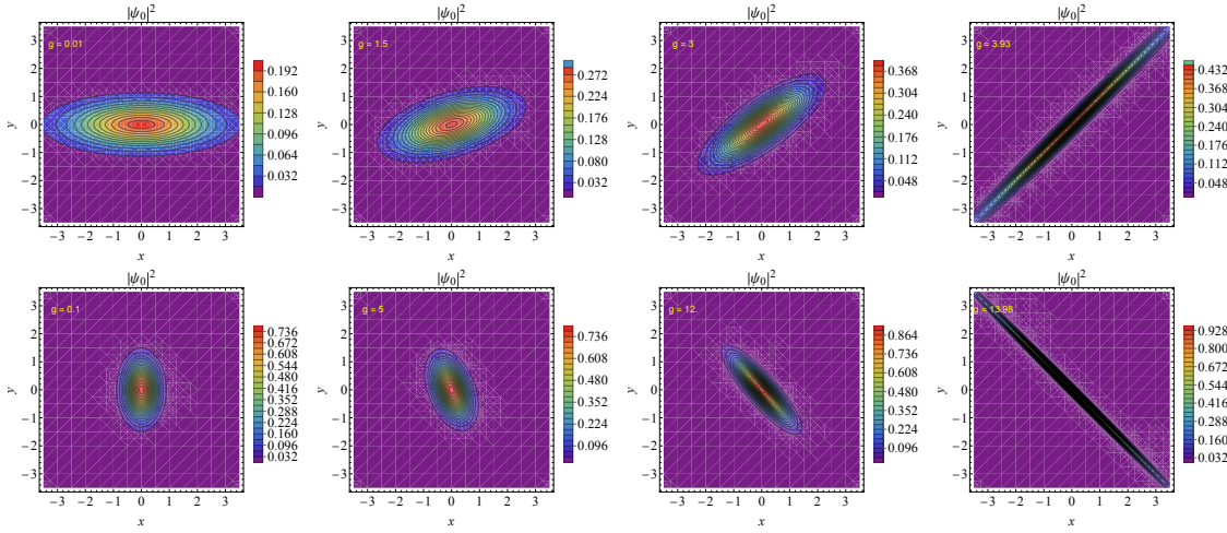
Figure 3: Probability densities for the “ground state” for different coupling constants g for the \epsilon = \eta = -1 branch with \nu = 4 , \Omega = -2 in the upper row and \epsilon = -\eta = -1 branch with \nu = 0.2 , \Omega = -4 in the lower row.
