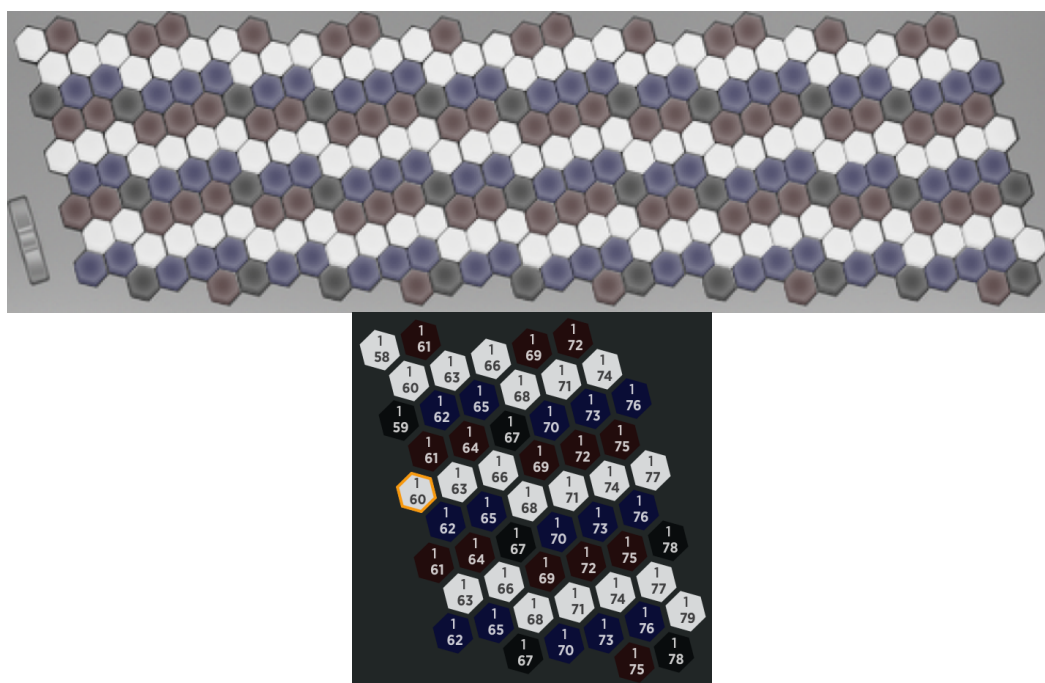
Figure 9. Bosanquet-Wilson mapping of 19EDO, a Diatonic EDO according to Giedraitis, a negative EDO according both to Barbour and Bosanquet, and close to 1/3 -Comma Meantone Temperament. This mapping is a literal representation of Figure 7. Sharp notes (in dark red, diagonally right/up from a white ‘natural key’) are lower than what would otherwise be their flat enharmonic equivalents (in dark blue, diagonally left/down from a white ‘natural’ key), with the exception of the E#/Fb and B#/Cb pairs, which are enharmonic (by being represented by the same black key, similarly to the black keys of the 12EDO piano). Consequently, a diatonic semitone (2 steps) is wider than a chromatic semitone (1 step). Middle C is mapped as MIDI note 60.
