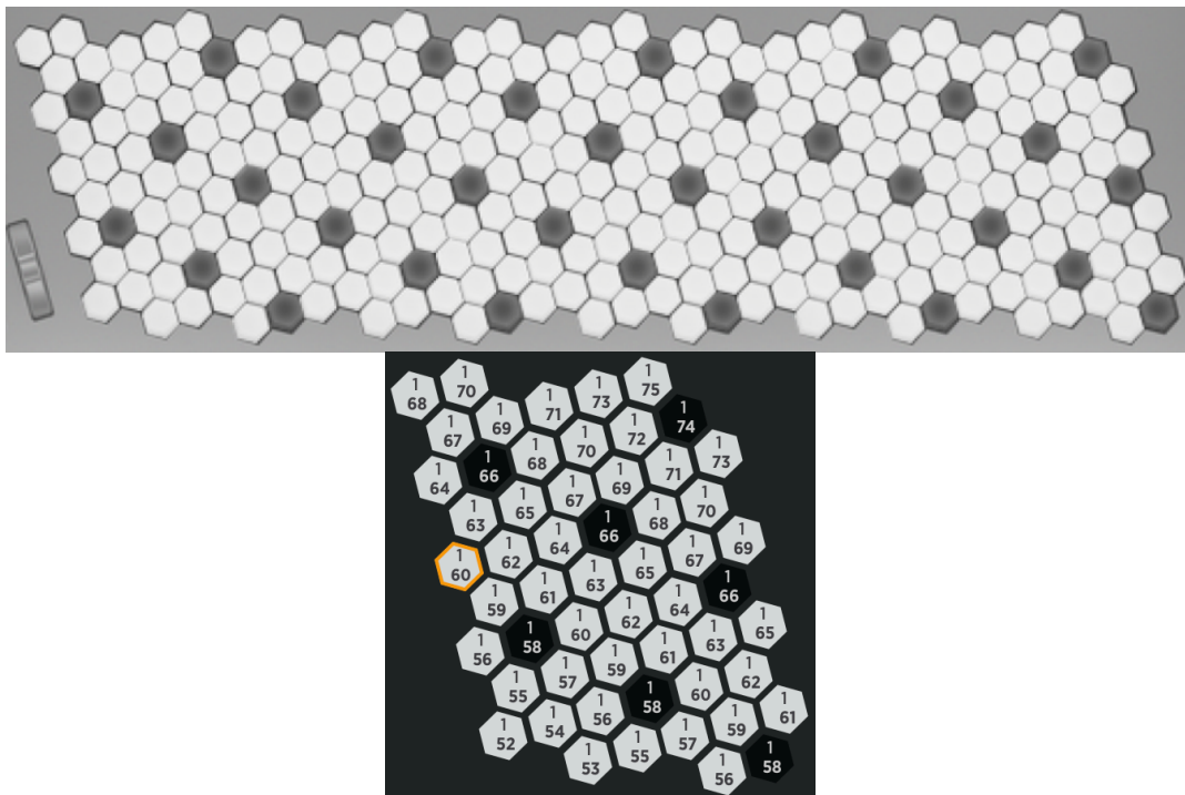
Figure 89. Bosanquet-Wilson mapping of 8EDO, a Supersharp EDO according to Giedraitis.
