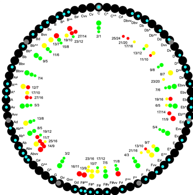
Figure 35. A representation of 7EDO (grey dots) and 72NPO (black dots and notation) against Sabat and Haywards's tuneable intervals.
