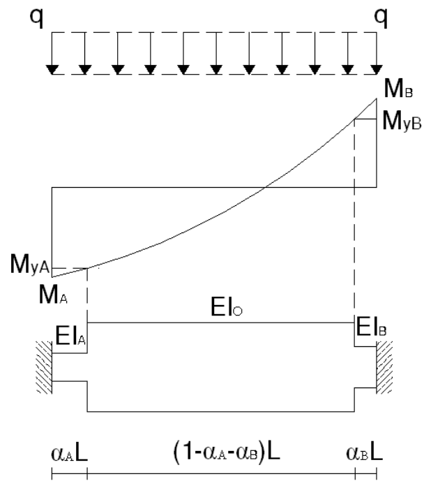
Figure 1: Flexural sub-element
