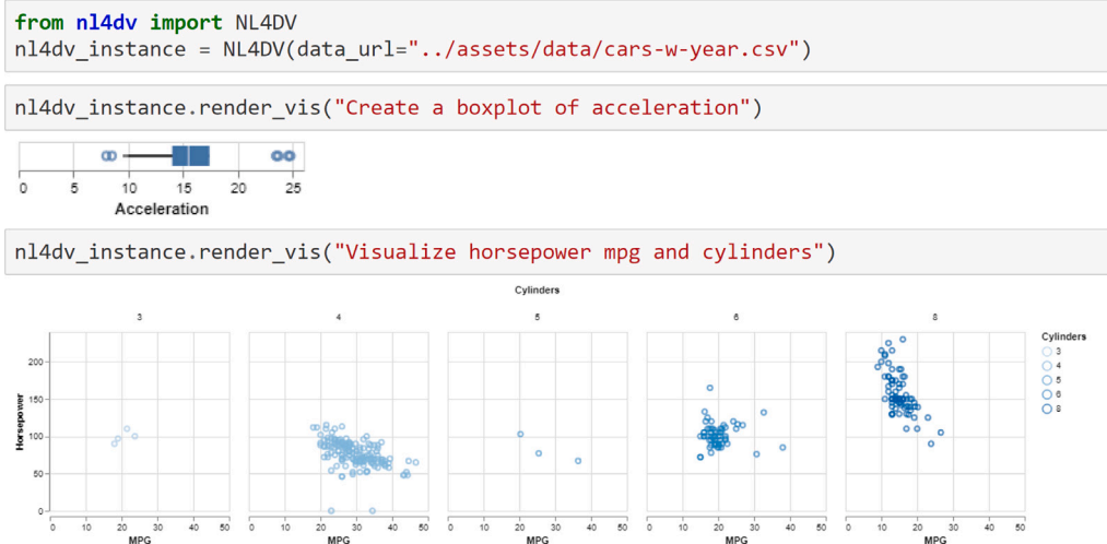
Fig. 3. A demonstration of the rule-based V-NLI NL4DV integrated within a Jupyter Notebook, enabling users to generate visualisations by specifying natural language instructions in Python. Image from Narechania et al. [23].
