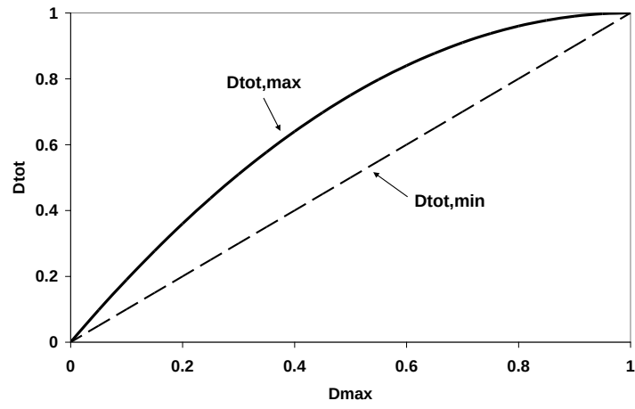
Fig 7 Variation of D_{\text{tot}} with D_{\text{max}} , for D_{\text{min}}=0 or D_{\text{max}}
