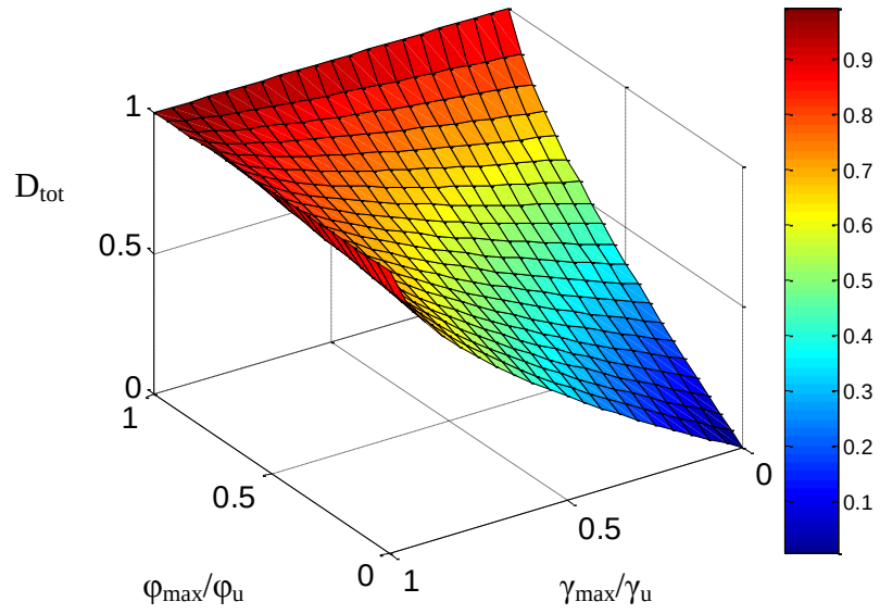
Fig 11 Variation of D_{\text{tot}} for the various combinations of \phi_{\text{max}}/\phi_u and \gamma_{\text{max}}/\gamma_u
