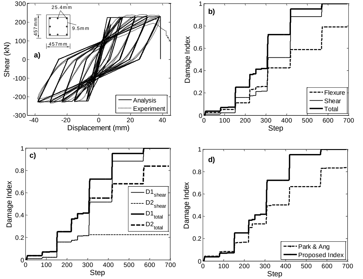
Fig 13 Lynn et al. (1996) specimen 2CLH18: (a) Lateral load vs. total displacement; (b) Variation of D_{tot} , D_{fl} and D_{sh} with the experimental load step; (c) Influence of the inelastic shear-flexure interaction effect on D_{sh} and D_{tot} ; (d) Comparison of the proposed index D_{tot} with the Park-Ang seismic damage index.
