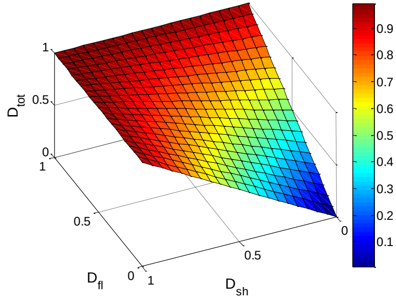
Fig 6 Variation of D_{\text{tot}} for the various combinations of D_{\text{fl}} and D_{\text{sh}}
