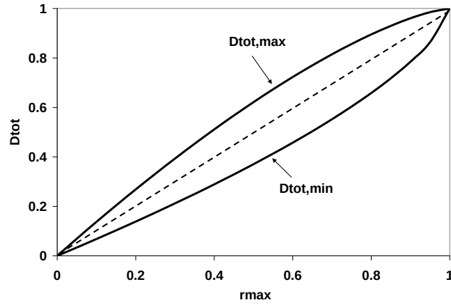
Fig 10 Variation of D_{\text{tot}} with r_{\text{max}} for \xi=2/3
