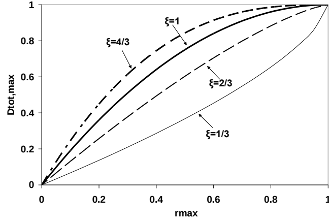
Fig 9 Variation of D_{\text{tot,max}} with r_{\text{max}}
