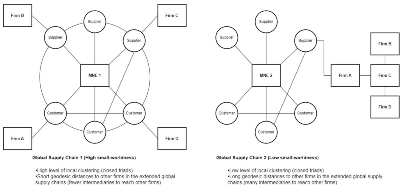
Fig. 1 MNE small-worldness
