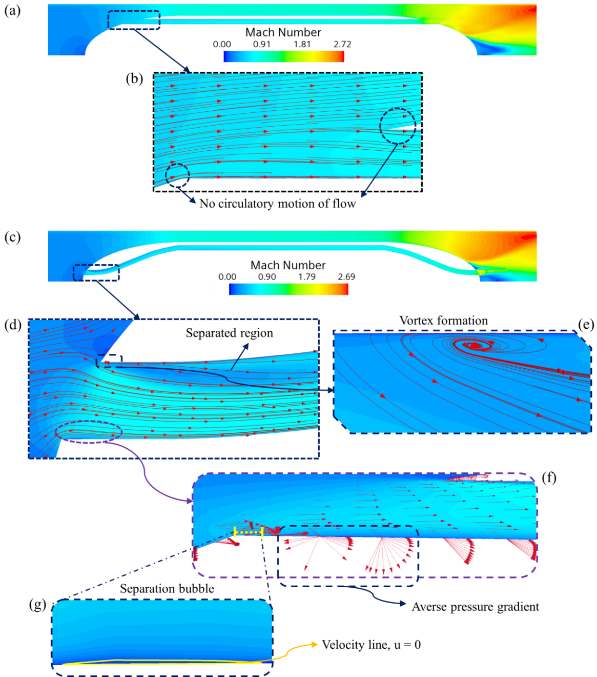
581 Fig. 14. Comparison of the flow structure within the top VD at Ma = 0.6 for DS type 1 and 4. (a) Mach distribution around 582 design 6.1. (b) Streamlines at the VD's inlet showing no circulation occurred at the entrance. (c) Mach distribution around 583 design 6.4. (d) Illustration of separated regions and streamlines at VD's inlet. (e) Magnified view of the rectangular box on 584 VD's upper wall at the vicinity of the duct inlet displaying vortex formation by drawing streamlines. (f) Magnified view of the 585 oval box on VD's lower wall showing the change in velocity vectors direction du to adverse pressure gradient. (g) 586 Demonstration of separation bubble by drawing the velocity line ( u = 0 ). Model configurations are labeled as referenced in 587 Table 2.
