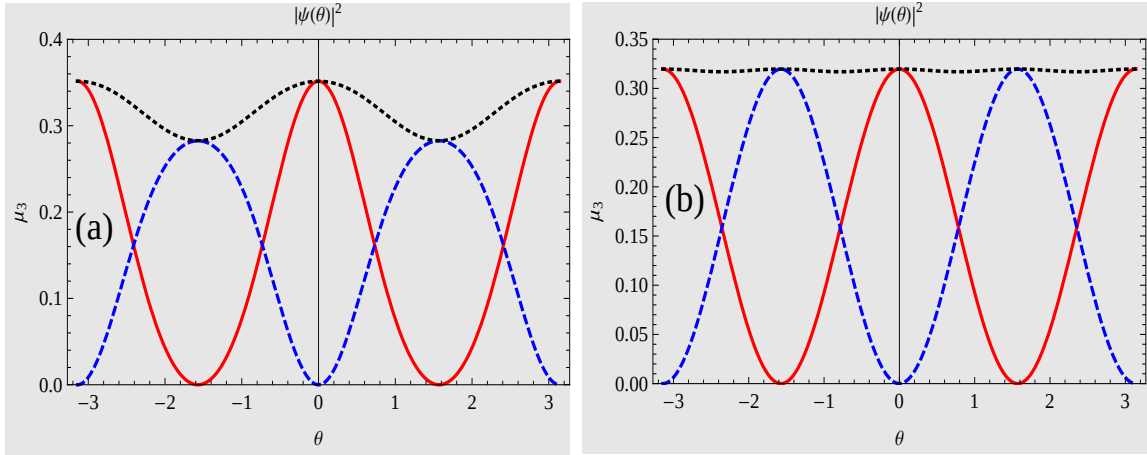
Figure 4: Intensities for a merging an even (red, solid) and odd (blue, dashed) wavefunction together with their sum (black, dotted) in the unbroken with \mu_3 = 0.8 , \mu_4 = 1 , \mu_7 = 4 and broken \mathcal{PT} -regime with \mu_3 = 1.2 , \mu_4 = 1 , \mu_7 = 4 , panel (a) and (b), respectively.
