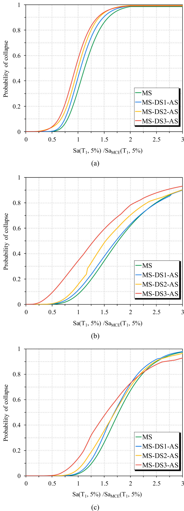
Fig. 14. the results of fragility curves for different MS-AS scenarios: (a) 4-story (b) 8-story (c) 12-story.
