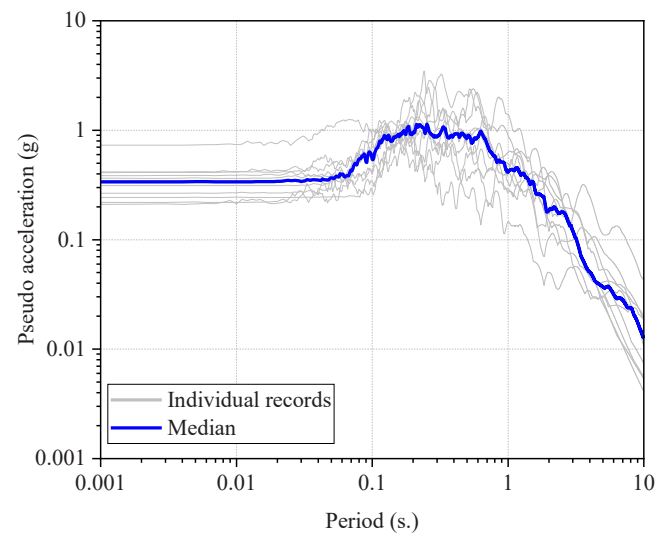
Fig. 2. Acceleration response spectra of the selected ground motion records.
