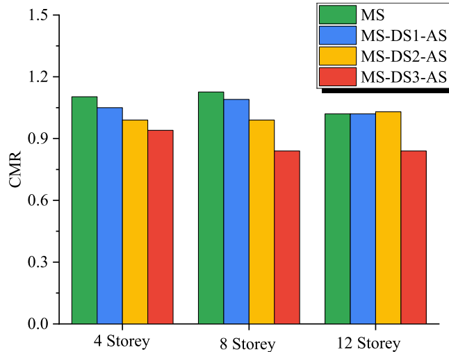
Fig. 15. The values of collapse margin ratio for only MS and MS-AS scenarios.
