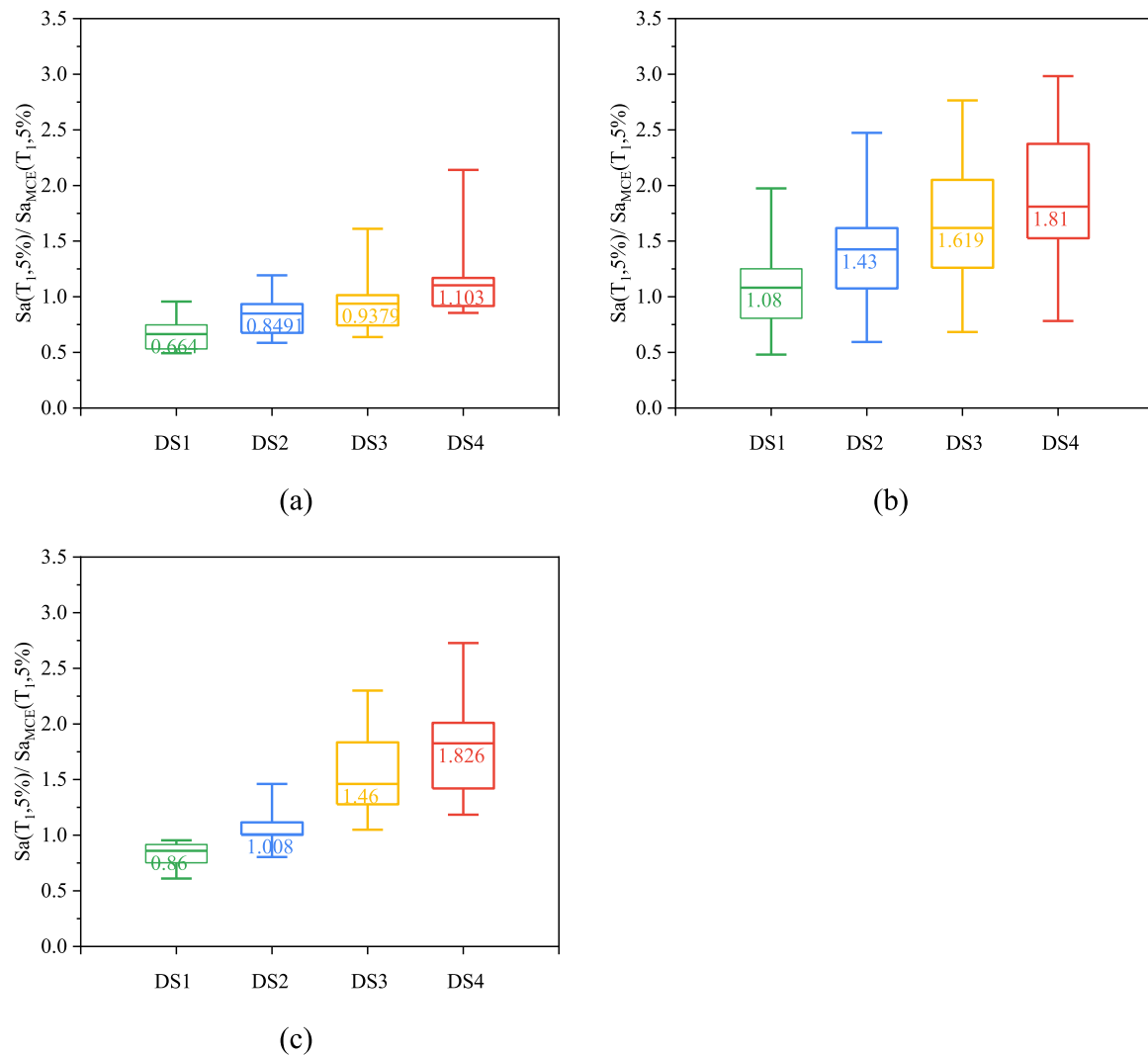
Fig. 10. Boxplots of spectral acceleration for (a) 4-story (b) 8-story (c) 12-story modular steel buildings.
