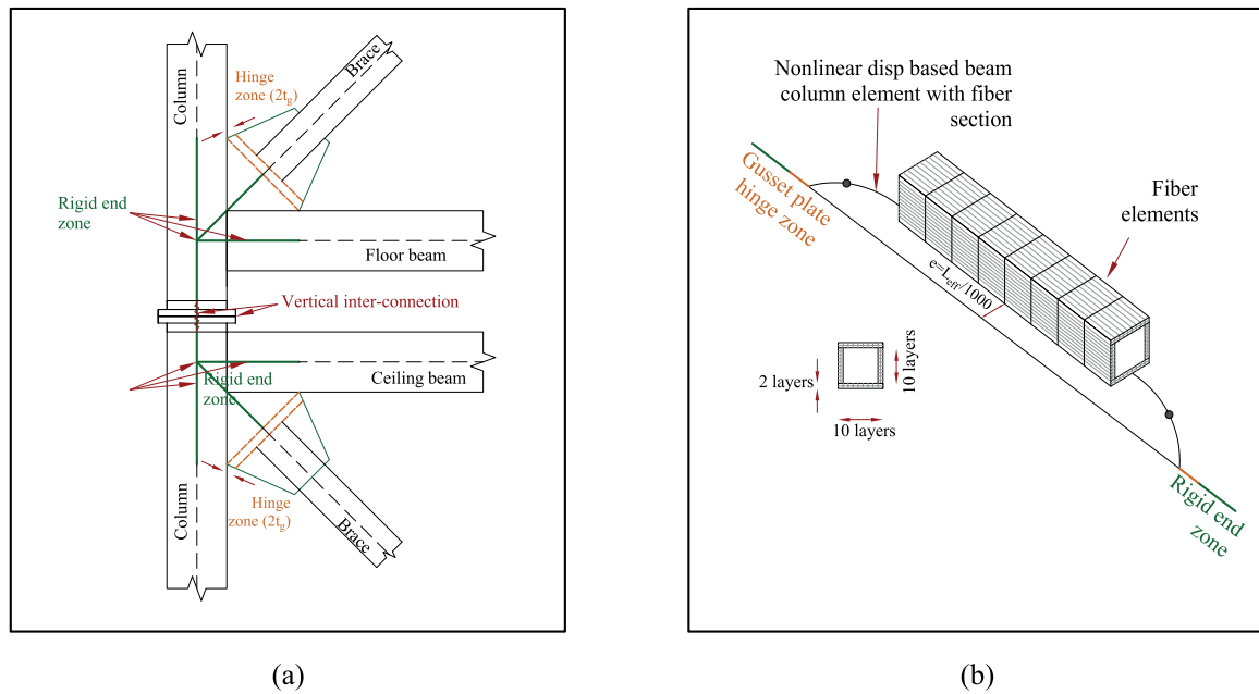
Fig. 7. Modeling details of (a) gusset plate (b) buckling behavior of brace [55].
