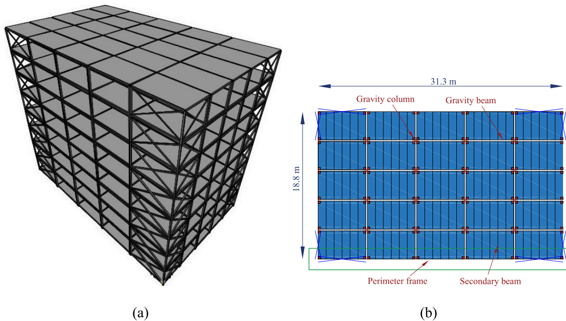
Fig. 4. (a) schematic 3D view of the 8-story MBS (b) Plan view of the studied MBSs.
