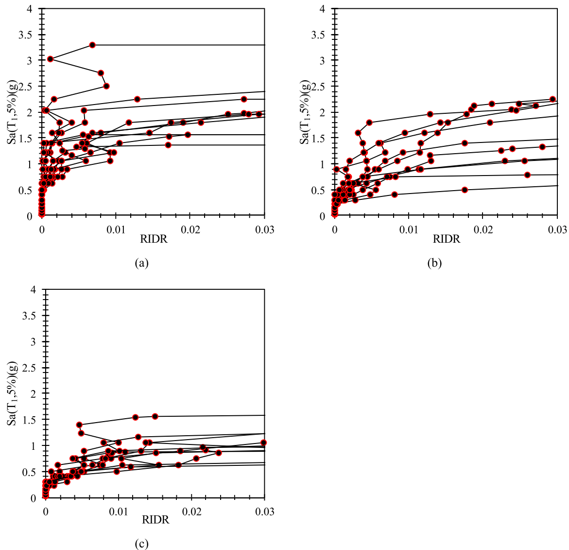
Fig. 9. IDA results of MBSs under the mainshock records considering RIDR, (a) 4-story (b) 8-story (c) 12-story.
