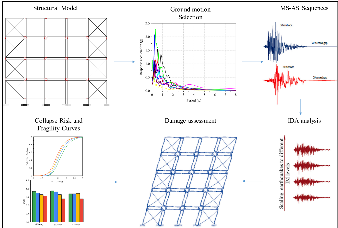
Fig. 1. Illustration of the process involved in developing MS-AS fragility curves for MBSs.
