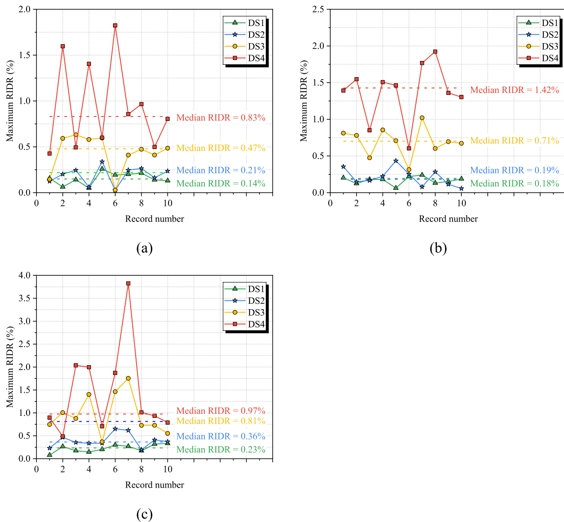
Fig. 13. The maximum residual inter-story drift ratio of (a) 4-story (b) 8-story (c) 12-story modular steel buildings subjected to mainshocks scaled at four IDR-based damage states.
