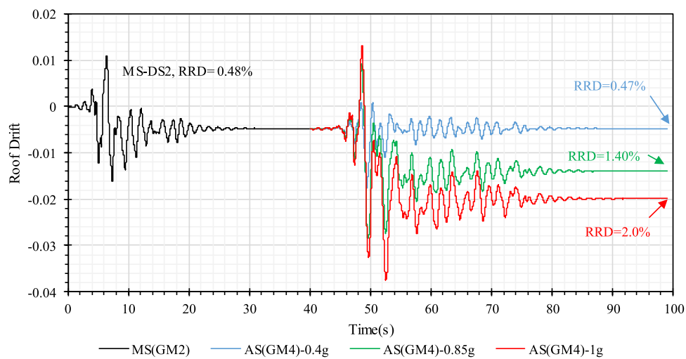
Fig. 11. Roof drift results for the 8-story MBS under mainshock-aftershock sequences with the same AS records but different intensities.
