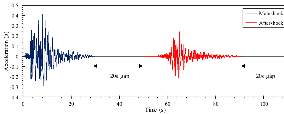
Fig. 3. Input acceleration time history of MS-AS sequences.
