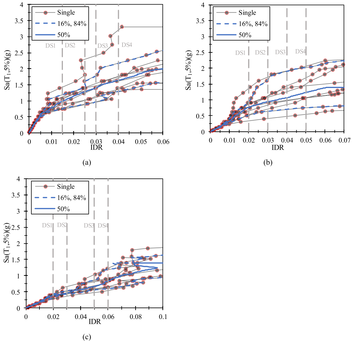
Fig. 8. IDA results of MBSs under the mainshock records considering IDR, (a) 4-story (b) 8-story (c) 12-story.
