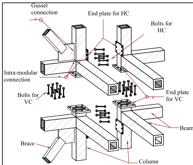
Fig. 5. Vertical and horizontal IMC details [56].
