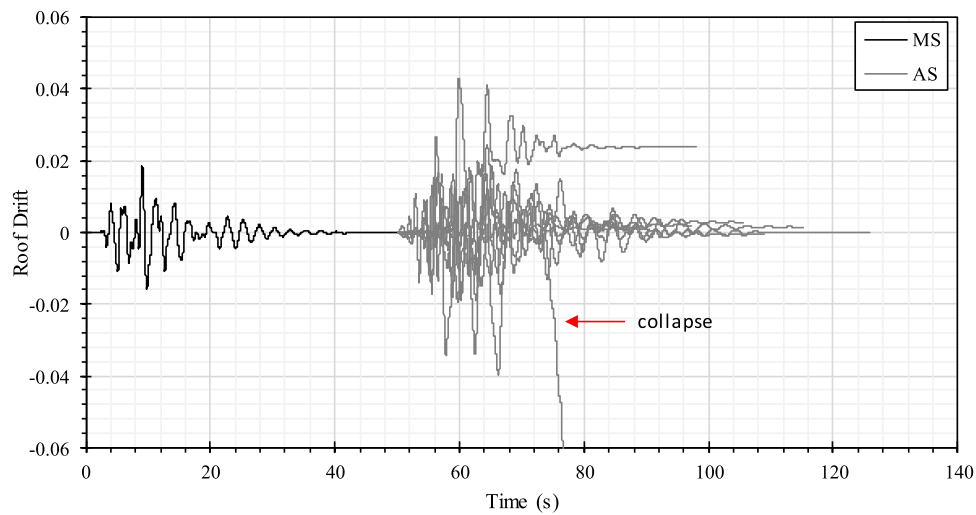
Fig. 12. Roof drift results for the 8-story MBS under mainshock-aftershock sequences with the different AS records at S_a(T_1, 5\%) = 0.75 g.
