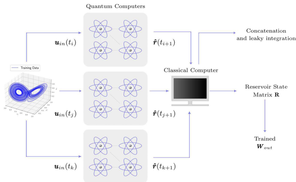
Fig. 11 Recurrence-free quantum reservoir computing parallel training. Input data \mathbf{u}_{in}(t) is divided into smaller-length signals and passed through multiple parallel quantum computers. The obtained reservoir activation signals \hat{\mathbf{r}}_{in}(t) associated with each input time series signal
