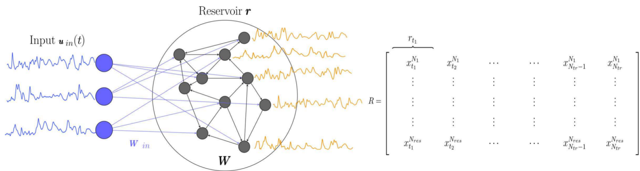
Fig. 2 Training phase in reservoir computing. Input time series \mathbf{u}_{in}(t) is mapped to a reservoir using \mathbf{W}_{in} matrix for CRC and suitable encoding schemes for QRC. Inside reservoir r , each neuron echoes with the input time series to generate a series of reservoir activation state signals.
