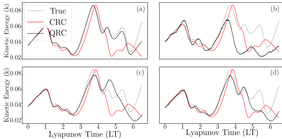
Fig. 3 Prediction of the MFE time series on unseen data set with a a noise-free probability distribution, b 0.5 \times 10^5 shots, c 2 \times 10^5 shots, d 4 \times 10^5 shots. Classical reservoir computing (CRC) results from the best-
