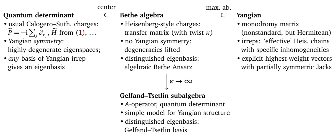
Figure 1: Overview of the role of the Yangian, and distinguished subalgebras, for the spin-Calogero–Sutherland model. Traditionally one considers the Calogero–Sutherland-style charges (left) and the Yangian (right). In this work we focus on the Heisenberg-style charges (middle). The Haldane–Shastry spin chain inherits this setup upon freezing.
