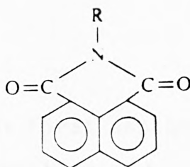
Naphthylimide
