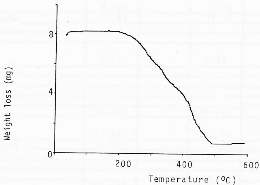
Fig. 3.13 Thermogravimetric analysis curves for poly- propylene containing 2 phr ferrocene + 20 phr Cereclor
