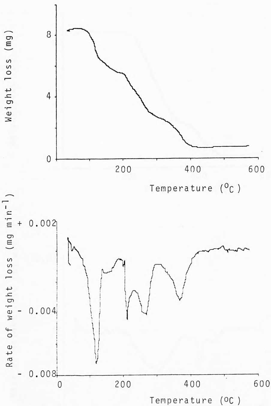
Fig. 3.10 Thermogravimetric analysis curves for a 3:7 mixture of ferrocene and Cereclor
