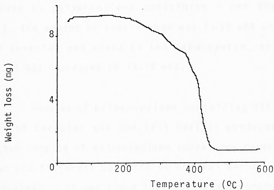
Fig. 3.17 Thermogravimetric analysis curves for polypropylene containing 1 phr BHB tris Fe(III) + 15 phr Cereclor
