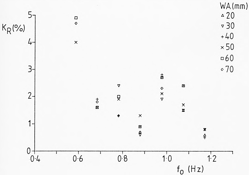
Reflection Coefficient
