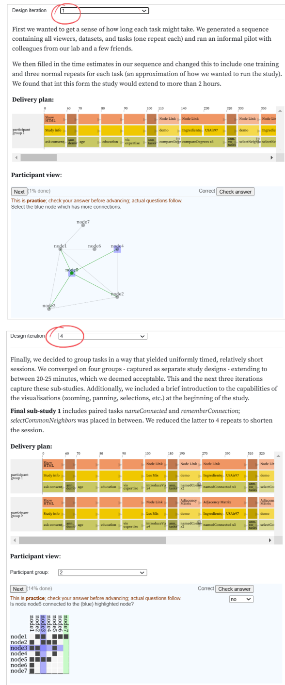
Figure 7: Our literate replica of Okoe et al.’s study captures the evolution of the study’s final design as a sequence of iterations. Each iteration is justified and its corresponding delivery is shown and can be experienced interactively. The figure illustrates the first and fourth iteration.
