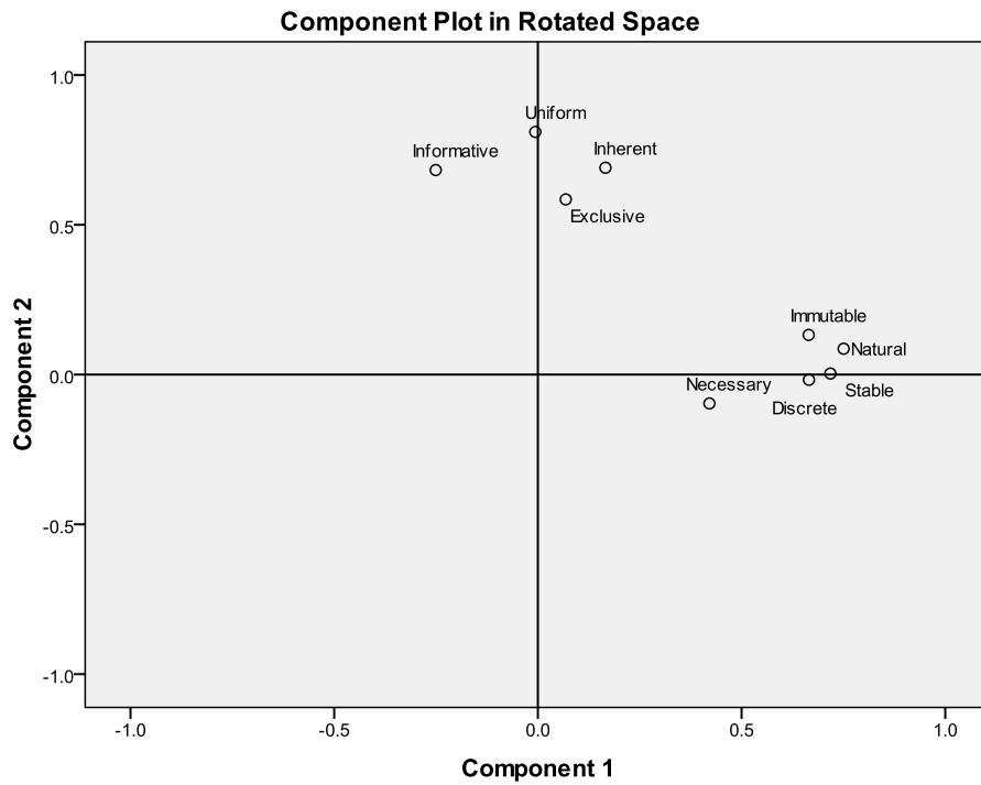
Figure 5.2. Factor Loadings for Factor 1 and Factor 2, Study 1
