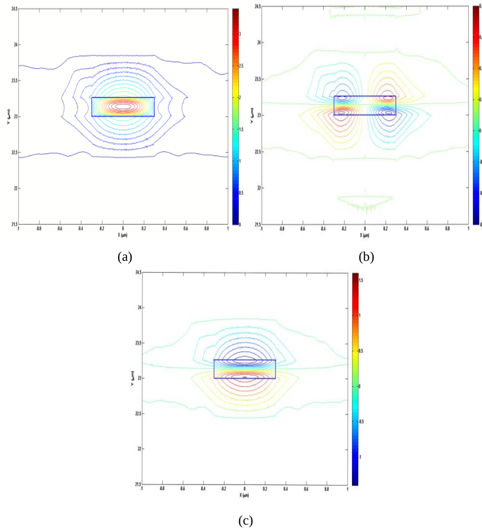
Figure 5.47. The quasi-TE mode of (a) H_y (b) H_x and (c) H_z field profiles of PS waveguide H0.26W0.60μm.
