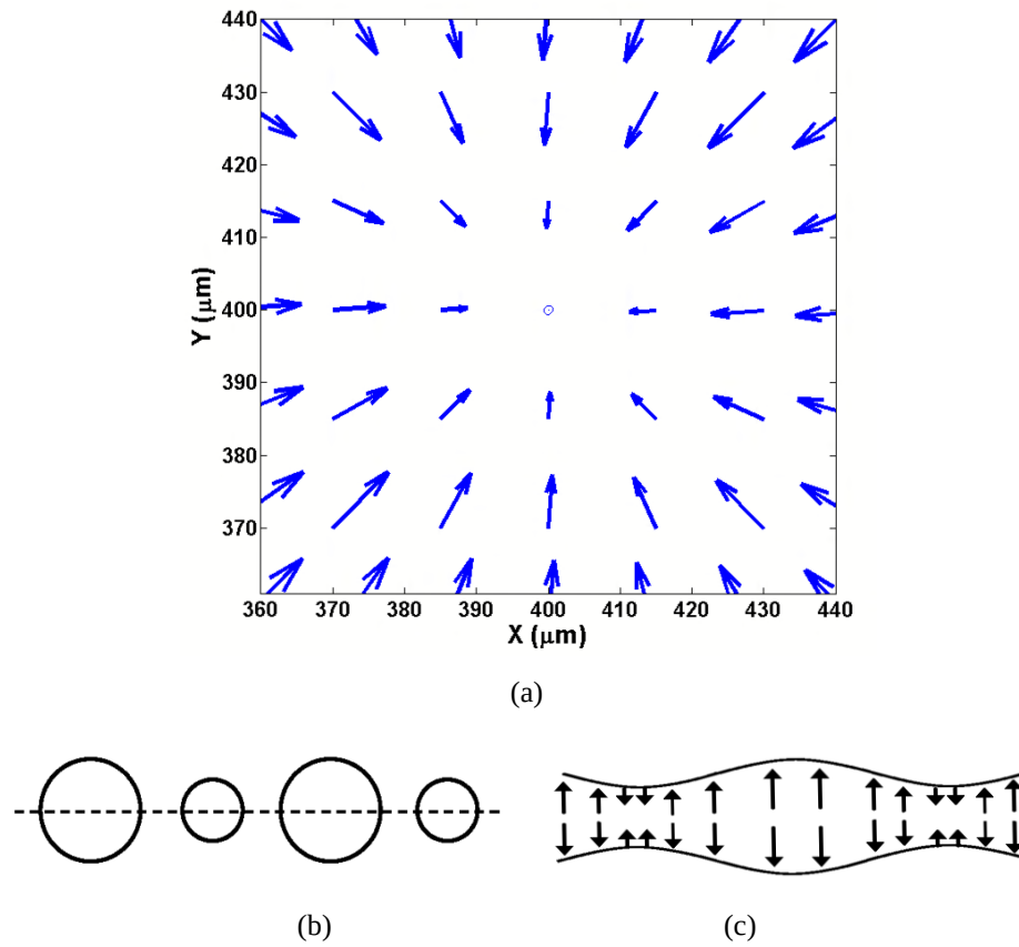
Figure 2.21. S_{11} Shear mode for the Radial mode (R) of the (a) vector plot U_t = \vec{U}_x + \vec{U}_y , (b) the characteristic of the Radial mode propagation, (c) the periodic displacement of Radial mode.
