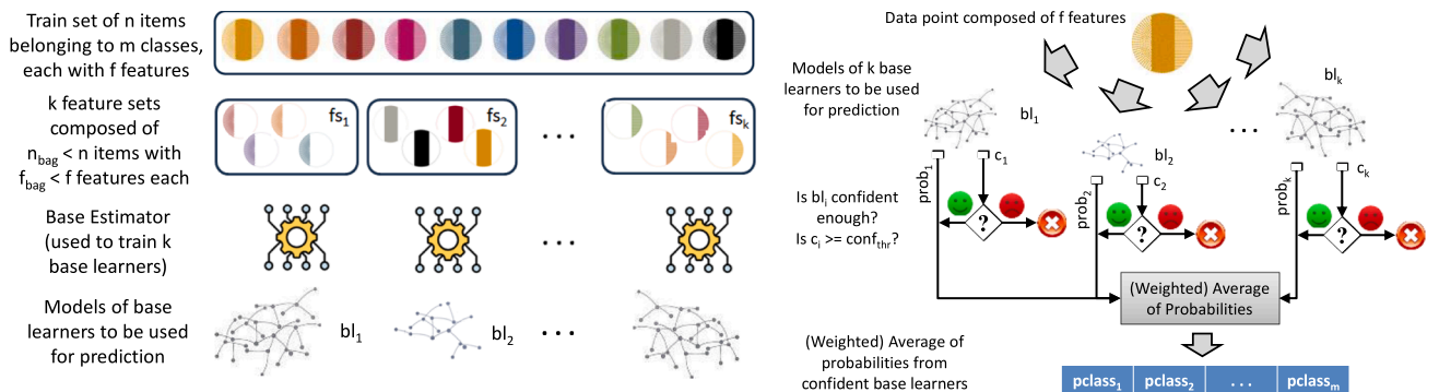
Fig. 1. Train (left) and test (right) schemas for Confidence Bagging (ConfBag) at a glance.
