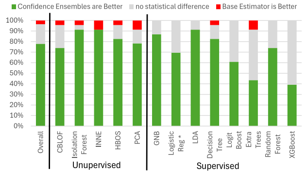
Fig. 7. The bar chart shows the percentage of cases in which confidence ensembles are statistically better (green), worse (red), no statistical difference (light-grey) against base estimators.
