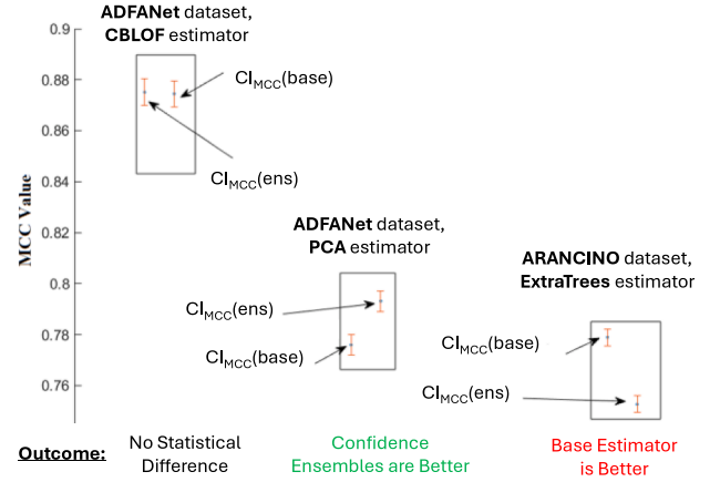
Fig. 6. Examples of possible outcomes of the statistical validation: i) no statistical difference (left), ii) confidence ensembles are better than the base estimator (center), and iii) the base estimator is better than confidence intervals (right).
