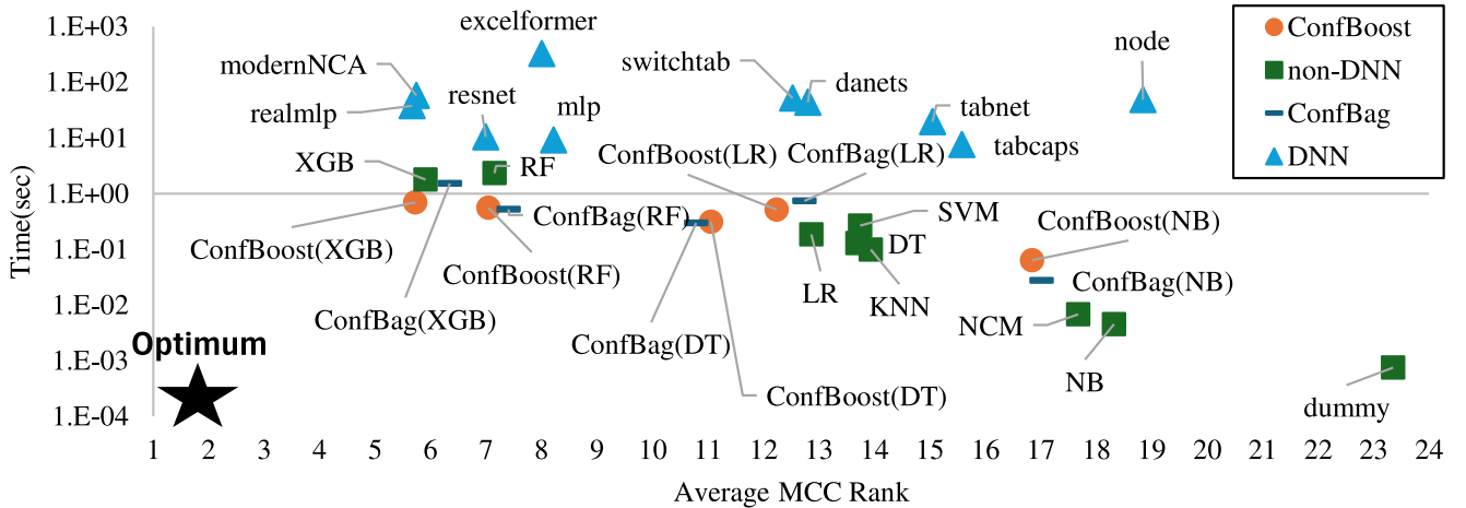
Fig. 3. Results using the TALENT benchmark: ConfBag (blue dashes) and ConfBoost (orange circles) are exercised alongside non-DNN (green squares) and DNN (light-blue triangles) classifiers. The plot shows the MCC rank against training time, averaged across 100+ datasets.
