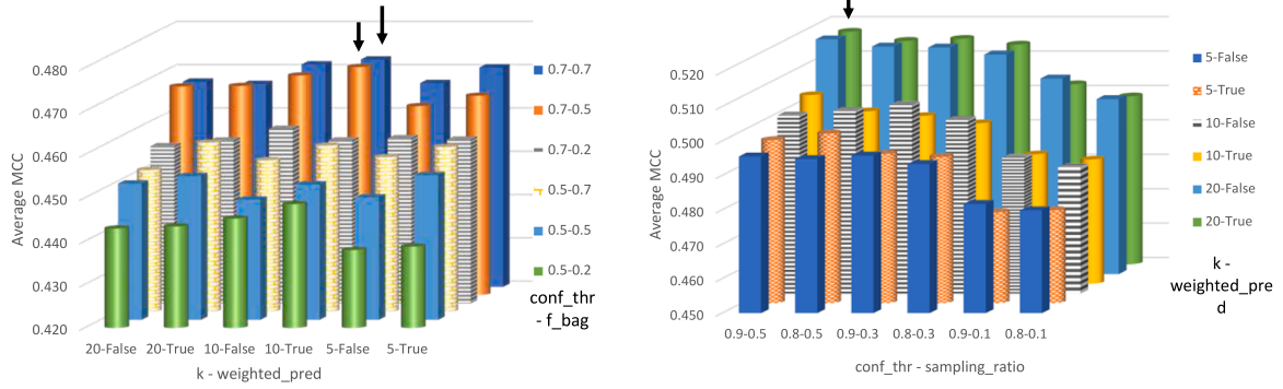
Fig. 4. Variation of MCC scores for different combination of hyperparameters for ConfBag (left) and ConfBoost (right) ensembles.
