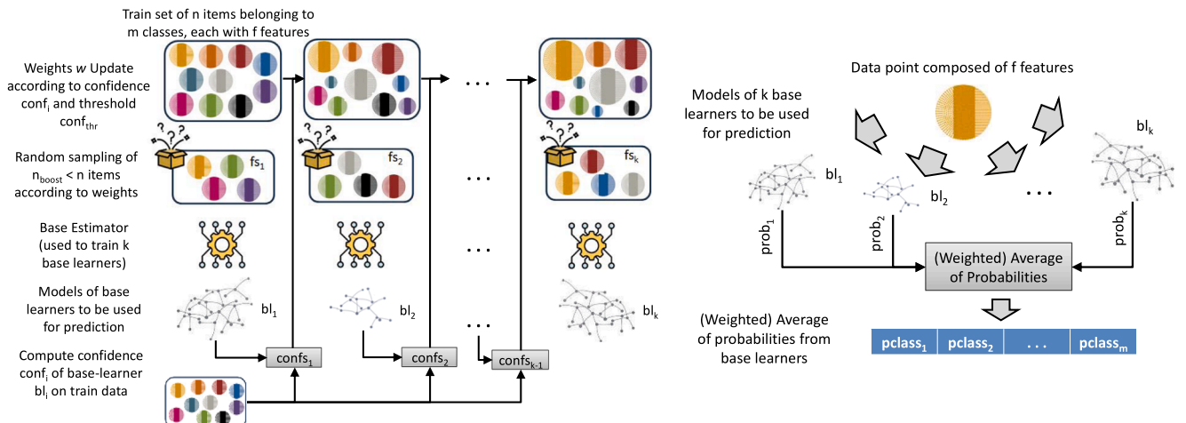
Fig. 2. Train (left) and test (right) schemas for Confidence Boosting (ConfBoost) at a glance.
