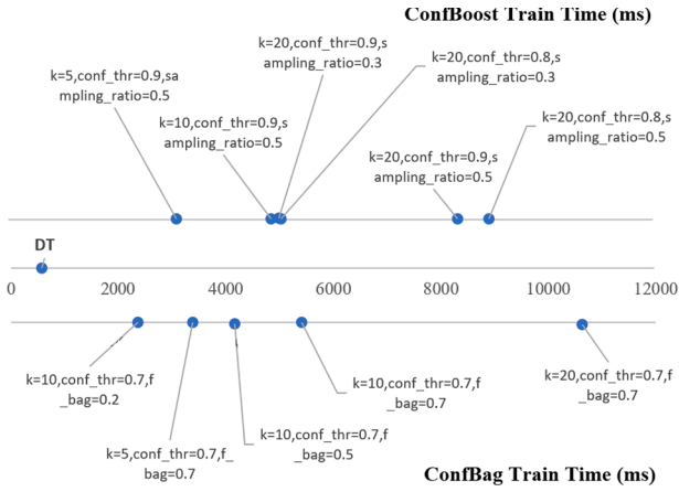
Fig. 5. Variation of Train Time for different instances of ConfBag (down in the figure) and ConfBoost (up) built over Decision Trees as base estimator (DT, middle of the plot).
