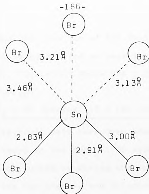
Figure 3.2a The environment of Sn(1): Trigonal pyramidal
