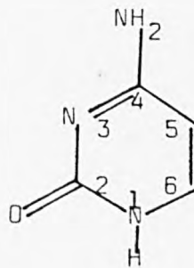
(e) Cytosine
