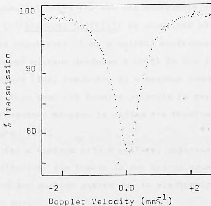
Figure 1.8 Mössbauer spectrum of \text{BaSnO}_3 using a \text{Ba } ^{119}\text{Sn O}_3 source.
