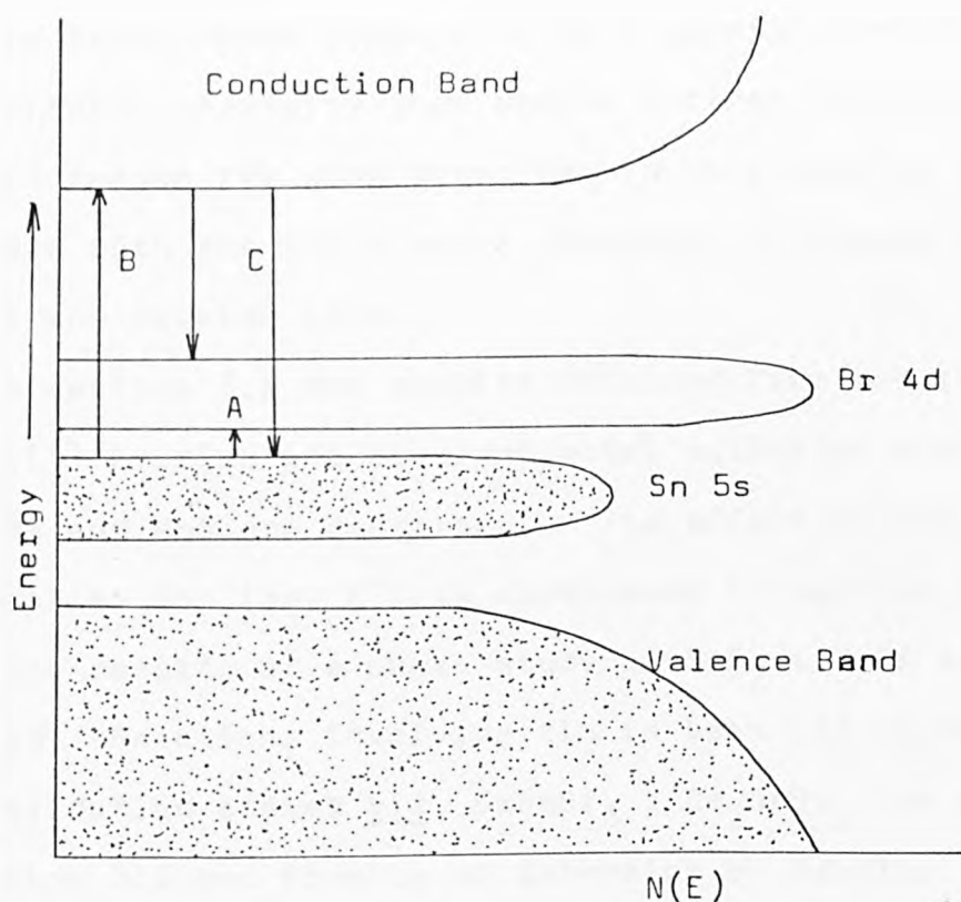
Suggested band structure for CsSnBr 3 showing thermal population (A), optical absorption (B) and emission (C).
