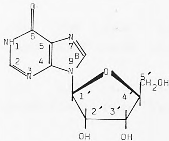
(c) Inosine
