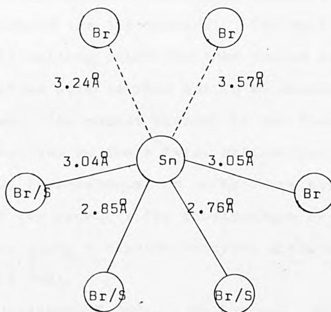
Figure 3.2b The environment of Sn(2): Square pyramidal
