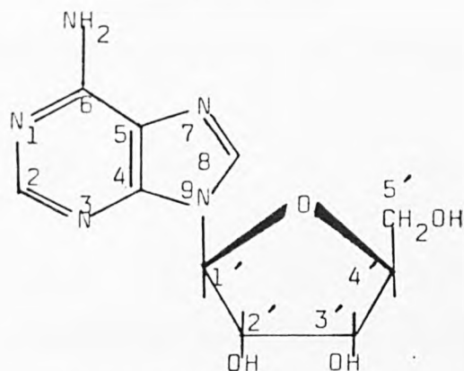
(a) Adenosine
