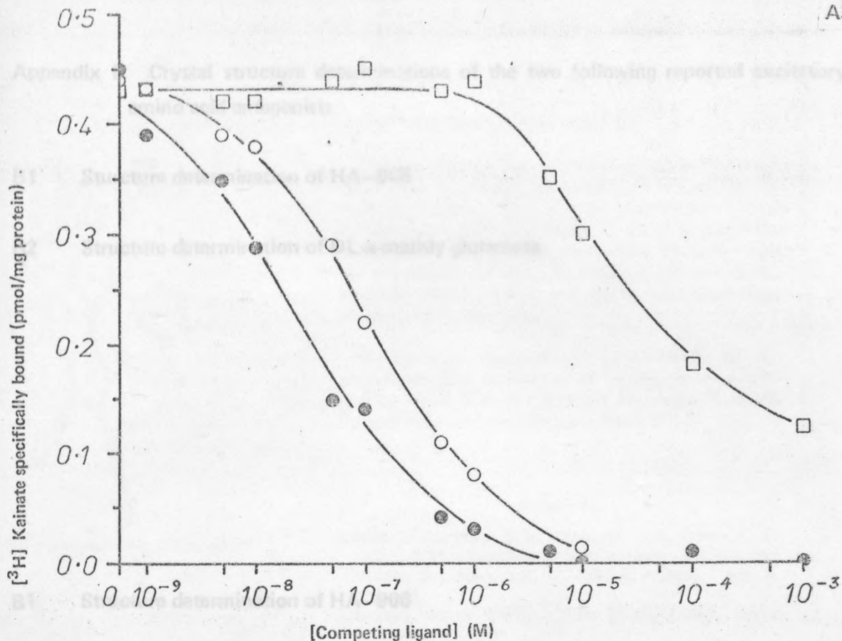
Fig A3.3 Inhibition curves for various compounds competing with specific [ 3 H] kainate binding. The routine assay was followed employing challenging compound concentrations over the range 10 -9 – 10 -3 M. Results are means of triplicate determinations. ● Kainate; ○ quisqualate; □ L-aspartate.
