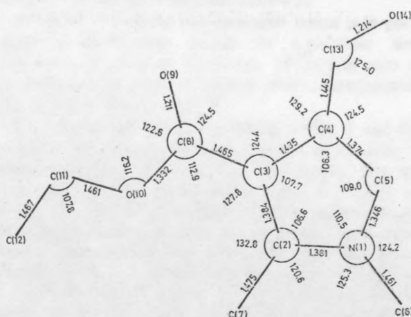
Fig. 2. Bond lengths (Å) and angles (°) involving the non-hydrogen atoms (standard deviations are 0.004 Å and 0.2° respectively).
