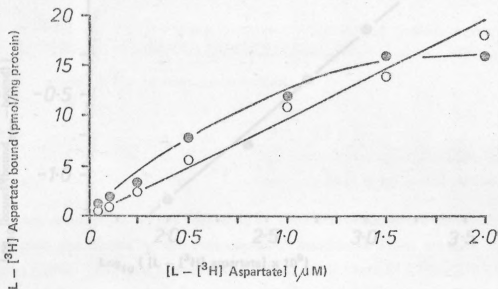
Fig. A2.1 Saturability of specific L - ^3\text{H} aspartate binding. The routine assay was followed except that final L - ^3\text{H} aspartate concentrations were varied over the range 0.05 - 2.0 \mu\text{M} . Results are means of triplicate determinations which varied by less than 9%. ● Specific; ○ nonspecific.
