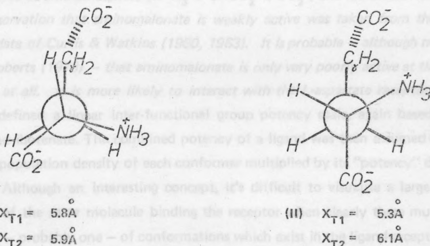
Fig 5.8 Possible active conformers of L-glutamate
