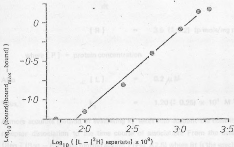
Fig. A2.3 Hill plot of the specific binding data of Fig. A2.1
