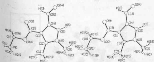
Fig. 1. A stereodrawing of the molecule.
