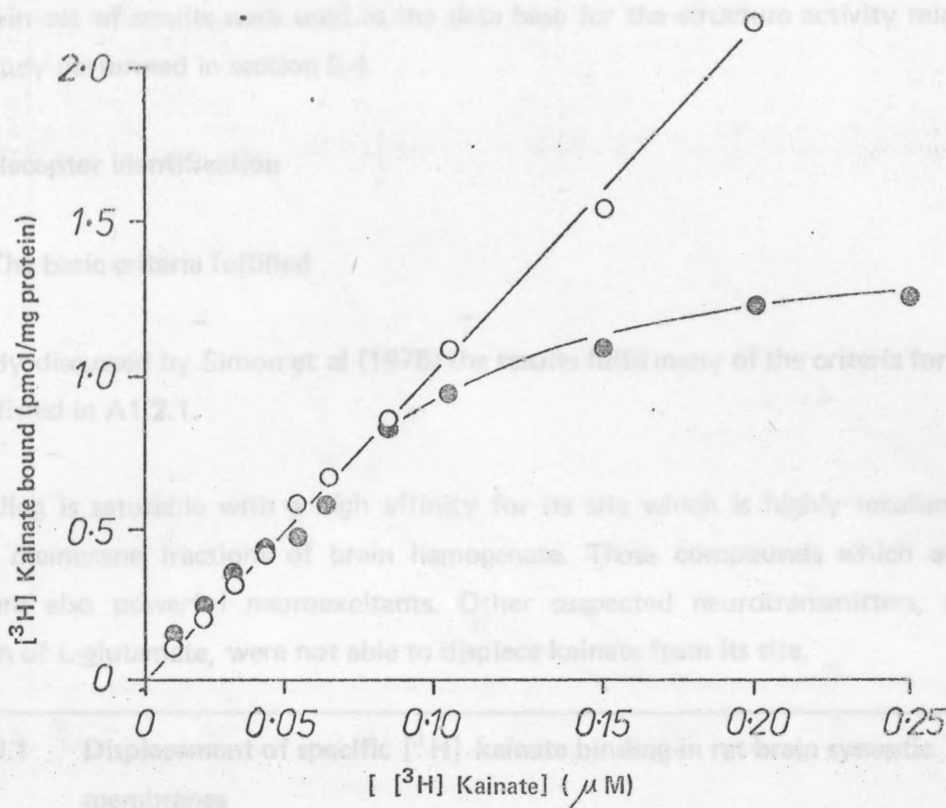
Fig A3.1 Saturation of specific [ 3 H] kainate binding • Specific; o nonspecific
