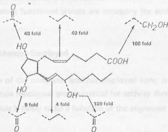
Fig 6.3 Relative importance of functional groups in \text{PGF}_{2\alpha} binding to bovine corpus luteum receptor (decreases of K_s following the structural modifications shown), (After Hammarstrom et al, 1976).
