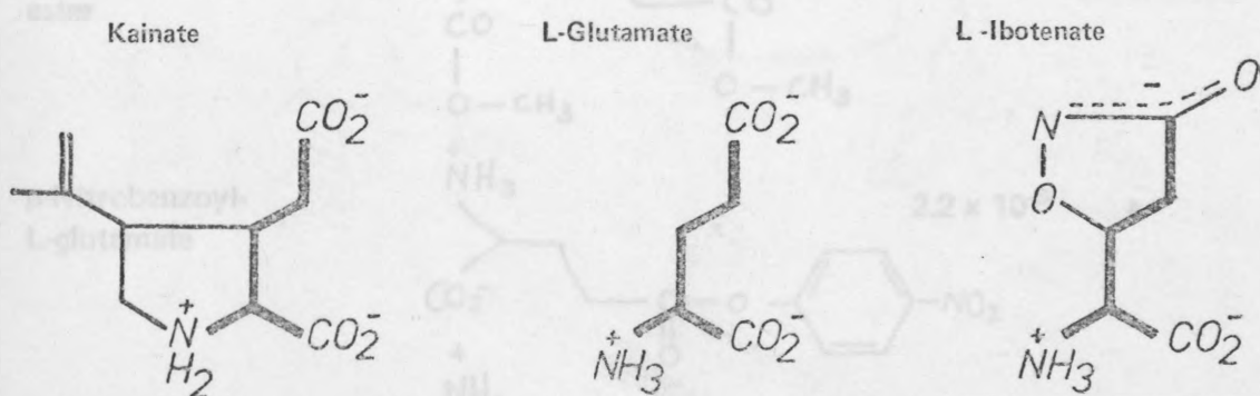
Fig 5.10 Structural congruences with L-glutamate skeleton
