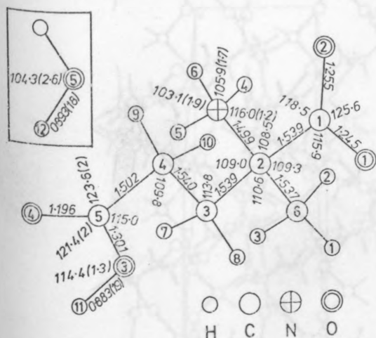
Fig. 1. Atomic numbering scheme, bond lengths (Å) and angles ( ^\circ ) for D,L- \alpha -methylglutamic acid. E.s.d.'s are 0.002 Å for bonds and 0.1 ^\circ for angles except where indicated otherwise. Bond lengths and angles not included on the figure are given below. Bond lengths (Å): N–H(4) 0.935 (16), N–H(5) 0.915 (16), N–H(6) 0.907 (16). Bond angles ( ^\circ ): C(2)–N–H(5) 111.0 (1.2), C(2)–N–H(6) 113.0 (1.3), H(4)–N–H(5) 106.8 (1.8), C(1)–C(2)–C(3) 110.8 (1), C(6)–C(2)–N 108.4 (1).
