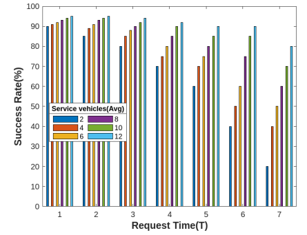
Fig. 8. Success Rate(%) w.r.t Request Time.
