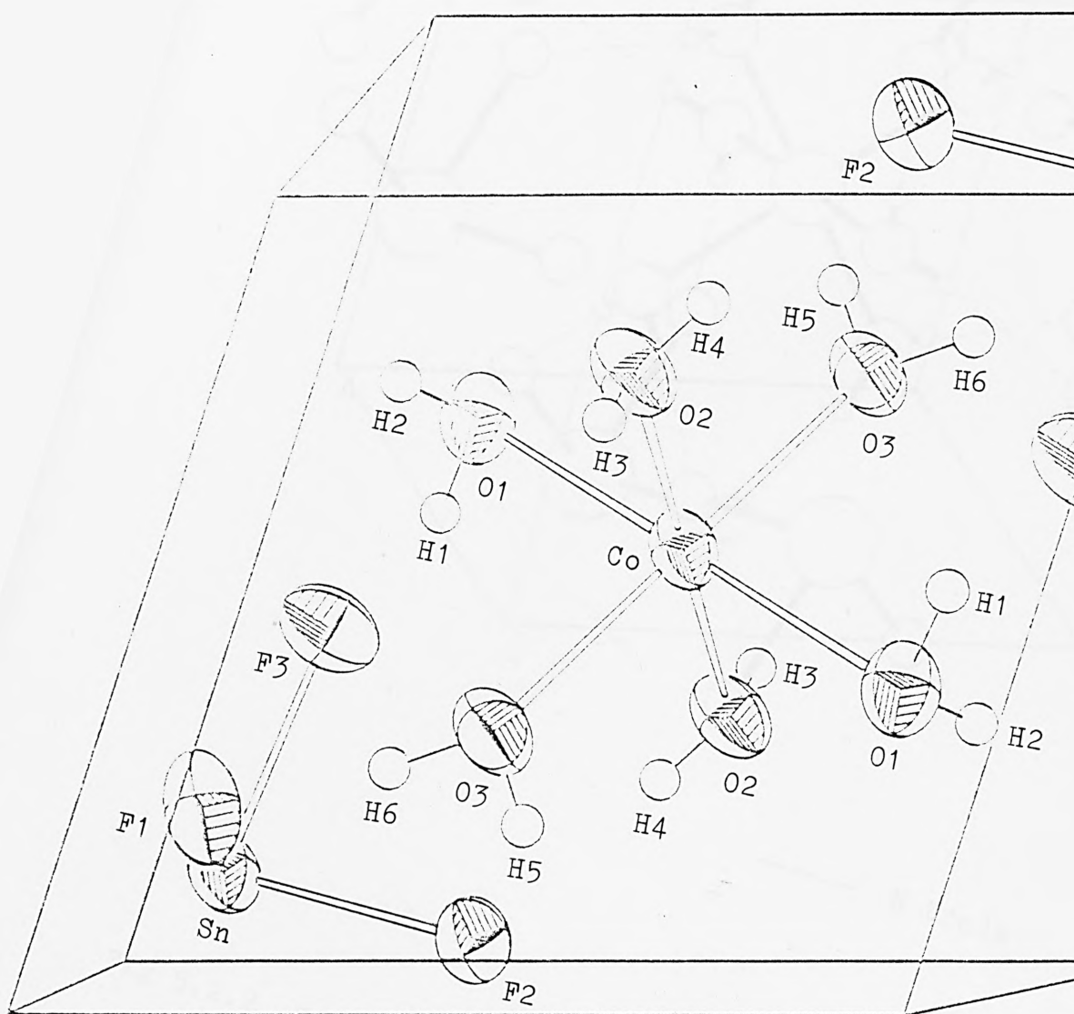
Fig 5.2.1 Thermal ellipsoid plot (50% probability) of the unit cell contents of \text{Co}(\text{SnF}_6) \cdot 6\text{H}_2\text{O}
