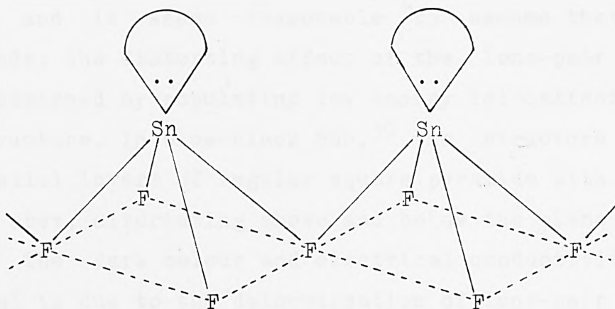
(c) \text{KSnF}_3 \cdot \frac{1}{2}\text{H}_2\text{O}
