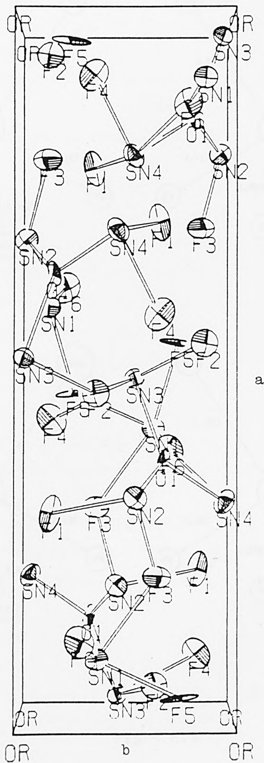
Fig 5.6.2 Thermal ellipsoid plot (50% probability) of unit cell contents of \text{Sn}_4\text{O}_6
