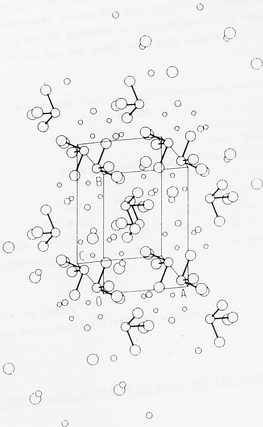
Fig 5.5.4 Packing diagram of \text{NH}_4\text{Br} \cdot \text{NH}_4\text{SnBr}_3 \cdot \text{H}_2\text{O} showing 3-dimensional array of discrete ions in the structure
