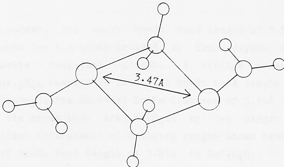
(b) [\text{Sn}(\text{NMe}_2)_2]_2
