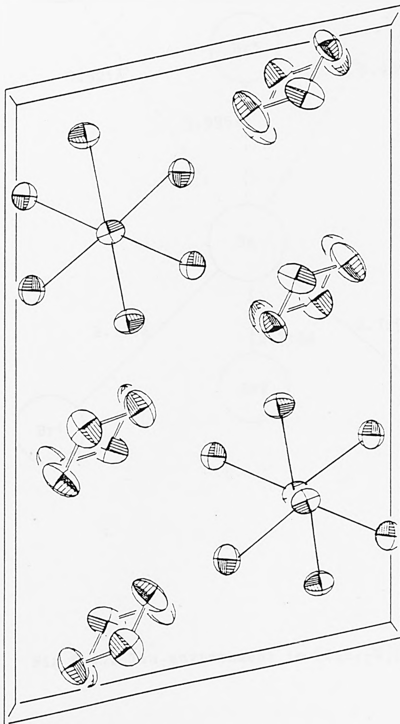
Fig 5.4.1 Thermal ellipsoid plot (50% probability) of the unit cell contents of [\text{C}_5\text{H}_{12}\text{N}][\text{SnBr}_3]
