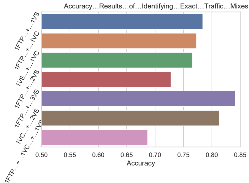
Figure 4.5: Accuracy results of identifying exact traffic mixes
