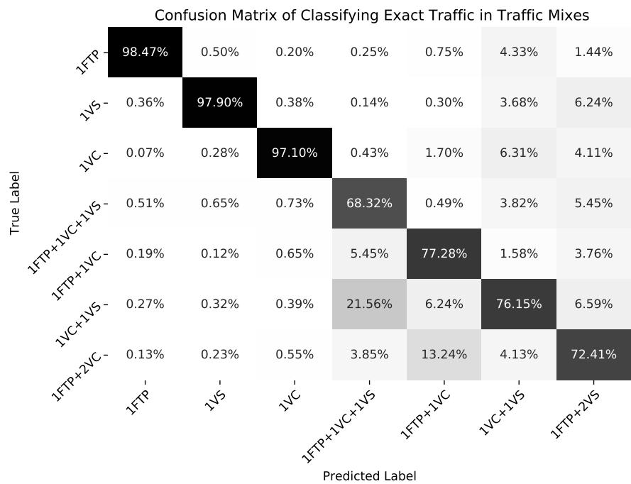
Figure 4.6: Confusion matrix of classifying exact traffic mixes.
