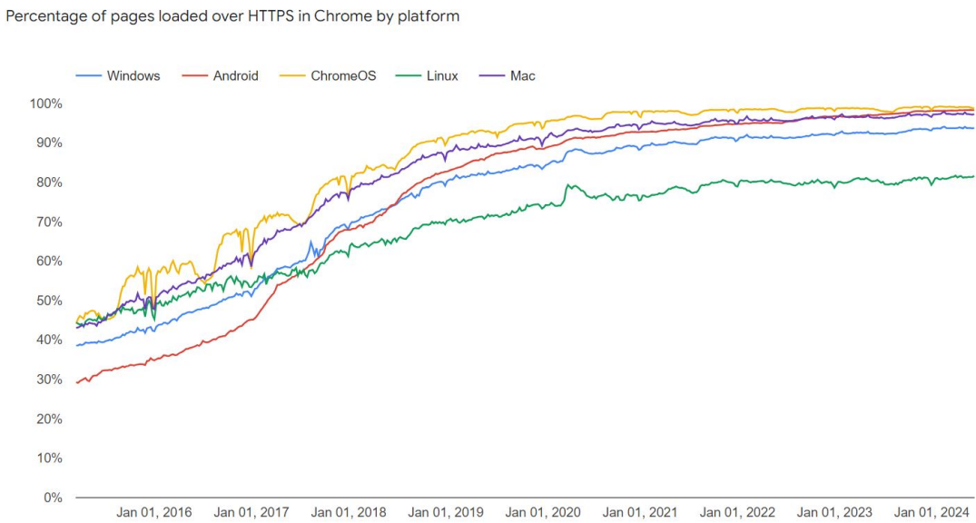
Figure 1.3: Percentage of Pages Loaded Over HTTPS in Chrome by Platform Google (2024).
