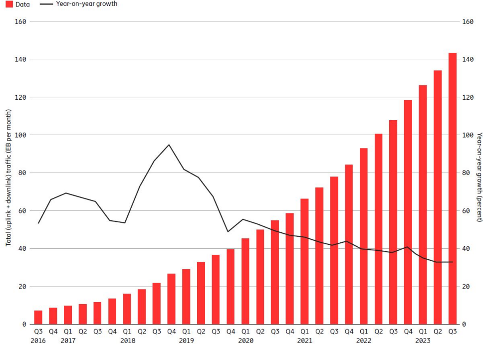
Figure 1.1: Global mobile network data traffic and year-on-year growth (EB per month) Ericsson (2021) .
