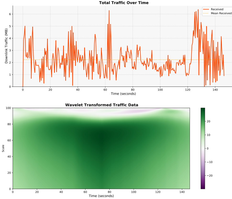
Figure 1.5: Downlink Traffic Data Over Time and Wavelet Transform Analysis.
