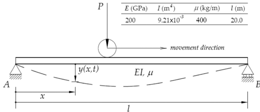
Fig. 4. Specification of simply supported beam.
