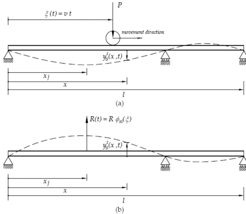
Fig. 2. Surrogate beam induced by eliminating a reaction.
