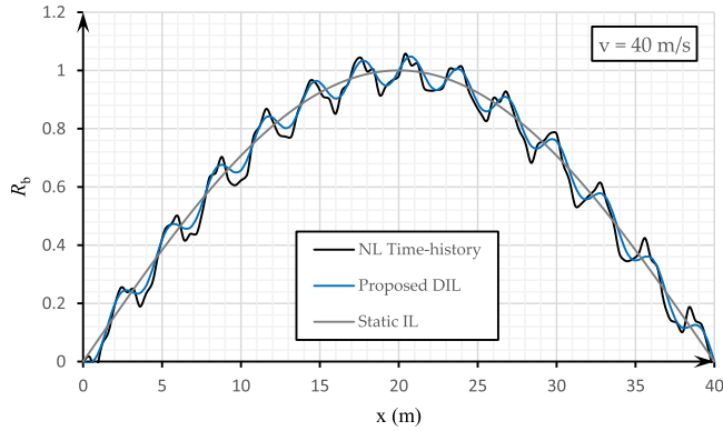
Fig. 15. Variation of the support B reaction determined by different methods.
