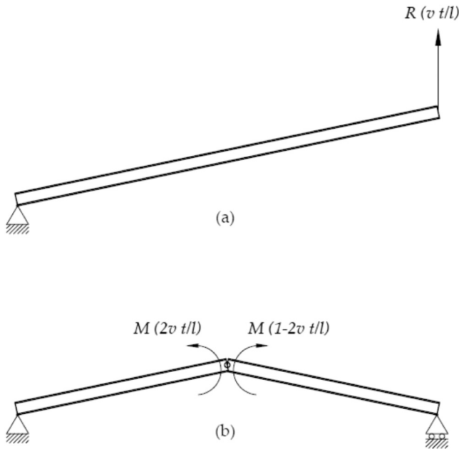
Fig. 5. Surrogate beams for determination of: (a) the support B reaction; (b) the mid-span moment.
