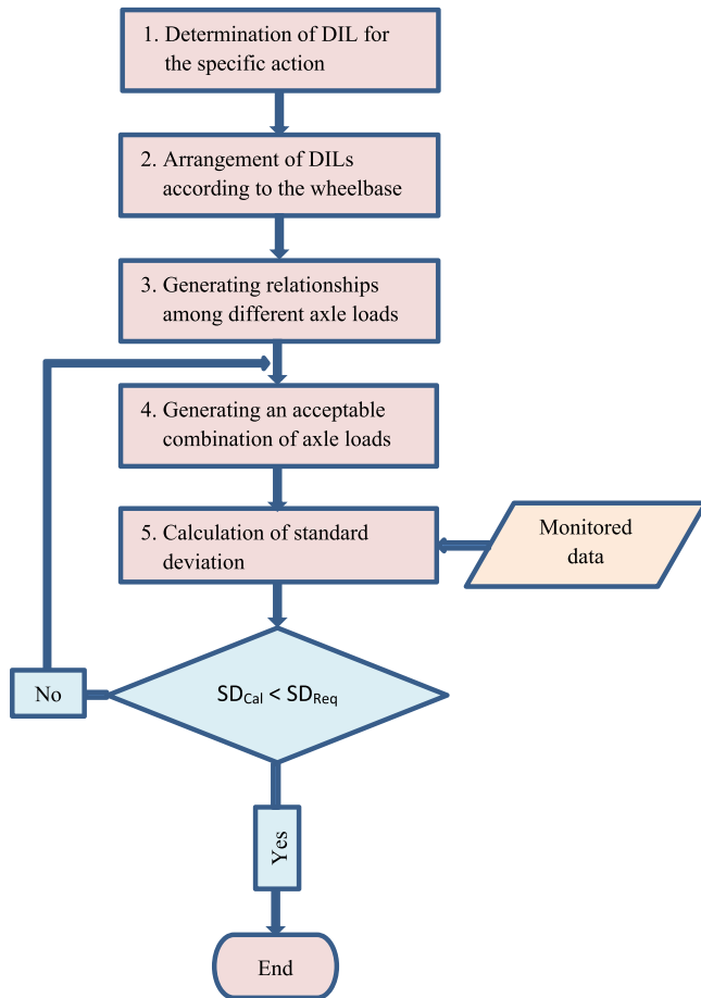
Fig. 18. Flowchart of moving load identification.
