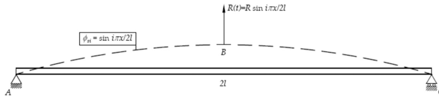
Fig. 14. Surrogate beam for determination of the support B reaction.
