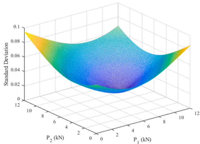
Fig. 22. Standard deviation in terms of different values of axle loads.
