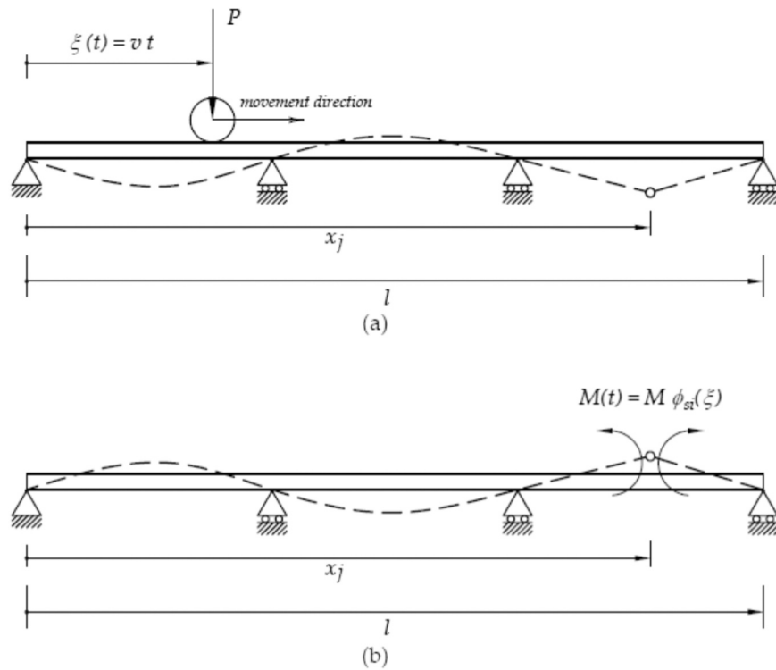
Fig. 3. Surrogate beam for internal moment influence line.
