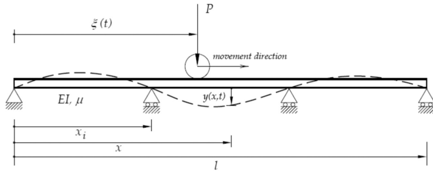
Fig. 1. Specification of a multi-span beam under a moving load.
