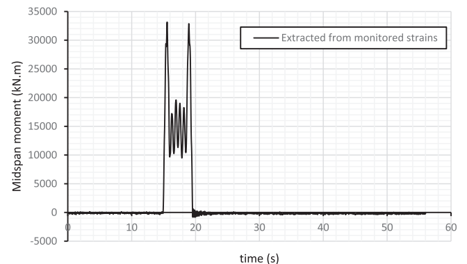
Fig. 25. Midspan moment during the time.
