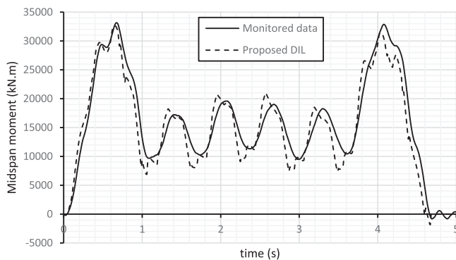
Fig. 27. Comparison between the monitored and predicted data.
