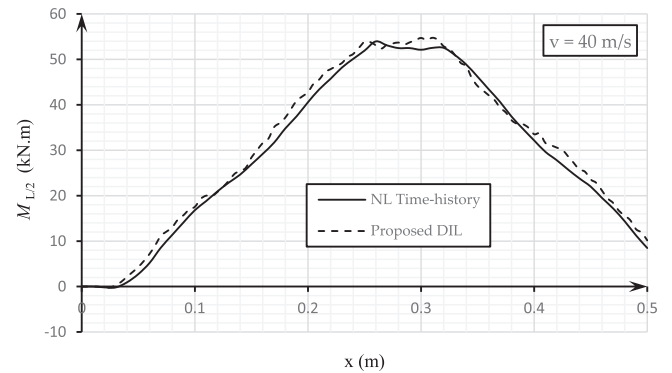
Fig. 23. Mid-span moment during the time.
