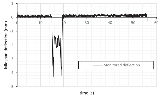
Fig. 24. Midspan deflection during the time.
