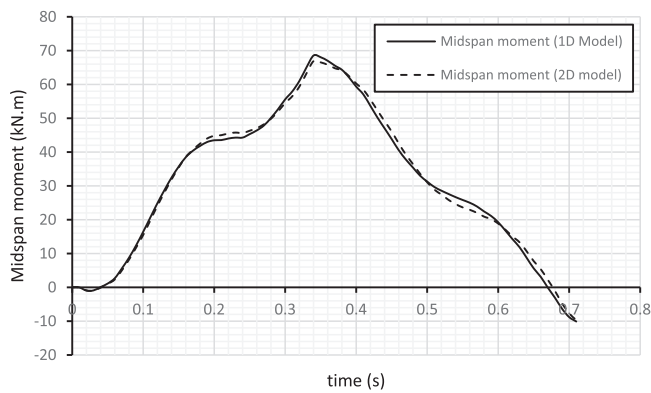
Fig. 26. DIL of mid-span moment (velocity=37.6 m/s).
