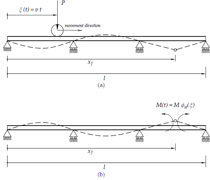
Fig. 3. Surrogate beam for internal moment influence line
