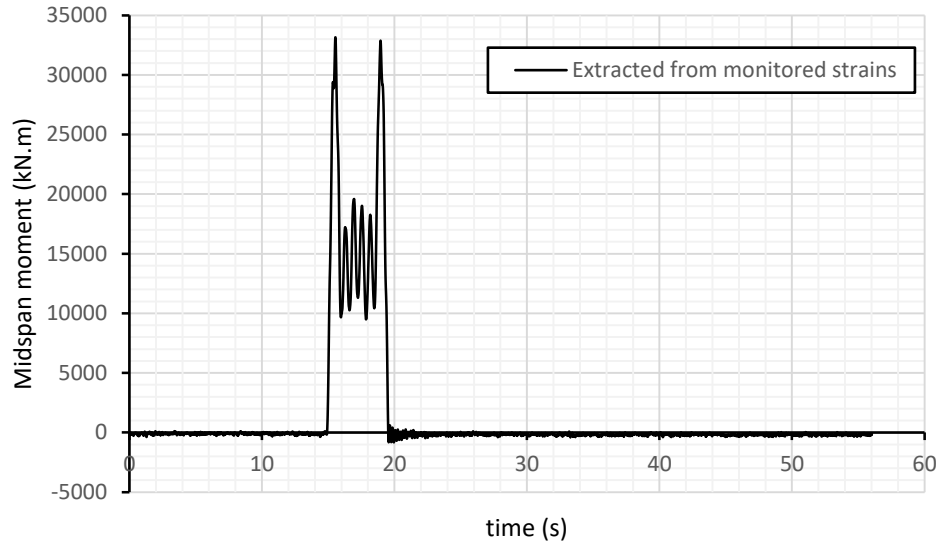
Fig. 25. Midspan moment during the time
