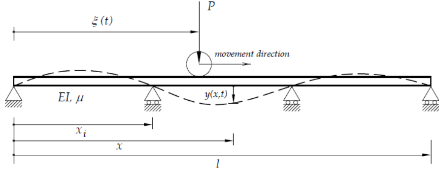
Fig. 1. Specification of a multi-span beam under a moving load
