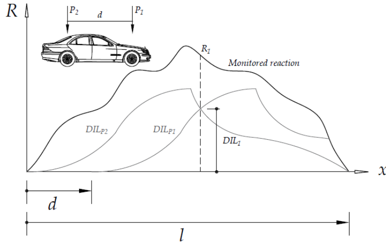
Fig. 19. Application of DIL method for moving load identification
