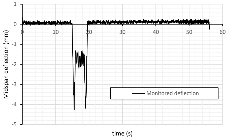
Fig. 24. Midspan deflection during the time
