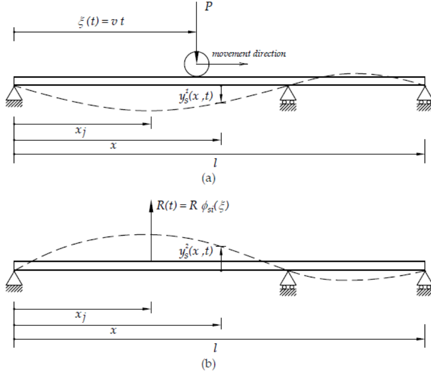
Fig. 2. Surrogate beam induced by eliminating a reaction
