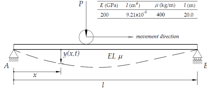
Fig. 4. Specification of simply supported beam
