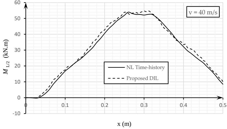
Fig. 23. Mid-span moment during the time
