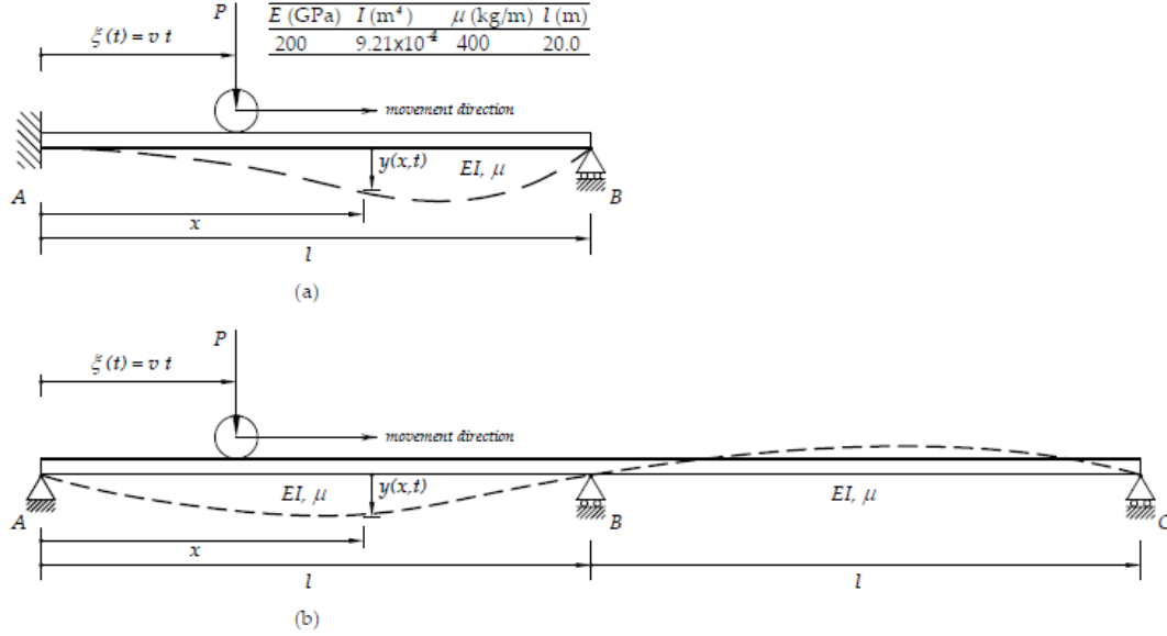
Fig. 10. Two statically indeterminate beams under a single moving load
