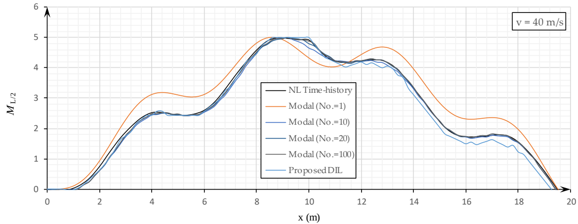
Fig. 7. Variation of the mid-span moment during the load passage
