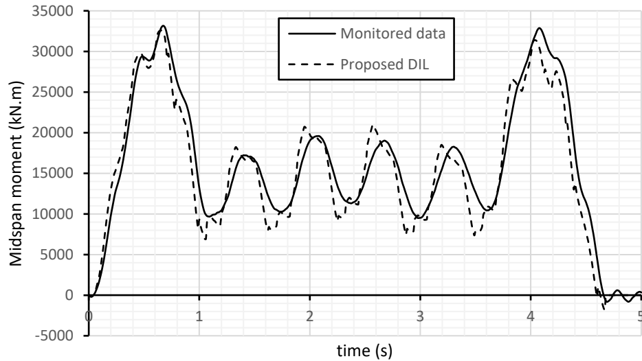
Fig. 27. Comparison between the monitored and predicted data
