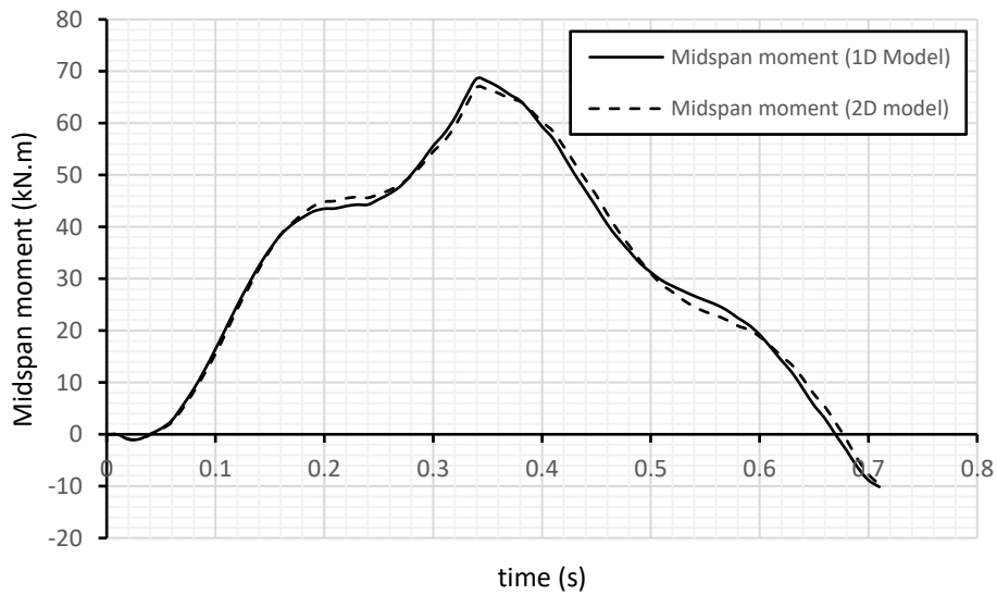
Fig. 26. DIL of mid-span moment (velocity=37.6 m/s)
