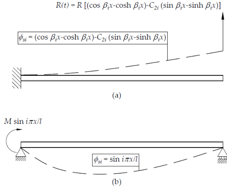
Fig. 11. Surrogate beams for determination of: (a) the support B reaction; (b) the support A moment
