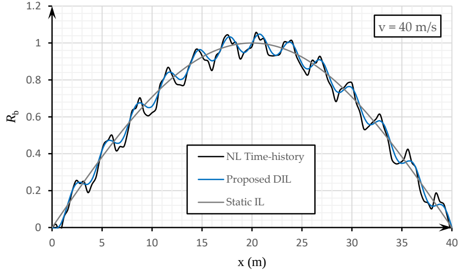
Fig. 15. Variation of the support B reaction determined by different methods
