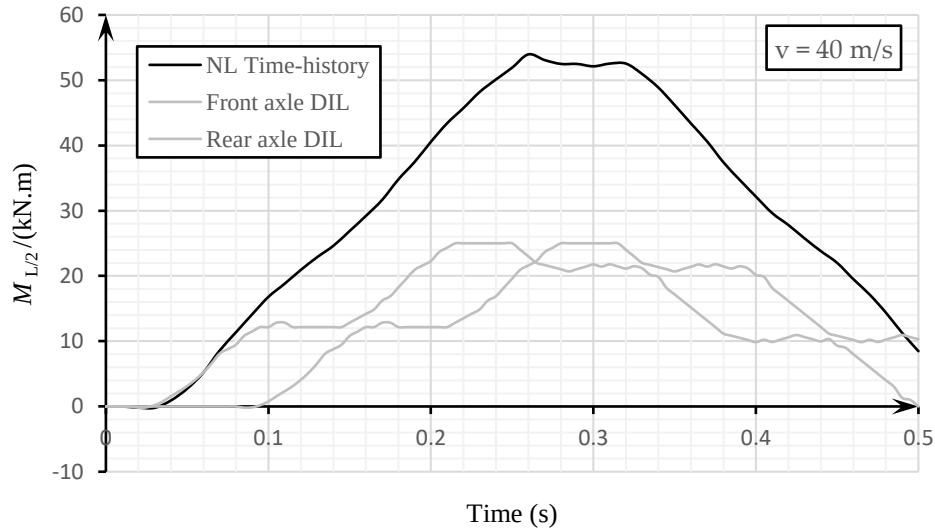
Fig. 21. Mid-span moment during the time obtained by nonlinear time-history analysis
