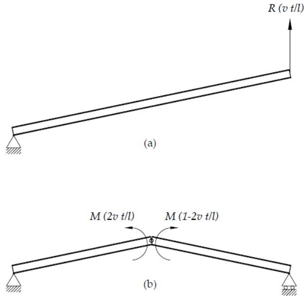
Fig. 5. Surrogate beams for determination of: (a) the support B reaction; (b) the mid-span moment
