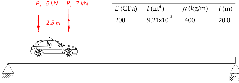
Fig. 20. A two-axle vehicle moving on a simple supported beam
