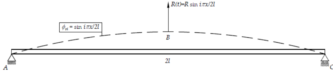
Fig. 14. Surrogate beam for determination of the support B reaction
