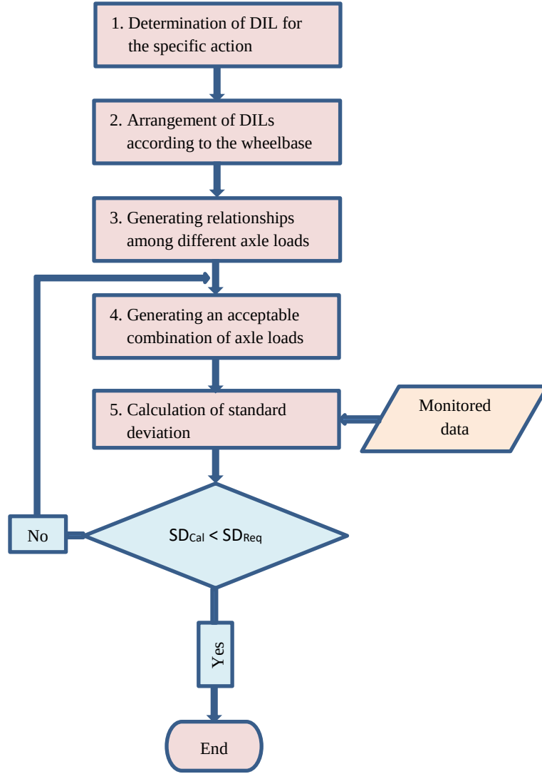
Fig. 18. Flowchart of moving load identification
