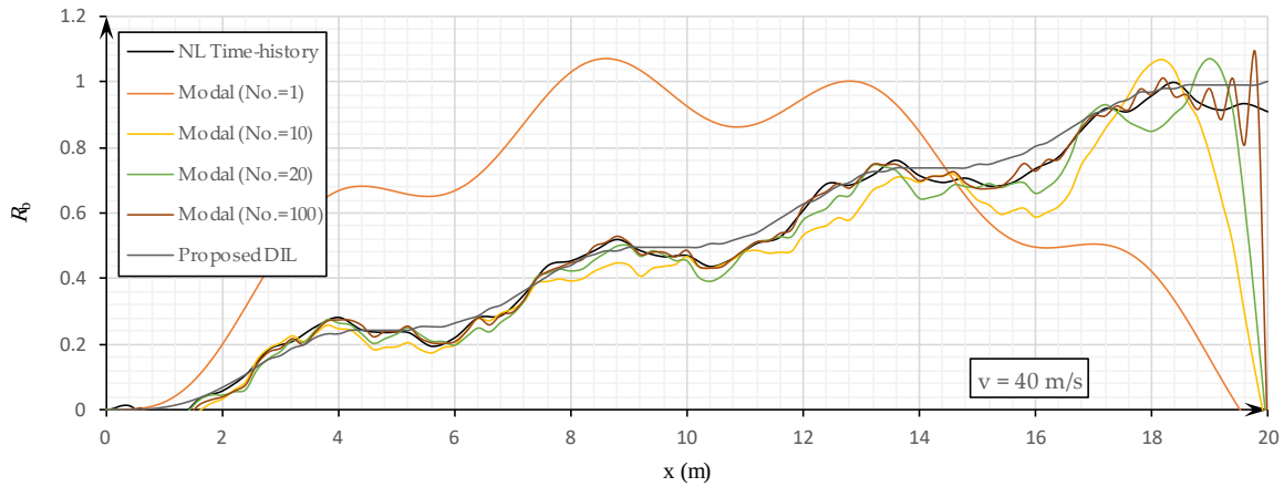
Fig. 6. Variation of the support B reaction during the load passage
