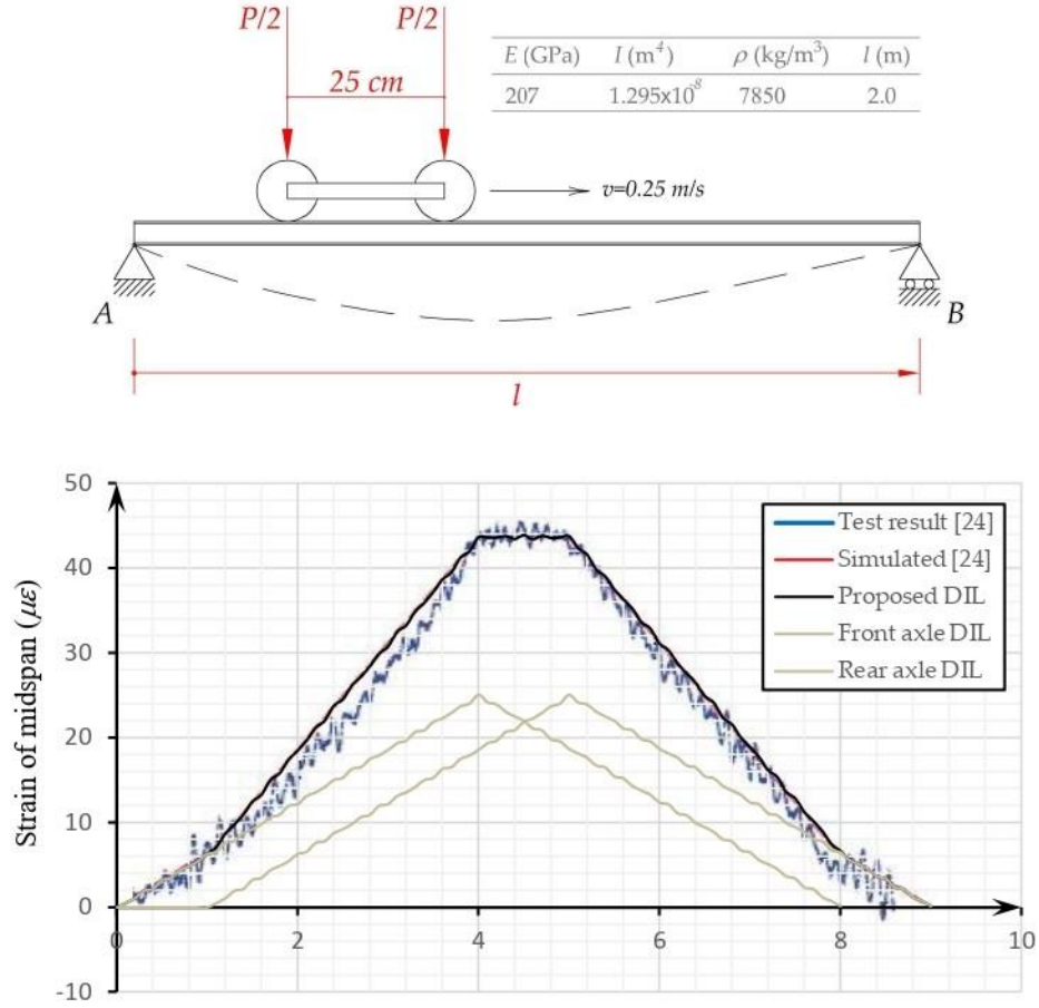
Fig. 17. Verification of the present method by comparing with test data [25]
