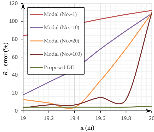
Fig. 16. Analysis error adjacent to the beam end
