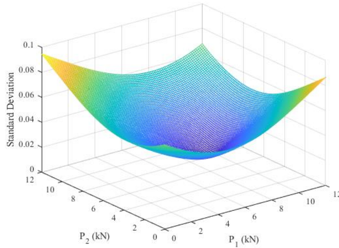
Fig. 22. Standard deviation in terms of different values of axle loads
