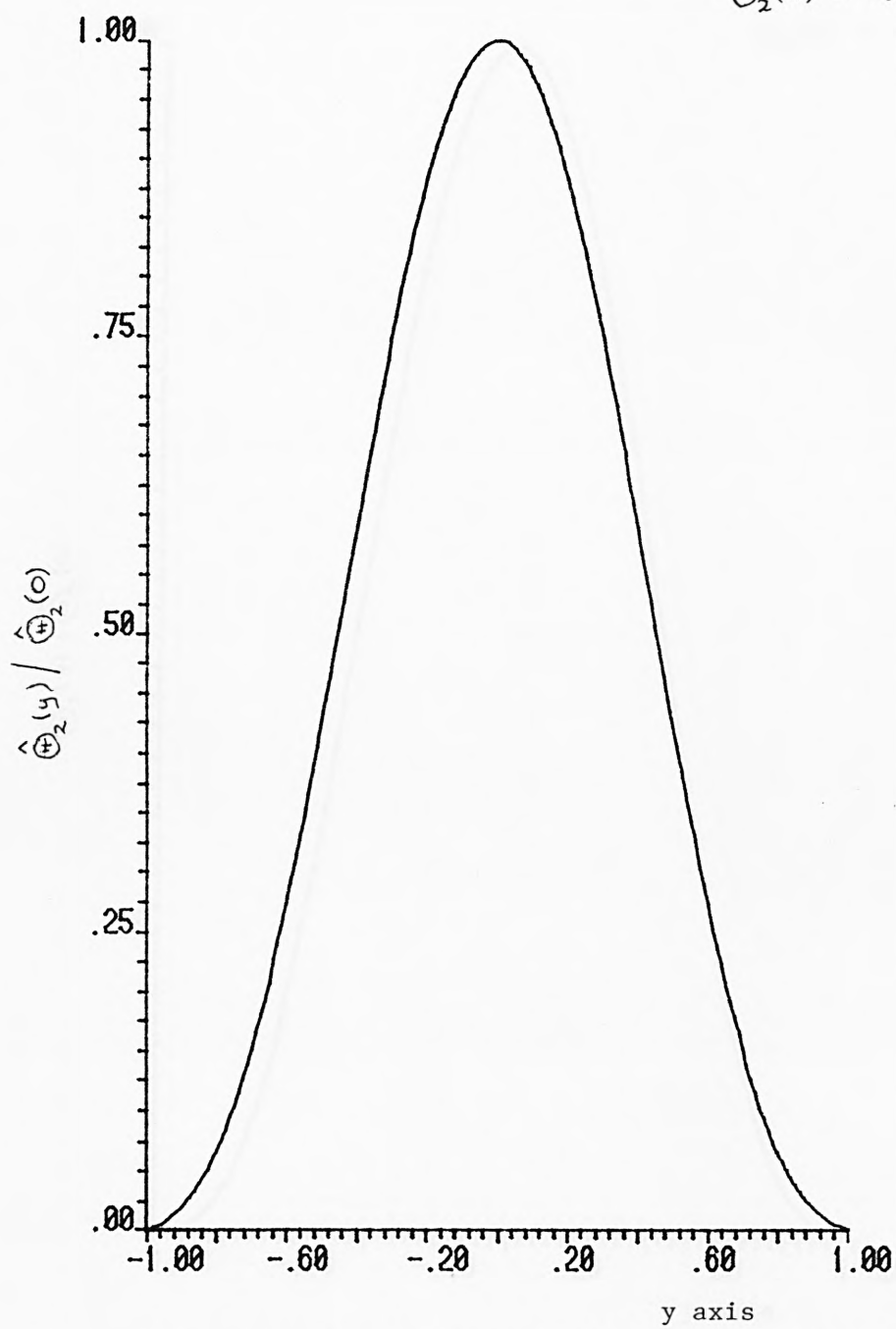
Figure 17b. Profile of the y-dependent function \hat{\Phi}_2^*
