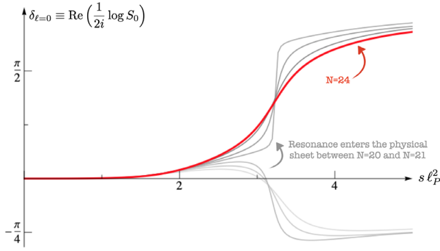
FIG. 4. Spin zero phase shift as we increase N from 18, ..., 23 (in gray) until 24 (in red). Between N = 20 and N = 21 a zero enters the physical sheet—it is the lightest resonance we encounter. Our best numerics with N = 24 seem to be close to converging in this energy range and hint at a mass of around m^2 \ell_p^2 \simeq 3.2 + 0.3i .
