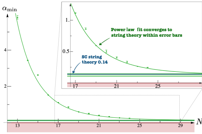
FIG. 2. Minimum \alpha_{\min}(N, \infty) obtained by extrapolating the various plateaus in Fig. 1. We estimate the error bars here by scanning over a large number of such fits as explained in the Supplemental Material [8], Appendix H. We then extrapolate these points to estimate \alpha_{\min}^{\text{Boot}} = \alpha_{\min}(\infty, \infty) \simeq 0.13 with an uncertainty represented by the green strip. It nicely embraces the strong coupling string prediction depicted by the solid blue line.
