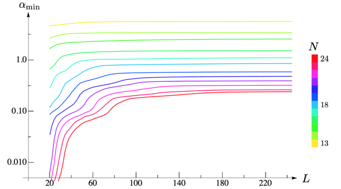
FIG. 1. Minimum \alpha_{\min}(N, L) . We see that the curves nicely converge towards a plateau whenever L is large enough. The larger N is, the further we need to go in L to reach this plateau. For each value of N we extrapolate these plateaus to estimate \alpha_{\min}(N, \infty) , which we plot in the next figure.
