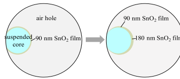
Fig. 2. Model of suspended core with \text{SnO}_2 film of 90 nm thickness used in the simulation.
