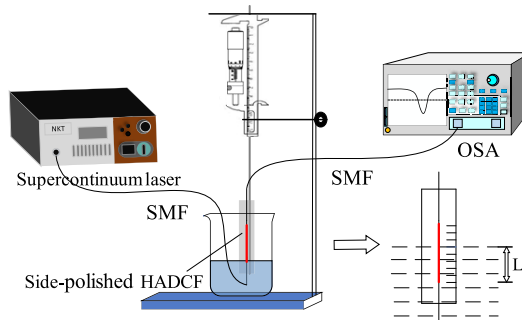
Fig. 4. Schematic diagram of test system used for RI sensing.
