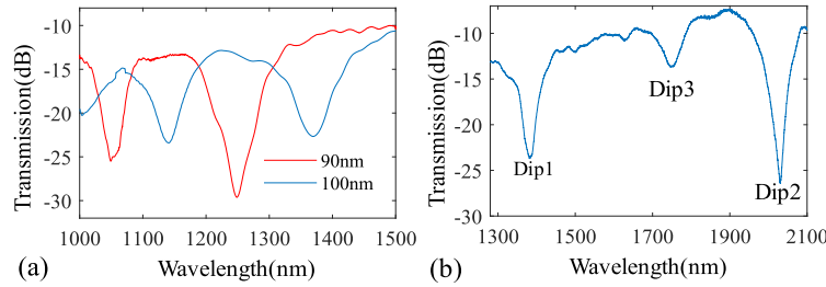
Fig. 5. (a) Transmission spectra of samples coated to different SnO 2 film thicknesses. (b) Transmission spectrum of a sample coated with a 100 nm thickness SnO 2 film, observing in the range 1300 - 2100 nm.
