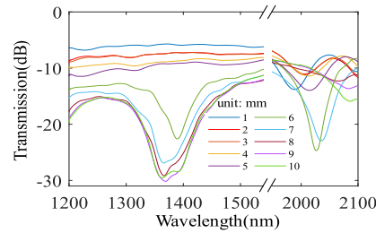
Fig. 6. Transmission spectra of a sample coated with 100 nm thickness SnO 2 film, for different depths of immersion into water.
