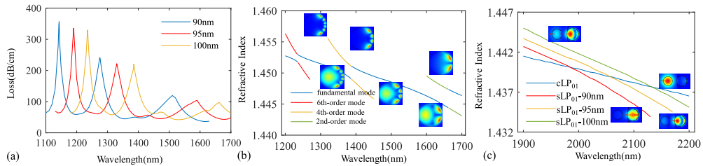
Fig. 3. (a) Confinement loss spectra of the suspended core with different thicknesses of the \text{SnO}_2 film. (b) Dispersion curves of the fundamental mode (blue line) in the suspended core and the higher-order modes (red, yellow and green lines) in the film with thickness of 100 nm. The inserts are the electric field distributions of fundamental mode, 6th-, 4th-, and 2nd-order loss modes. (c) Dispersion curves of the \text{cLP}_{01} and the \text{sLP}_{01} modes for different thicknesses of \text{SnO}_2 film. The inserts show the electric field distributions of the \text{cLP}_{01} and the \text{sLP}_{01} modes.
