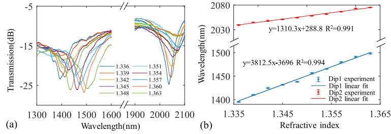
Fig. 7. (a) Transmission spectra for solution with the RI in range of 1.336-1.363. (b) RI sensitivities of Dip 1 and Dip 2.
