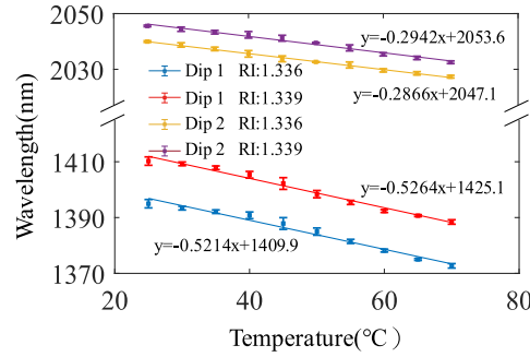
Fig. 8. Temperature sensitivities of Dip 1 and Dip 2 at RI values of 1.336 and 1.339.
