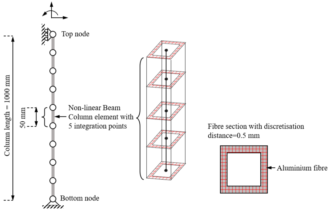
Fig. 13. Overview of the fibre element modelling (figure adapted from (Georgantzia et al. 2024) [Used with permission
