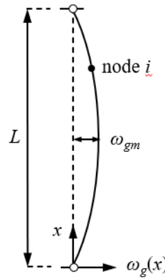
Fig. 14. Schematic of initial global imperfections of a pin-ended column (figure adapted from (Georgantzia et al. 2024) [Used with permission of American Society of Civil Engineers, from: Journal of Materials in Civil Engineering, E. Georgantzia et al., vol. 36 no. 6, 2024; permission conveyed through Copyright Clearance Center, Inc.].
