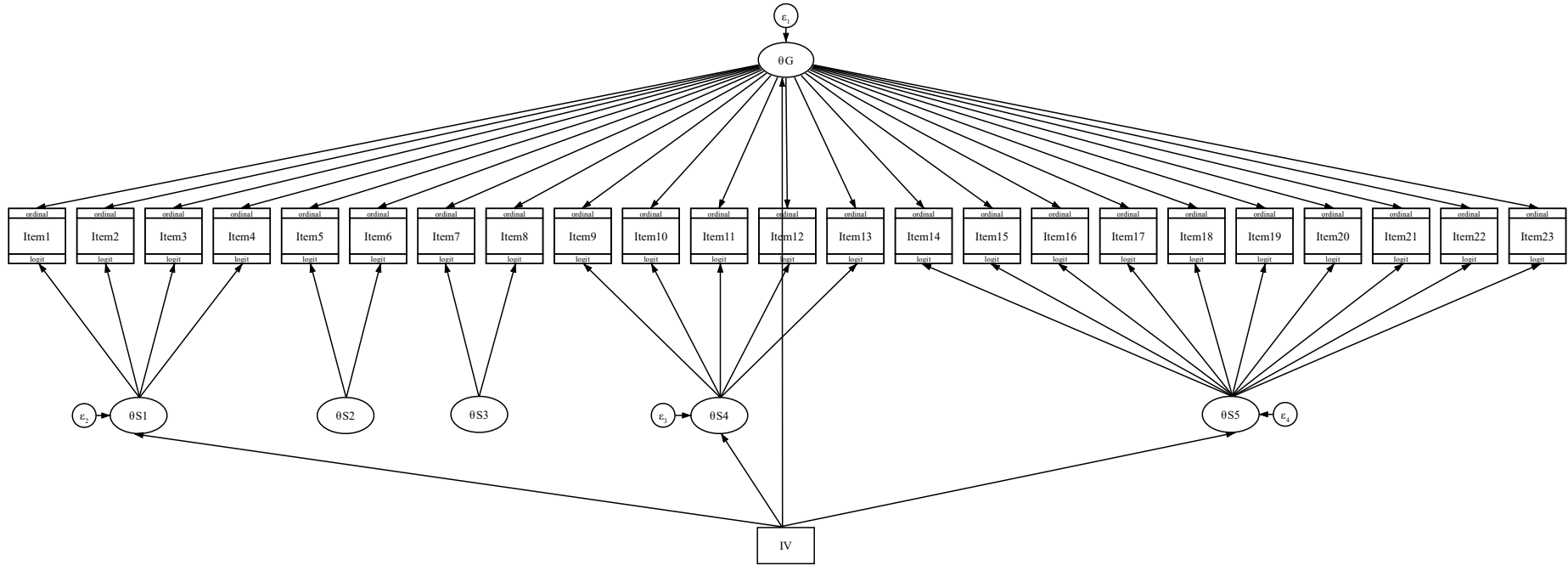
Figure 6.1: Multiple Group Graded Response Bifactor IRT Model
