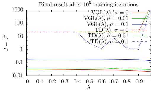
Figure 3.8: Results of VGL(\lambda) under various \lambda and noise-levels, \sigma , for solving the Vertical-Lander Problem, from a fixed trajectory start point. All results are generated for critic learning rate \alpha = 10^{-6} and actor learning rate \beta = 10^{-3} . For each value of \lambda , the graph shows the value of J - J^* after 10^5 training iterations. All results are gathered as the median result of 10 trials (i.e. from 10 different initial randomizations of the neural weights). TD(\lambda) results from Fig. 2.3 are included as dotted curves, for comparison.
