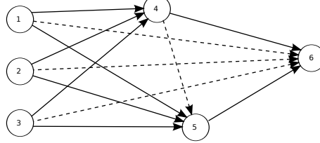
Figure 11.1: An example neural-network architecture obtainable by Alg. 11.1, with three input nodes and one output node. When all graph edges are included, we have a fully connected feed-forward neural network, with all short-cut connections. If the dotted edges are removed (for example by clamping those weights to zero) then a more traditional layered network is obtained, containing a single hidden layer of two nodes. For the purpose of this chapter, only a single output node is required, which in this example is node 6.
