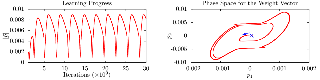
Figure 9.2: Divergence for TD(0) generated with the diverging parameters described in Section 9.3, and a learning rate of \alpha = 10^{-6} . The left-hand graph shows progress of \|\bar{p}\| versus iterations. The oscillation shown in this left graph occurs because the weight vector goes into a limit cycle after divergence. This limit cycle is shown fully in the right-hand graph, which shows the evolution of the weight vector (p_1, p_2) in phase space. The phase curve starts close to the origin (at the 'X'), then moves in the direction of the arrow, and finally finishes off in a limit cycle. The weight vector initially moves in the opposite direction from the origin, i.e. away from the target fixed point; confirming divergence.
