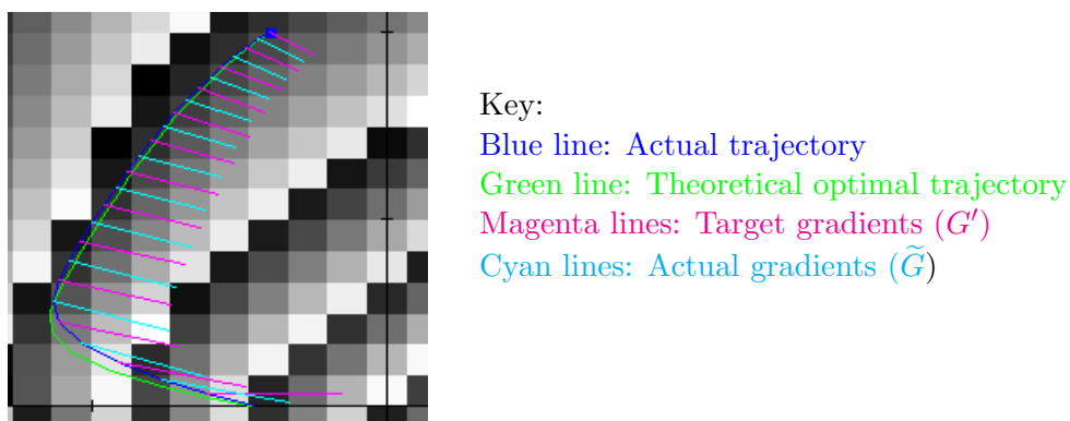
Figure 7.1: Trajectory Optimality Occurs when the Value-Gradients are Learned, under a Greedy Policy. This picture, repeated from Fig. 3.6, shows the key fact motivating VGL methods compared to VL methods: Merely learning the target value-gradients, under a greedy policy, will necessarily bend the trajectory into a locally extremal or locally optimal shape. Hence this picture concisely illustrates the trajectory-optimality principle of VGL, which is proven for deterministic environments in this chapter.
