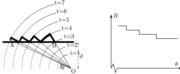
Figure 10.2: An Example of the Problems that Can Occur when Clipping is Not Used. The left figure shows that spurious zigzag boundary penetrations can occur when clipping is not used. The right figure shows a corresponding graph of R , the trajectory length, versus \theta , and this yields no useful local gradient information. Hence minimising R with respect to \theta using only dR/d\theta would be impossible.
