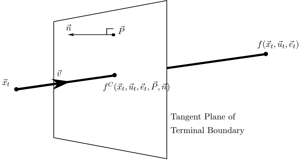
Figure 10.4: The Final State Transition of a Trajectory Crossing the Tangent Plane of a Terminal Boundary. The unclipped line goes from \vec{x}_t to f(\vec{x}_t, \vec{u}_t, \vec{e}_t) . The line intersects the plane at a point given by the new clipped model function f^C(\vec{x}_t, \vec{u}_t, \vec{e}_t, \vec{P}, \vec{n}) .
