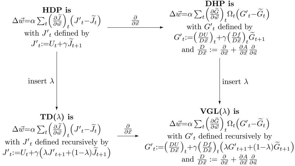
Figure 1.1: Relationship of VGL( \lambda ) to other ADPRL algorithms.
