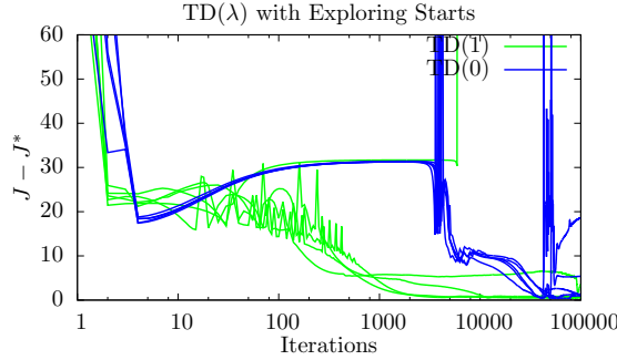
Figure 2.4: Results for Using Exploring Starts to Solve the Vertical-Lander Problem by TD(\lambda) . The graph shows the trajectory cost averaged over 10 trajectories with fixed start points. Each curve shows a different experimental trial (i.e. different weight initialisation); five different significant trials for TD(1) and five trials for TD(0) . In this experiment, both algorithms make significant progress in solving the problem. (For comparison to VGL methods, see also Fig. 3.9.)
