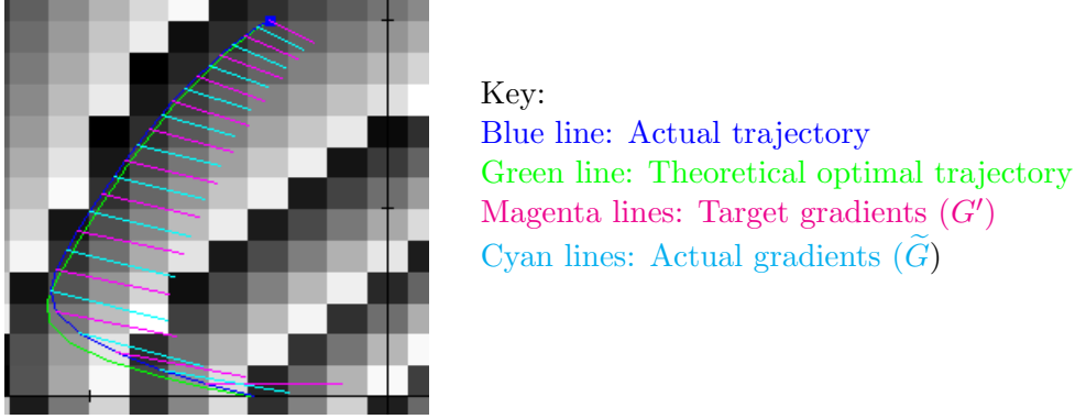
Figure 3.6: Trajectory Optimality under a Greedy Policy, for Value-Gradient Learning. This diagram shows the value gradients, \tilde{G} , matching their targets, G'_t , well (the lines \tilde{G} match the lines G' closely in magnitude and direction). Consequently the trajectory (the blue curve) matches the optimal trajectory (the green curve). This fact, that simply learning the target value gradients exactly will produce a locally extremal or optimal trajectory, is a key motivating theorem for VGL, and is proven in Chapter 7 for deterministic environments. In this diagram, the grey-scale background indicates the magnitude of the critic function at each point in state space. The grey scale has changed significantly from the VL-learned value-function shown in Fig. 3.1, since now the value-gradients have been learned successfully. Note that the white bands are not discontinuities in this figure; it is just that the graph plotter ran out of colours and wrapped around from white to black again.
