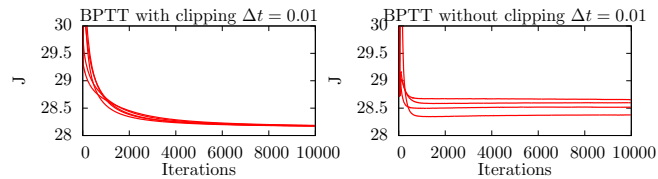
Figure 10.7: Vertical Lander with \Delta\tau = 0.01 .
