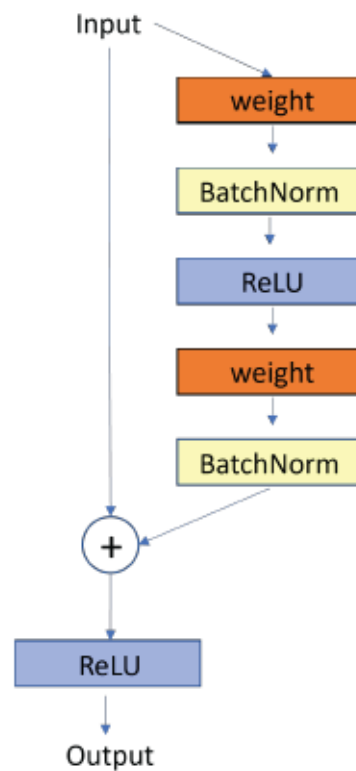
Fig. 2.4 ResNet Block as described in the original introduction by He et al. [4]. The residual layer or block contains two weight layers, in this case, convolutional layers. The input of the block is saved and then added to the output of the batch normalisation of the second convolutional layer right before its activation layer.
