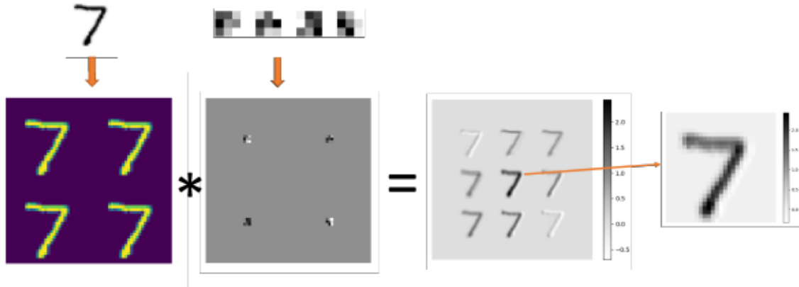
Fig. 2.12 Experimental results of the channel tiling technique applied to four input channels of MNIST digit "7" as input and four kernels corresponding to one output channel extracted from the model also trained on MNIST. The input image is padded and tiled four times (each corresponding to the kernel). Kernels are also padded and tiled into one kernel block. Convolution has been performed with both blocks, and the image in the middle of the output is cropped out. The cropped-out image is the sum of the convolutions of inputs with 4 kernels.
