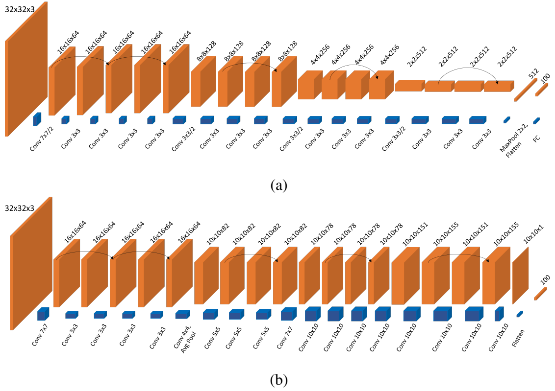
Fig. 3.7 The comparison between our tweaked ResNet-18 used for CIFAR-100 training and FatNet, which is built on ResNet-18 and specifically designed for CIFAR-100 classification. (a) ResNet-18 architecture is slightly altered in our version. Our model does not employ strides, given that optical systems are unable to carry out strides in convolutions. Moreover, to enhance compatibility with CIFAR-100, we've omitted the second non-residual convolutional layer. (b) FatNet, which is based on ResNet-18, is tailored for CIFAR-100. This structure has fewer channels but larger resolutions when compared to ResNet-18. The kernel sizes can reach up to 10 \times 10 , and feature maps are never pooled to smaller than 10 \times 10 . The concluding layer is a 10 \times 10 matrix that is flattened into a 100-element vector, with each element representing a CIFAR-100 class.
