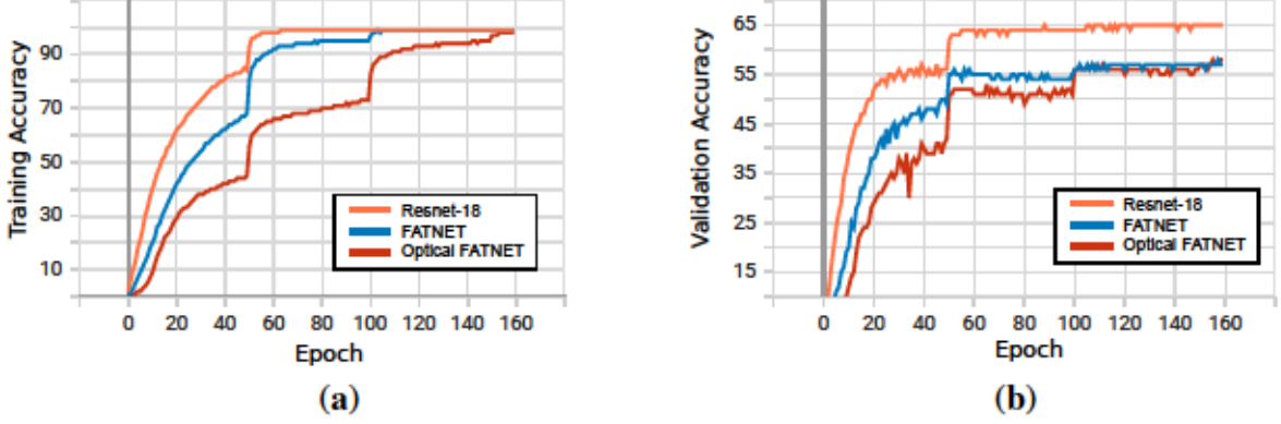
Fig. 3.12 Comparison of training and validation accuracies per epoch for each model used in the experiment. The steep jumps can be seen every 50 epoch due to the learning rate update by a scheduler. (a) The ResNet-18, Res-FatNet, and the Optical simulation of Res-FatNet all accomplished a training accuracy of 99%, with ResNet-18 achieving it in fewer epochs. Conversely, the optical simulation took longer to train due to the complex computation needed to simulate light propagation. (b) As for validation accuracy, ResNet-18 reached up to 66%, while Res-FatNet could not exceed 60% for both validation and testing, despite its fewer convolutional operations.
