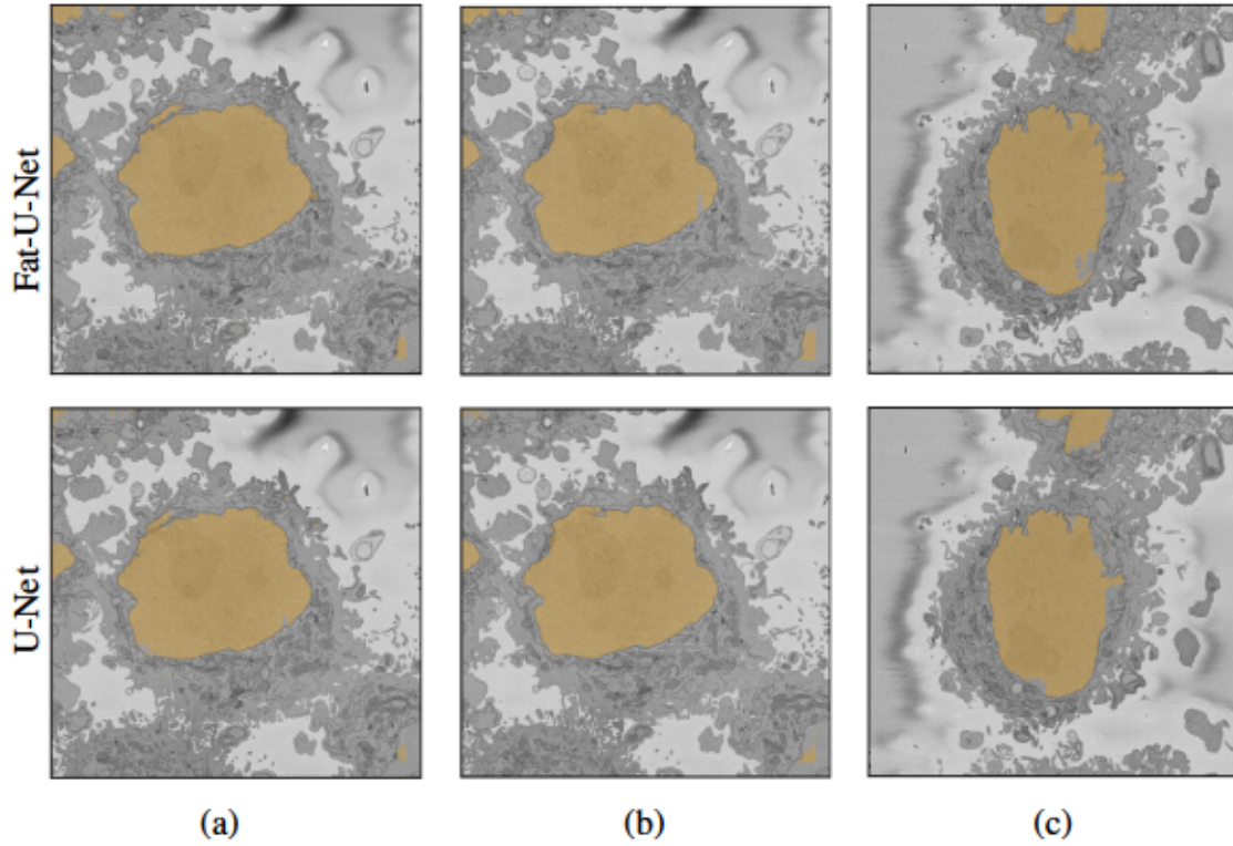
Fig. 4.6 Qualitative results of HeLa dataset. (a) train slice 119 (b) test slice 121 (c) Unseen cell, taken from the larger field.
