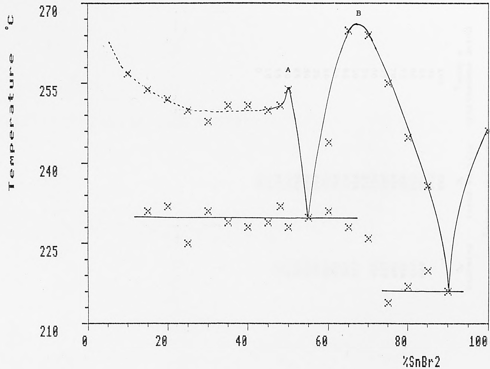
Fig. 3.8. Phase diagram for KBr : SnBr 2 system
