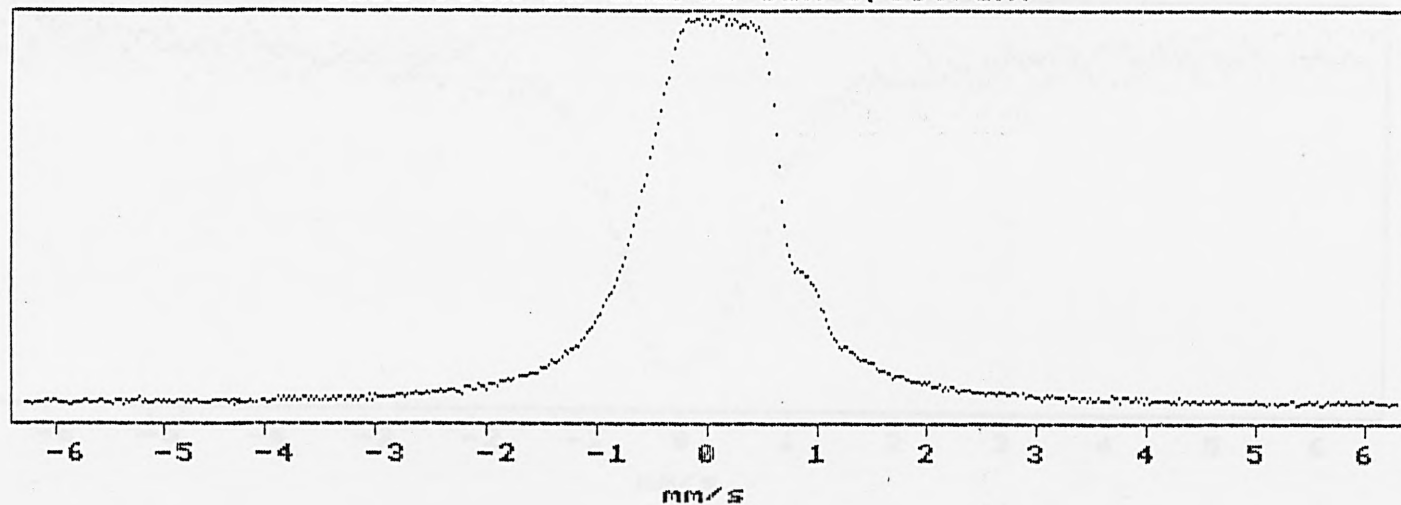
Fig.4.33 SnO 2 film on Quartz CEM spectrum.
