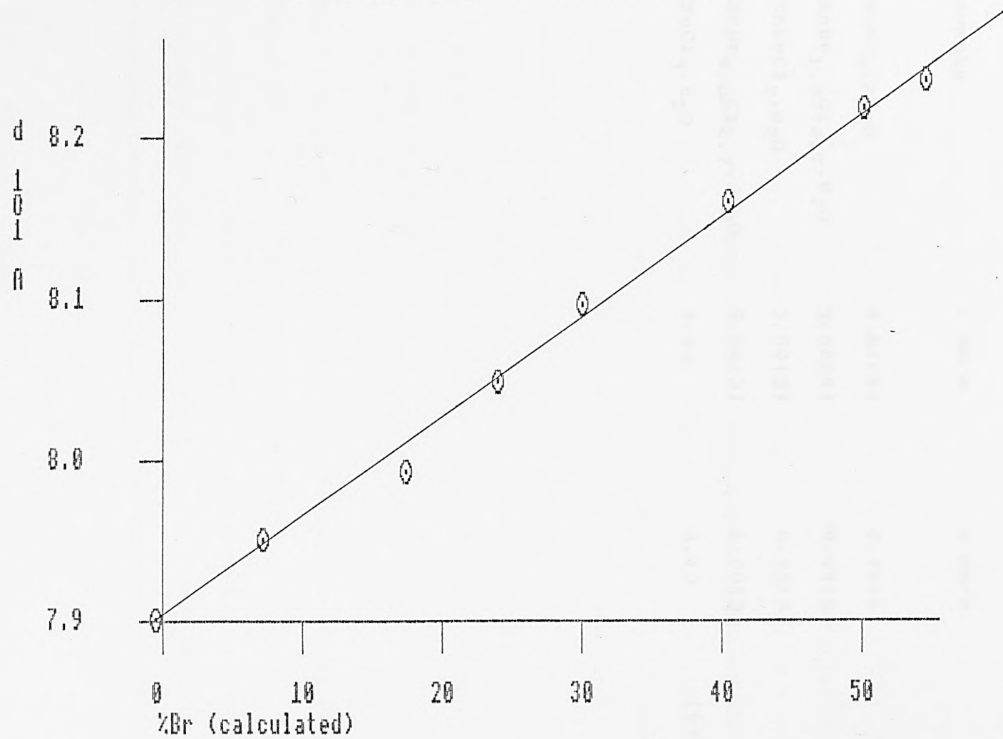
Fig.2.12 Lattice expansion in \text{KSnBrnC13-n.xH2O}
