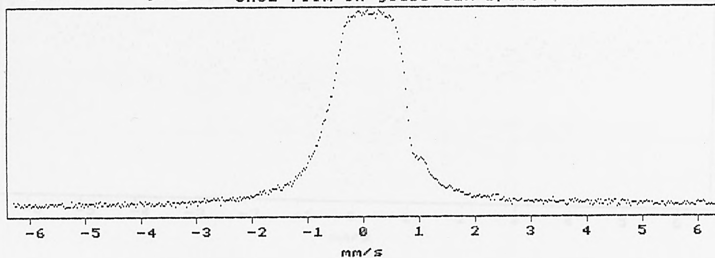
Fig.4.32 50 \Omega/\text{cm}^2 SnO 2 film on glass CEM spectrum.
