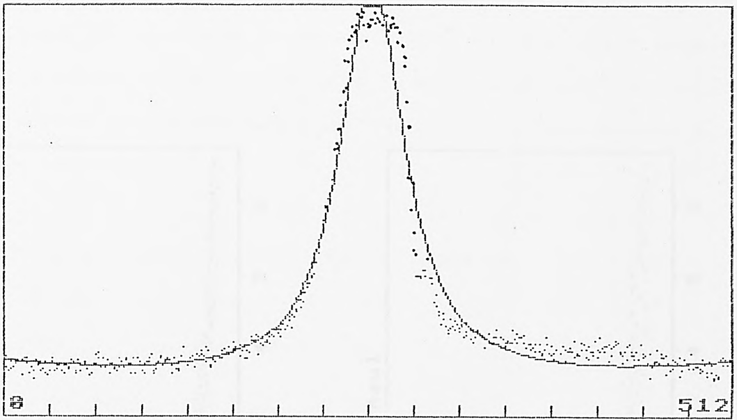
Fig.4.16: Single line fit to calibration spectrum
