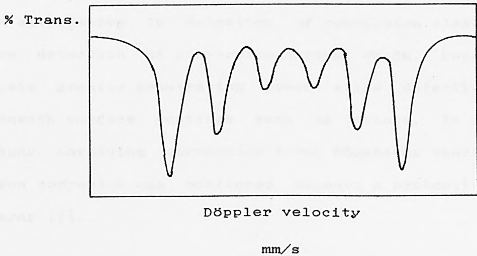
Fig.4.10 Magnetically split Mössbauer spectrum
