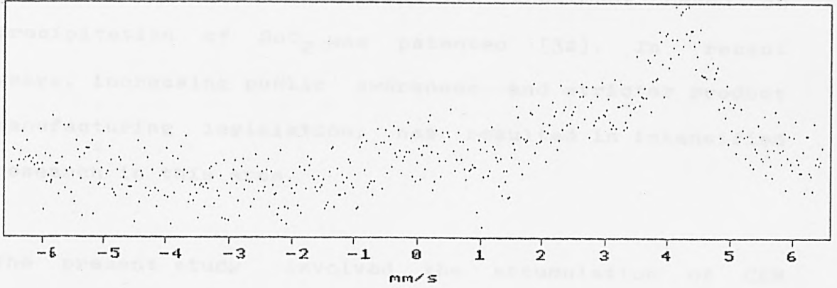
Fig.4.38e CsSn3Br1.5F5.5 CEM spectrum of fresh sample
