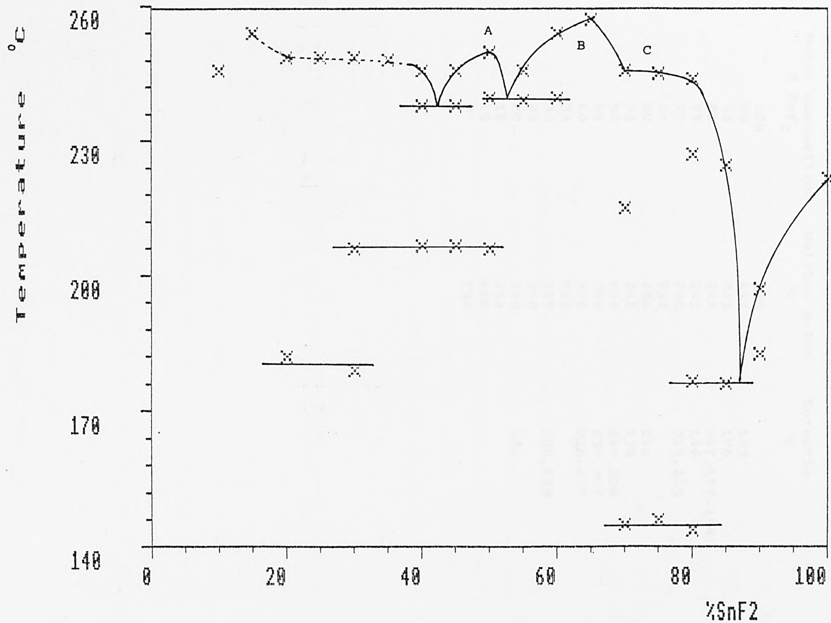
Fig. 3.17. Phase diagram for KBr : SnF 2 system
