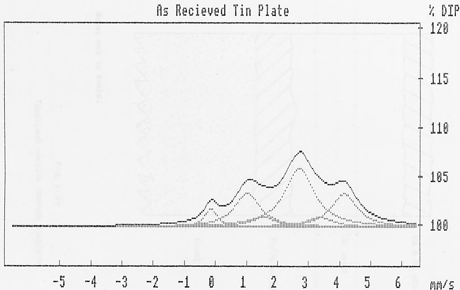
Fig.4.26: Computer simulation, based on fitted parameters, of the component lines in the 'as-received' tinplate spectrum.
