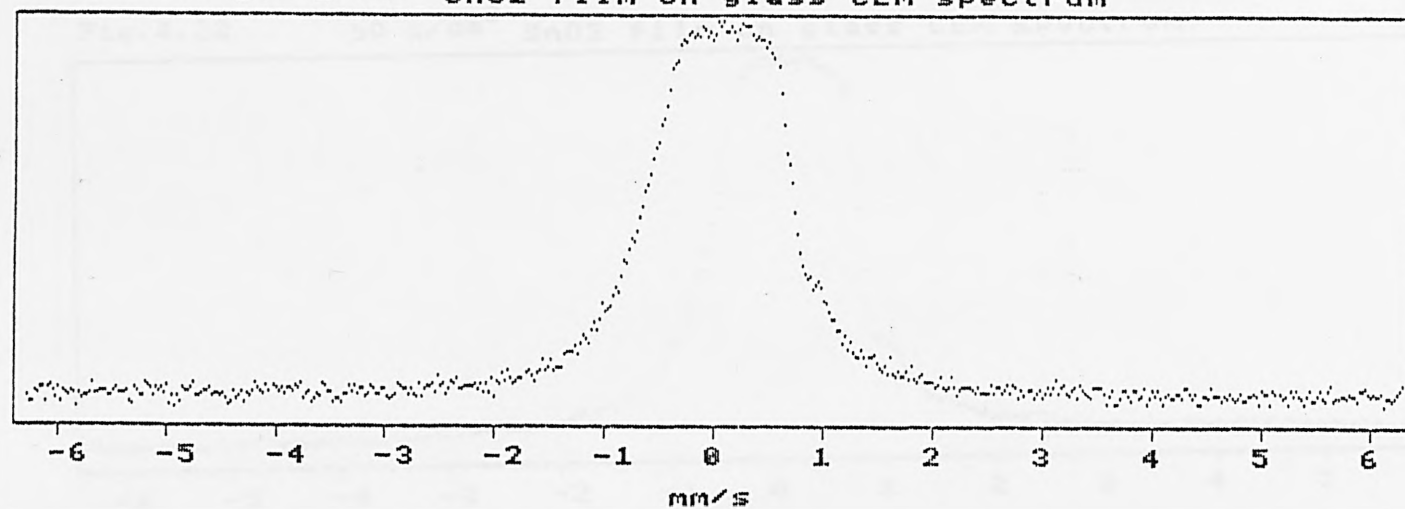
Fig.4.30 500 \Omega/\text{cm}^2 SnO 2 film on glass CEM spectrum
