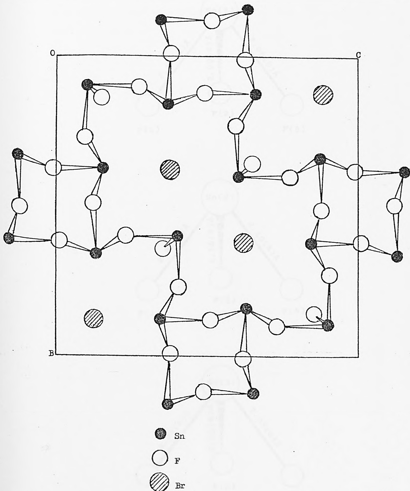
Fig.5.19: Projection onto (100) of \text{Sn}_3\text{BrF}_5
