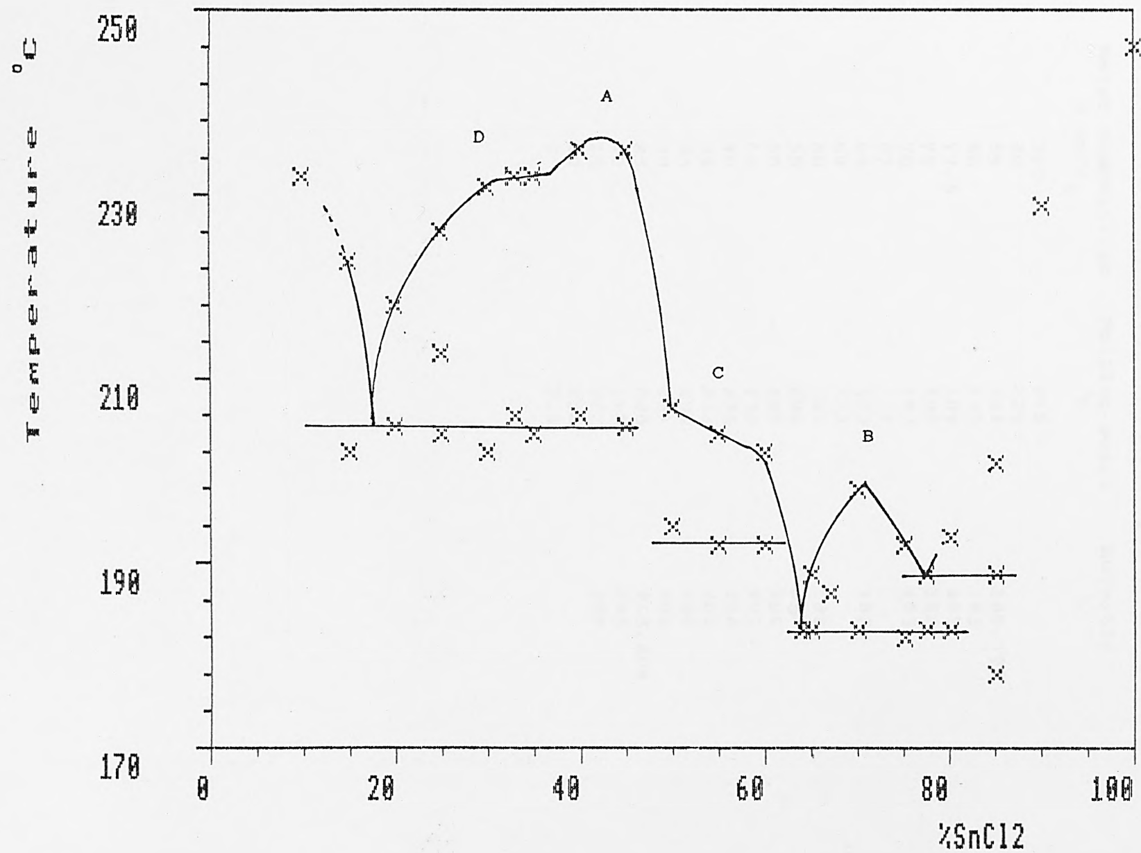
Fig. 3.13. Phase diagram for KBr : SnCl 2 system
