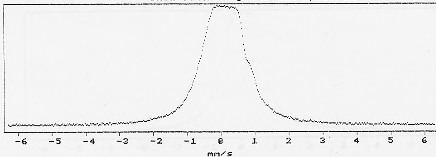
Fig.4.31 200 \Omega/\text{cm}^2 SnO 2 film on glass CEM spectrum
