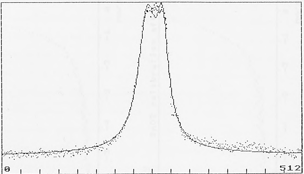
Fig.4.17: Doublet fit to calibration spectrum
