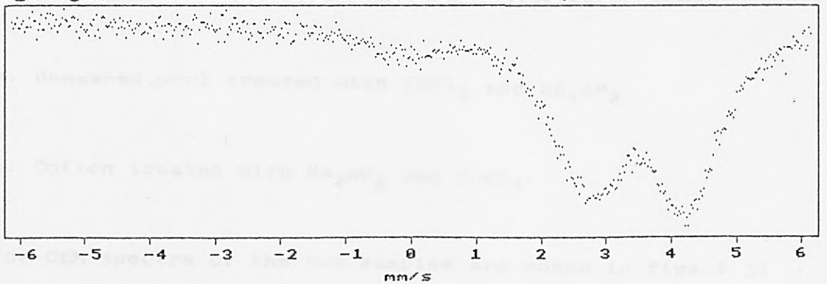
Fig.4.38f CsSn3Br1.5F5.5 86K transmission spectrum
