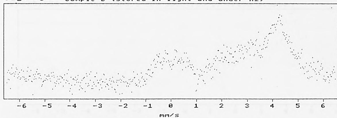
Fig.4.38b Sample b (stored in light and under N 2 )
