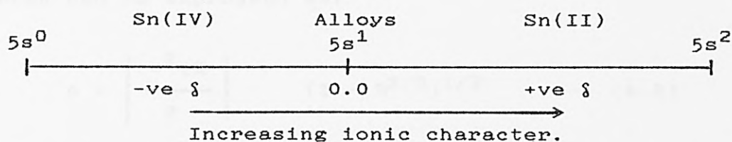
Fig.4.6: Variation of \delta in Sn materials wrt \alpha -Sn.
