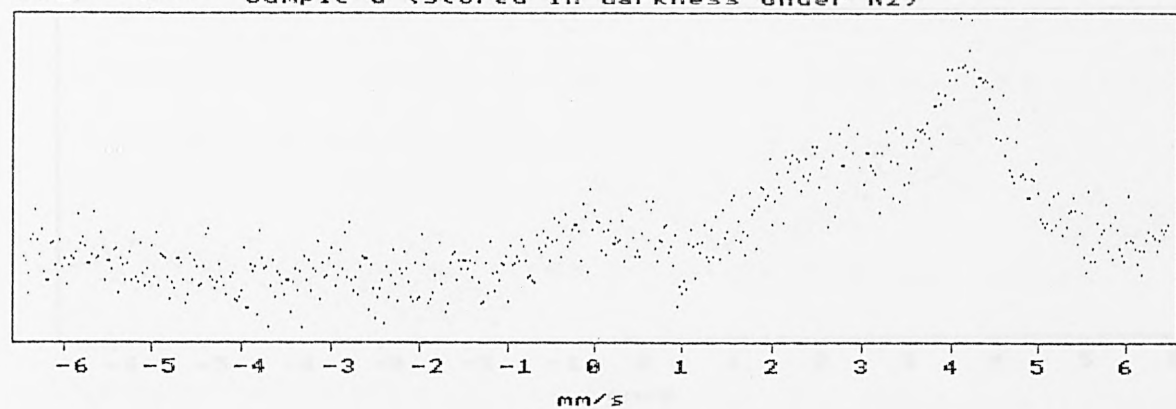
Fig.4.38a Sample a (stored in darkness under N 2 )
