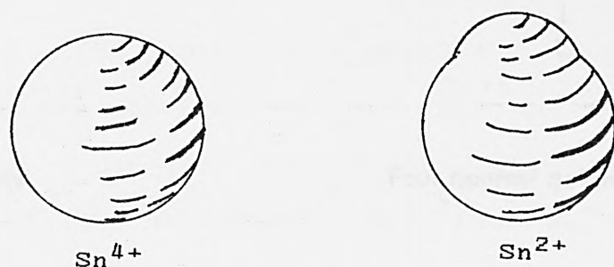
Fig.1.4 Electron density around tin ions.
