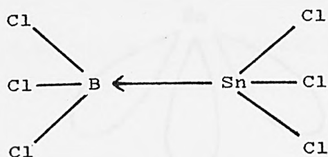
Fig.1.10 \sigma - donation by SnCl_3^-
