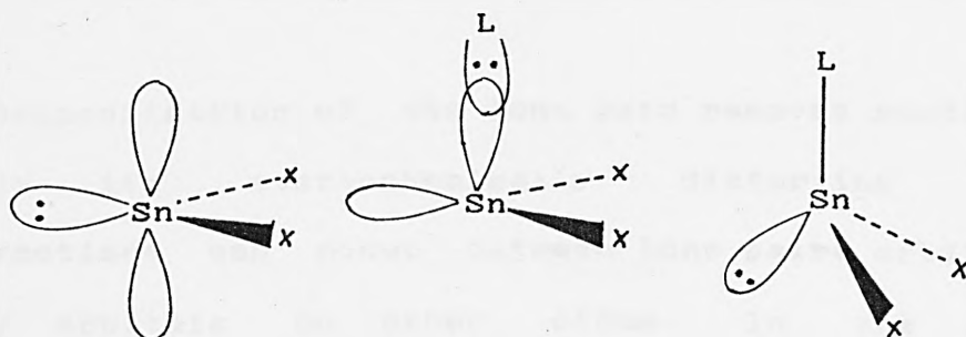
Fig.1.8 sp^2 \rightarrow sp^3 hybridisation in complex formation.
