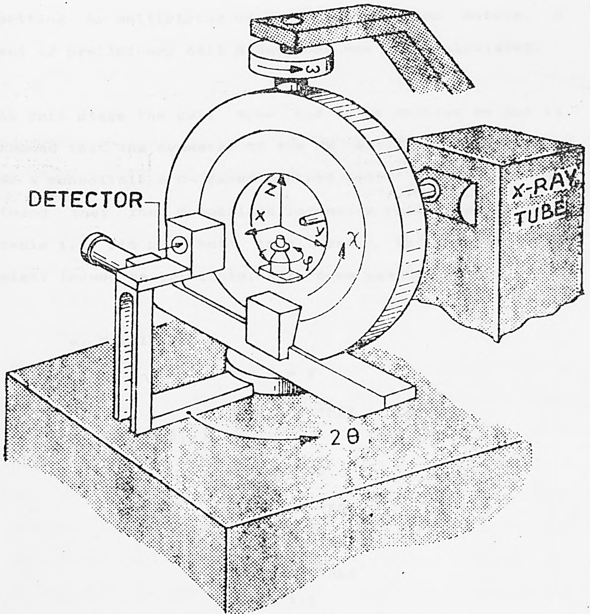
Fig. 1.17: Definition of angles and coordinates on four circle diffractometers.
