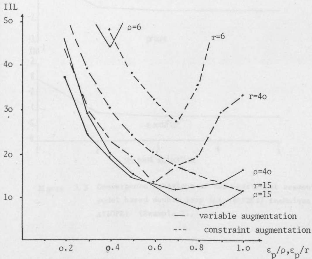
Figure 7.2 Sensitivity to \epsilon_p of model based double loop (MBDL1) technique (Example 1).
