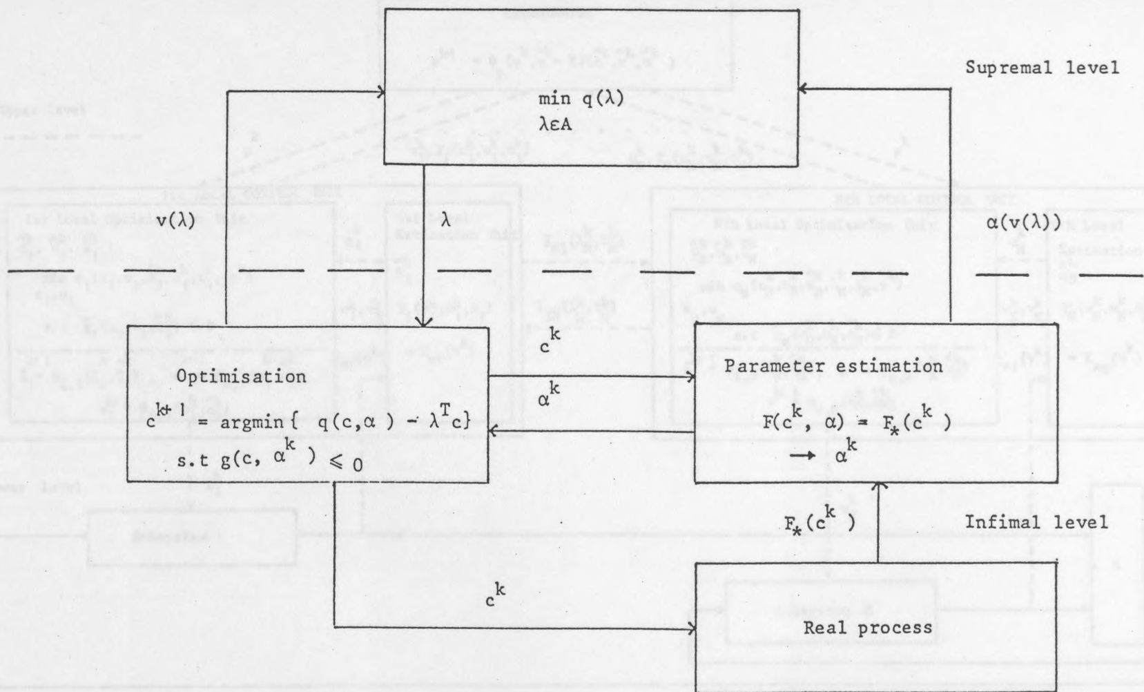
Figure 3.2 Two - level type algorithm.
