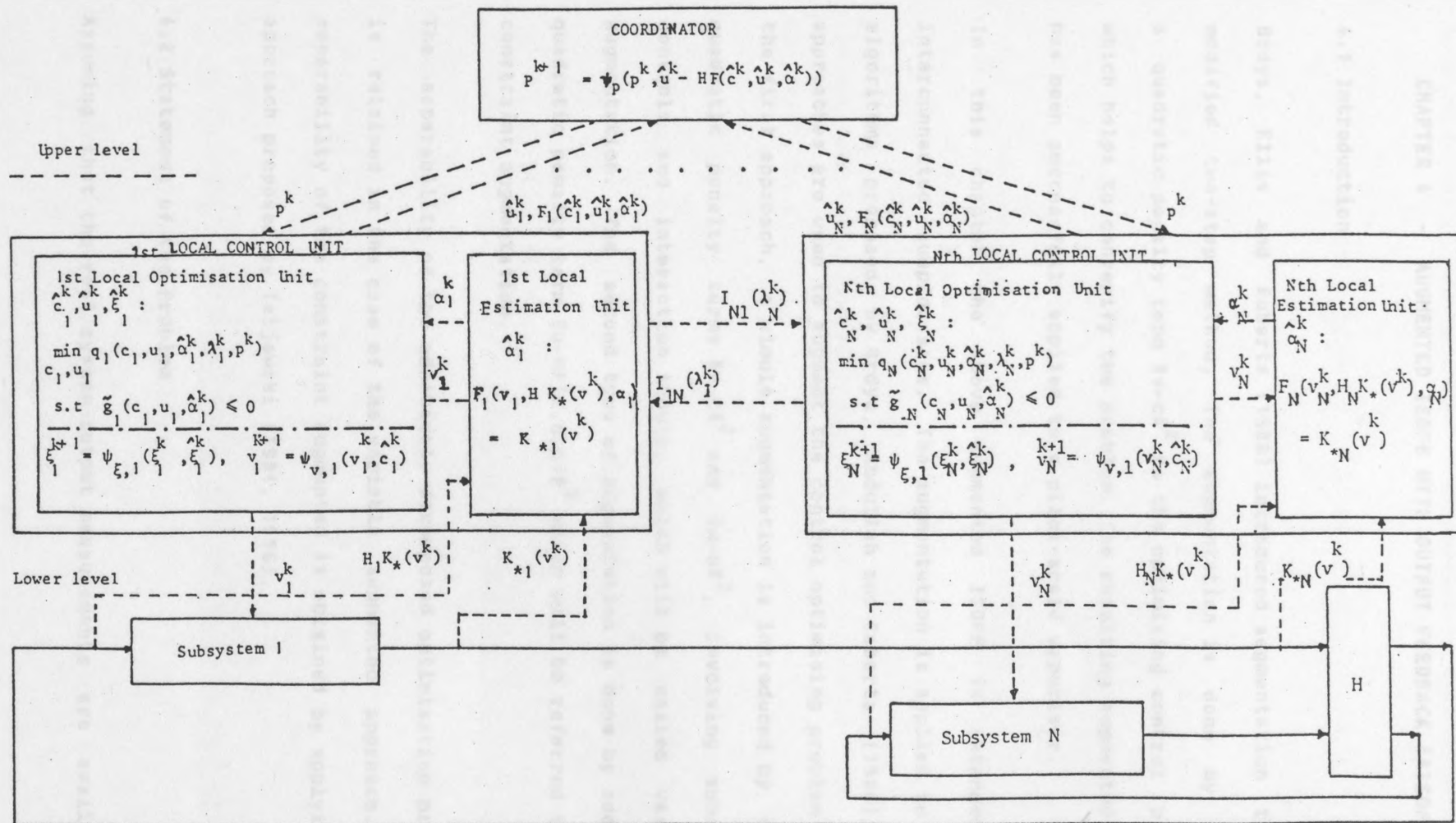
Figure 3.4 A two-level structure with input-output information feedback.
