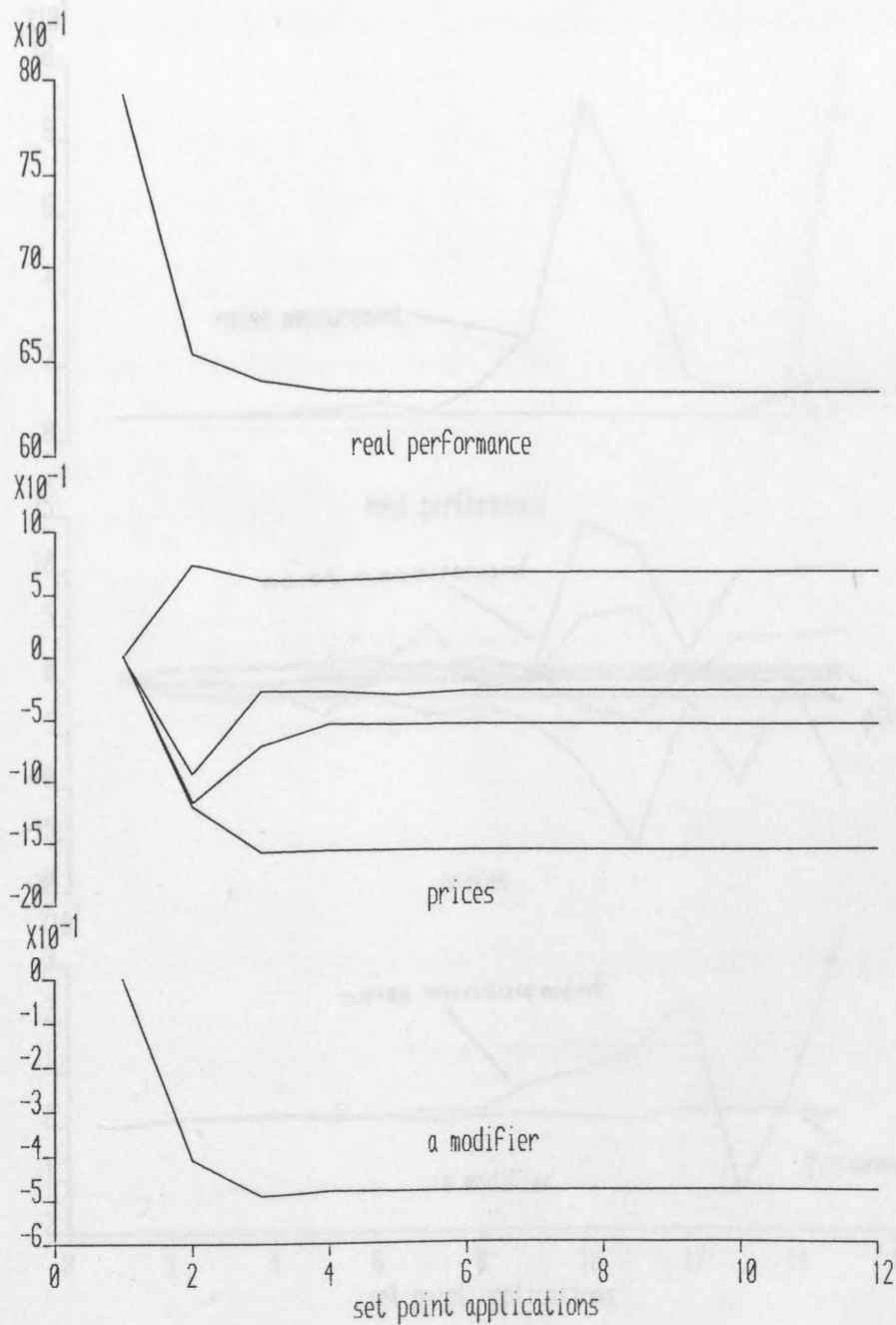
Figure 7.4 Convergence behaviour of the variable augmented model based double loop (VA - MBDL2) technique of AISOPE2 (Example 2).
