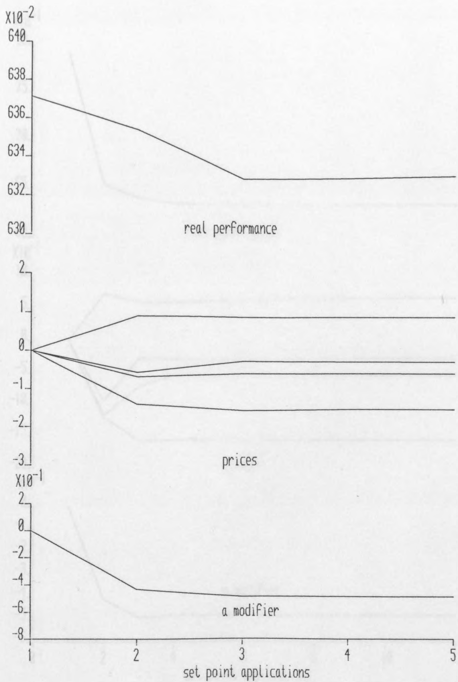
Figure 7.3 Convergence behaviour of the constraint augmented model based double loop (CA-MBDL1) technique of AISOPE1 (Example 2).
