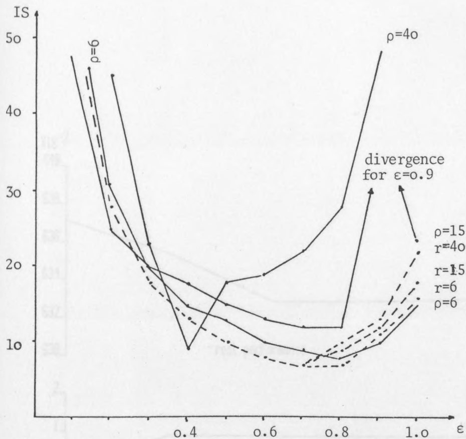
Figure 7.1 Sensitivity to \epsilon of model based double loop (MBDL1) techniques (Example 1).
