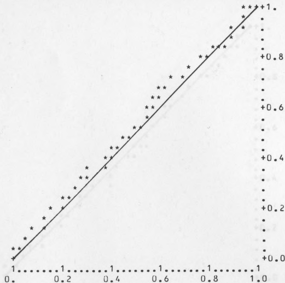
FIG.5.26. D y-plots, data in Table 5.2, the plots based on the line printer output.
