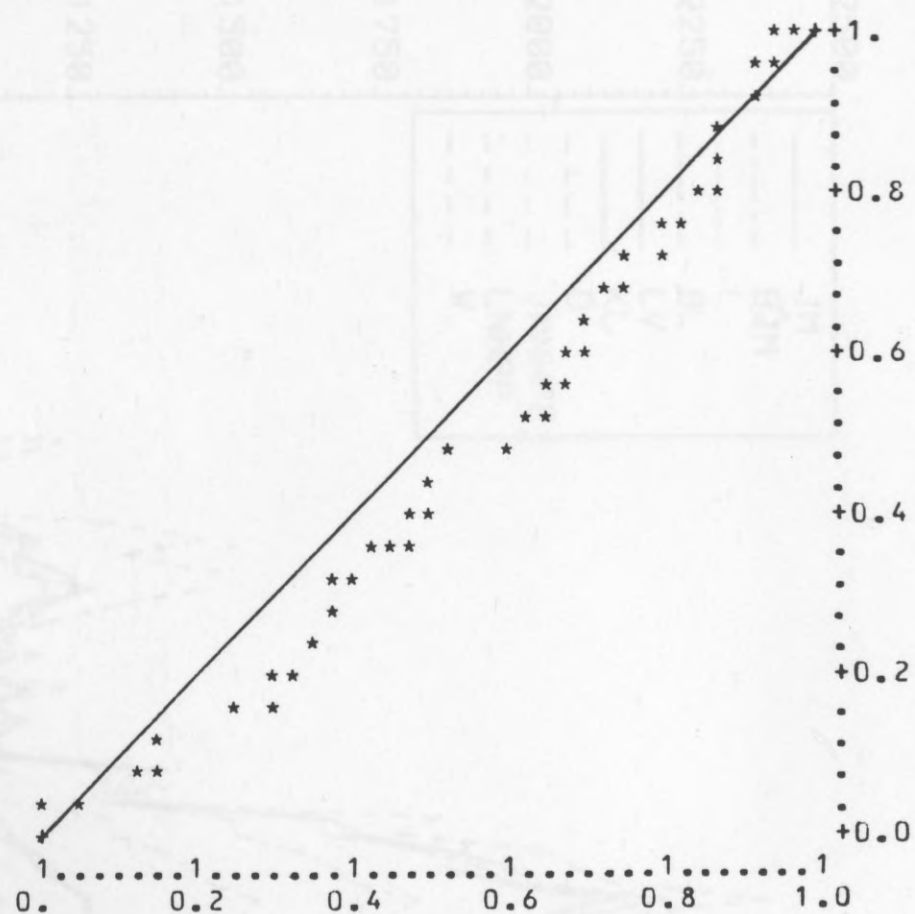
FIG.5.20. KL u-plots, data in Table 5.2, the plots based on the line printer output.
