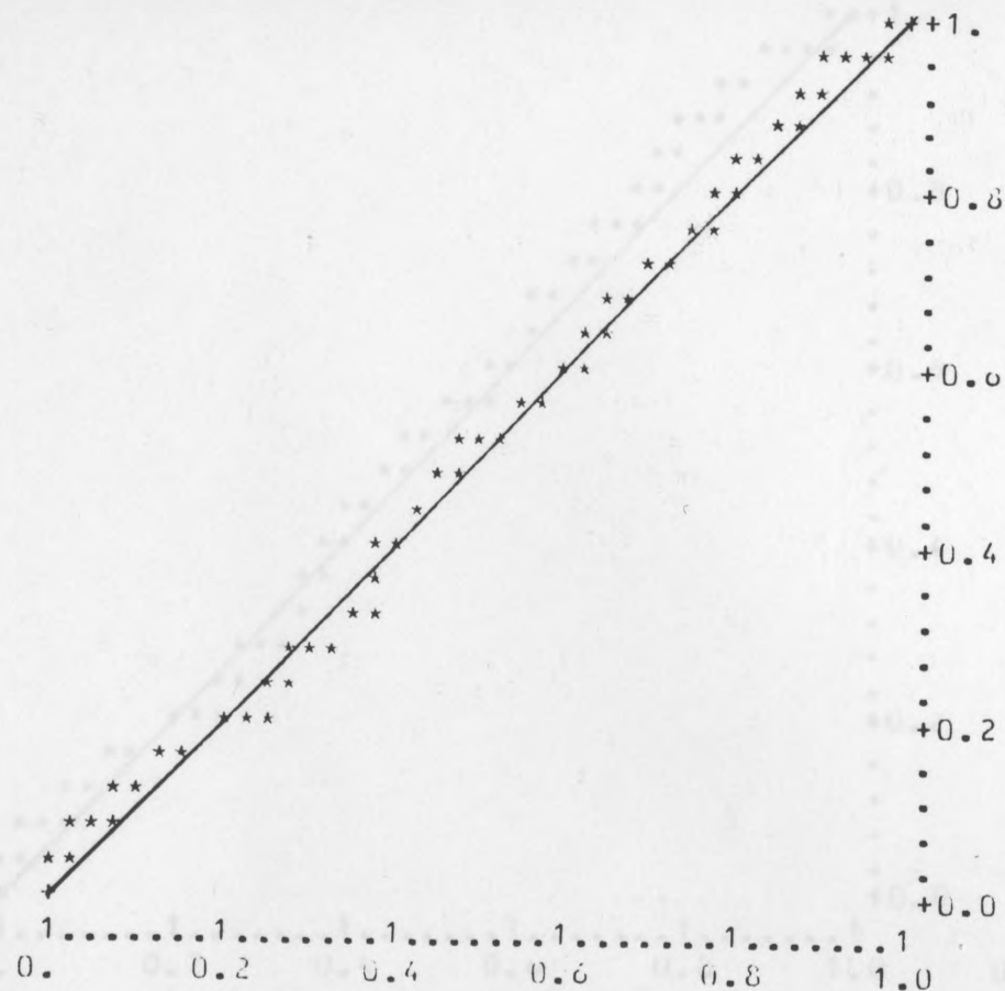
FIG. 5.49. BJM y-plots, data in Table 5.4, the plots based on the line printer output.
