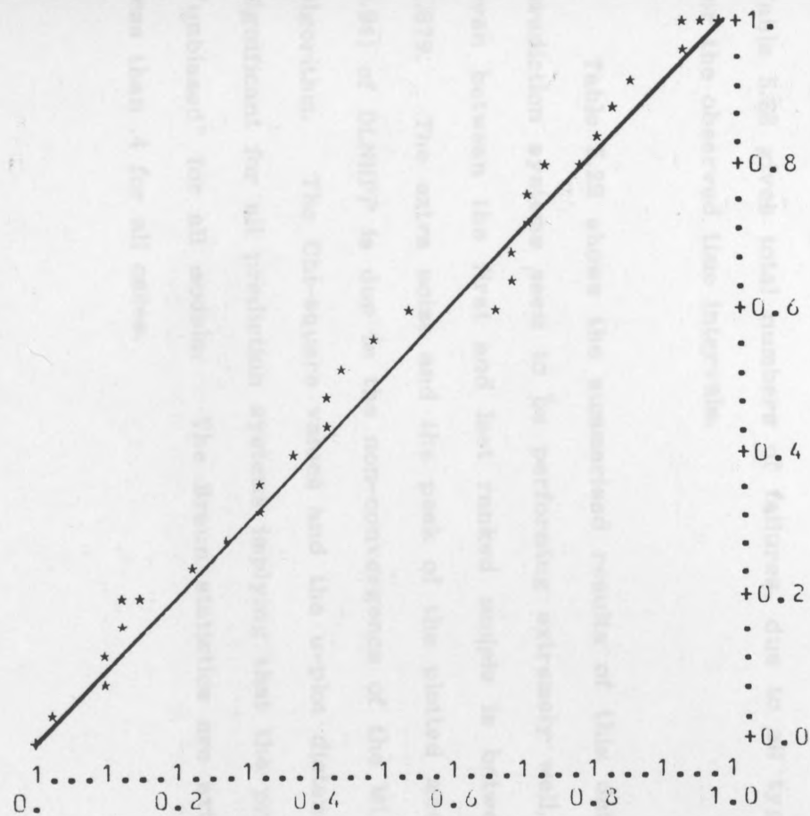
FIG.5.93. DKL u-plots, data in Table 5.25, the plots based on line printer output.
