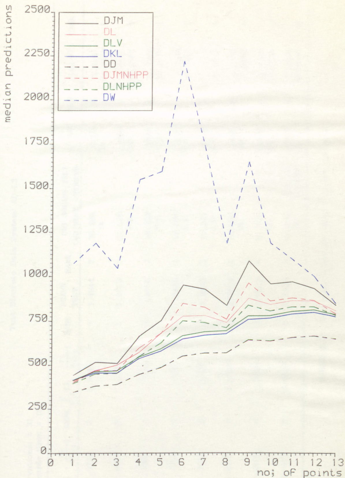
FIG.5.97. The plots of predictive median time to 1st Failure in each prediction interval for system L3 data(AD-L3)
