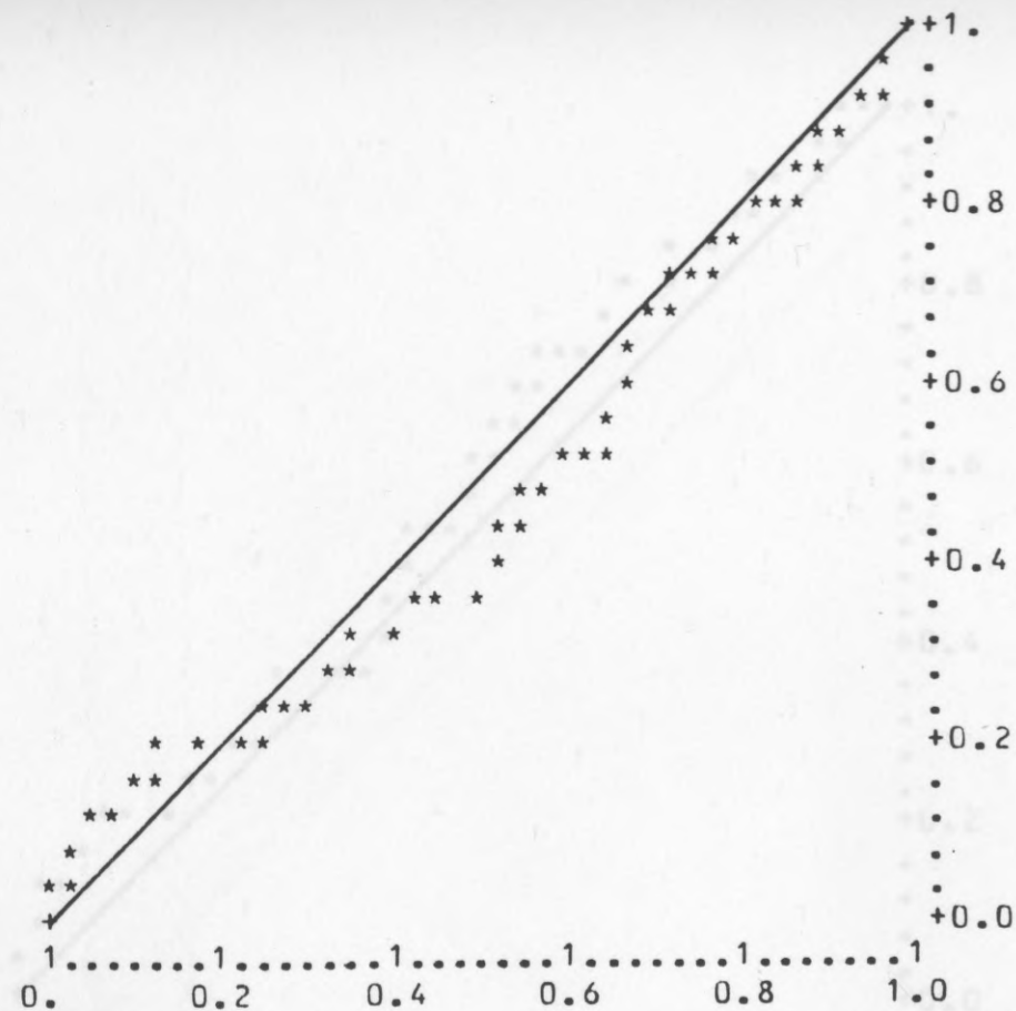
FIG.5.8. D u-plots, data in Table 4.1, the plots based on the line printer output.
