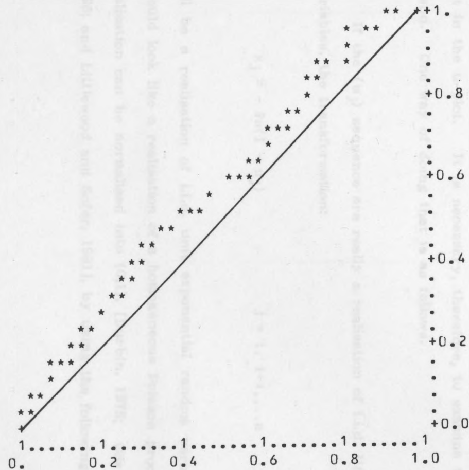
FIG.4.4. LV y-Plots, data of Table 4.1, the plots based on the line printer output.
