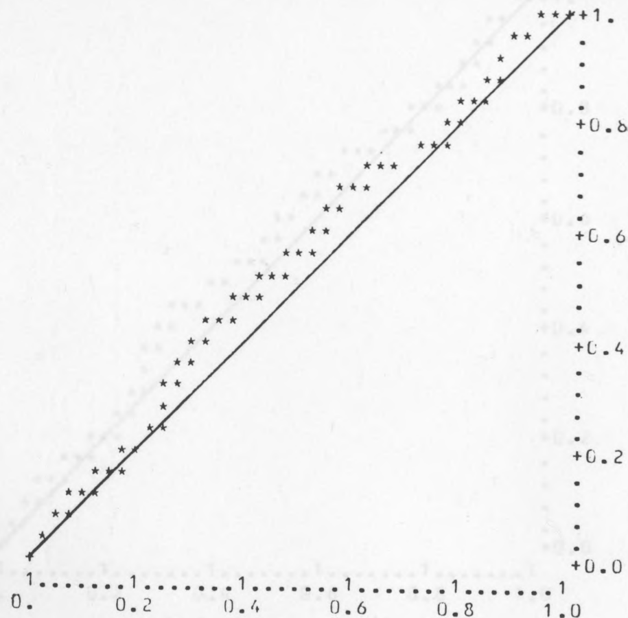
FIG. 5.48. BJM u-plots, data in Table 5.4, the plots based on the line printer output.
