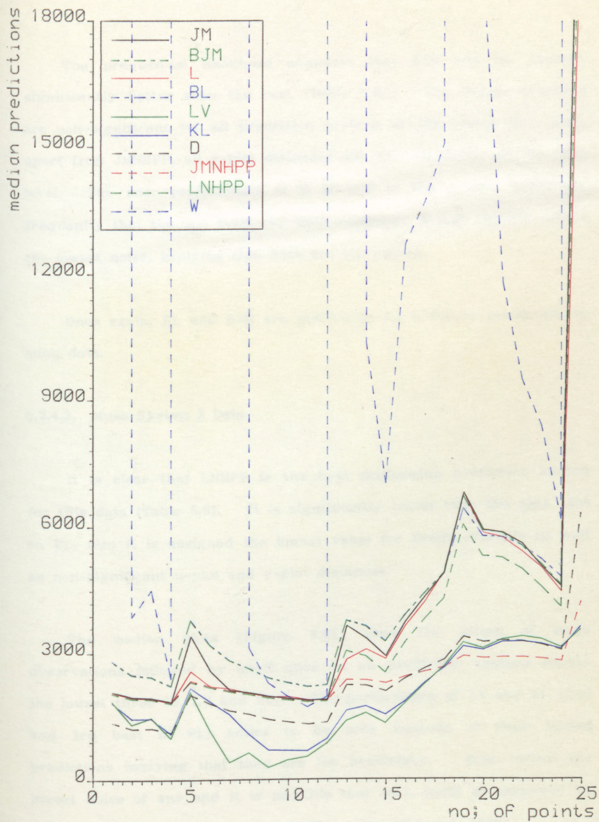
FIG.5.61. The plots of predictive medians for Musa's system 17 data
