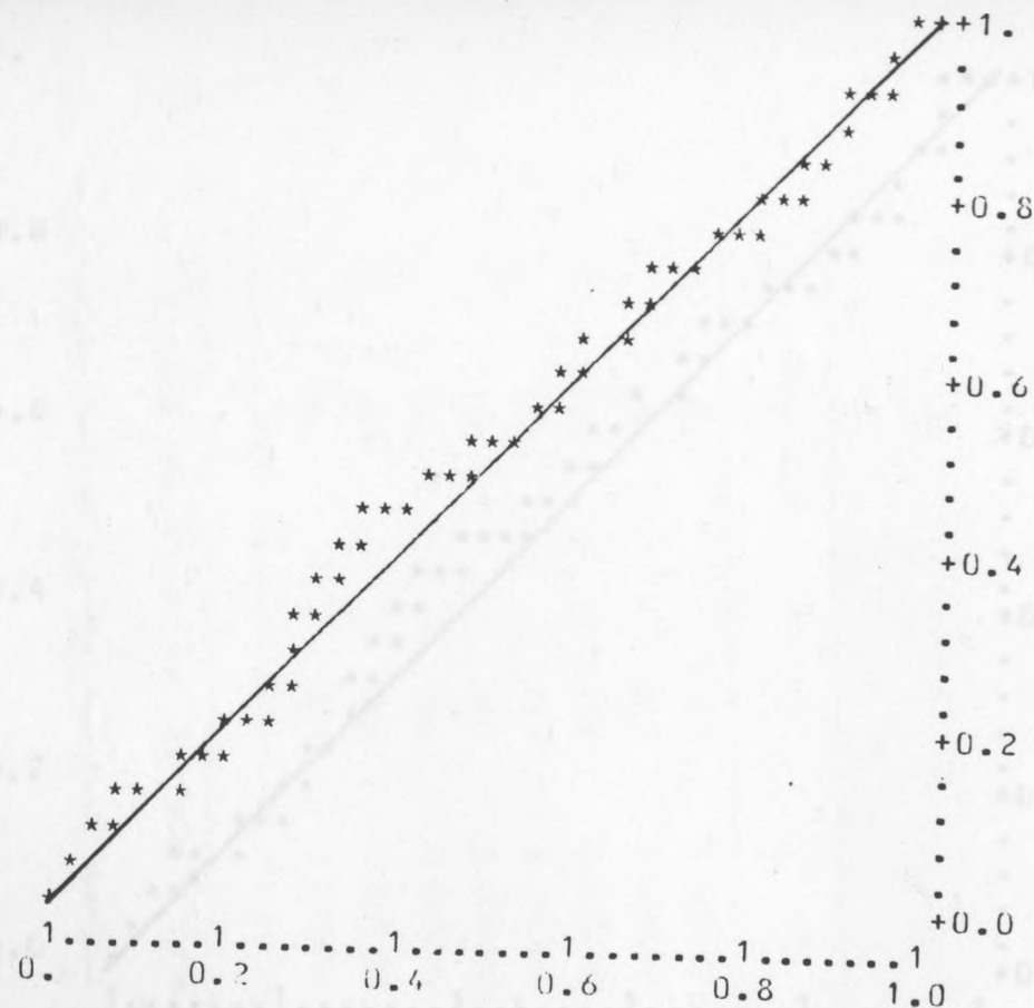
FIG. 5.56. LNHPP u-plots, data in Table 5.4, the plots based on the line printer output.
