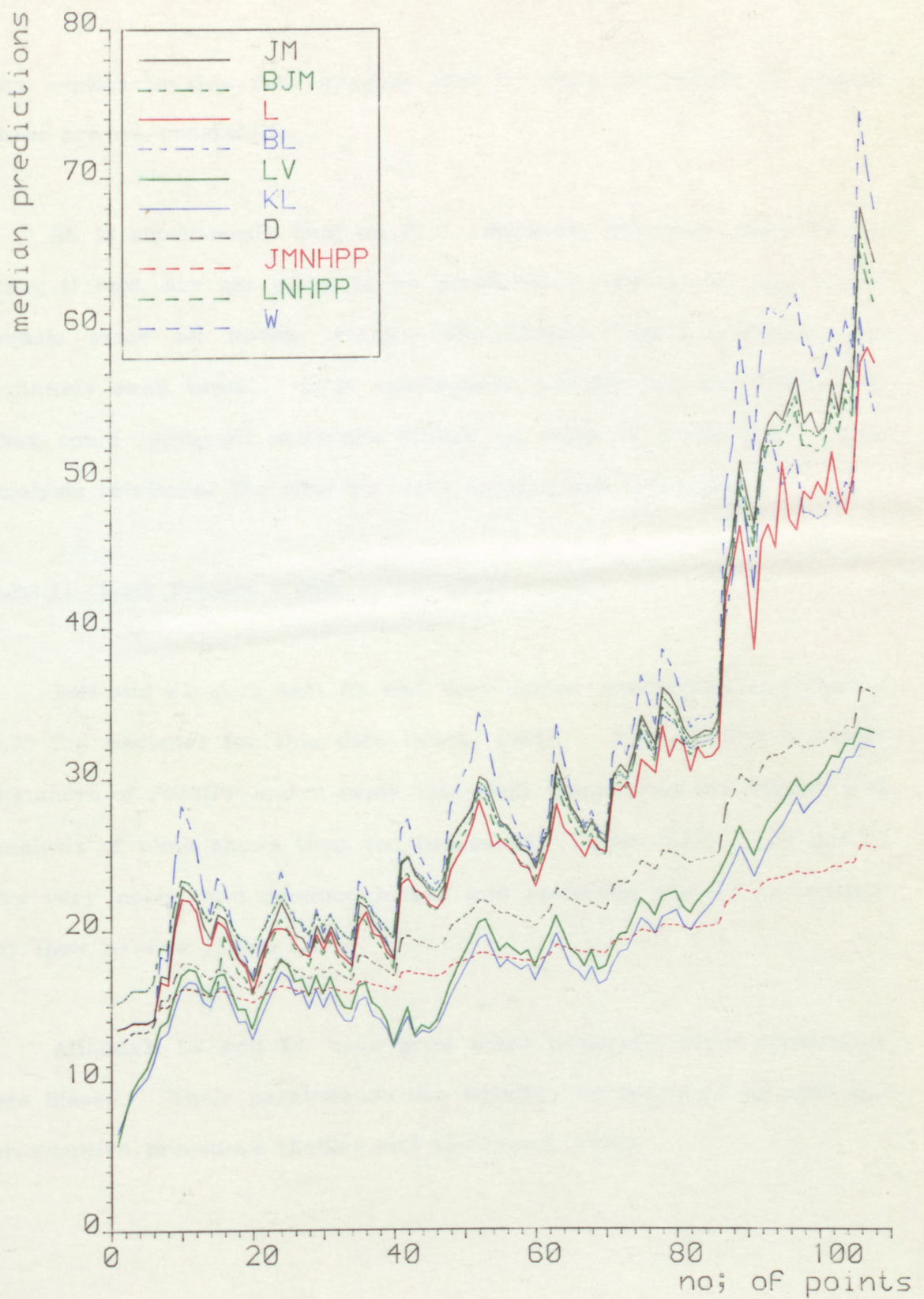
FIG.5.69. The plots of predictive medians for system SYSEN data
