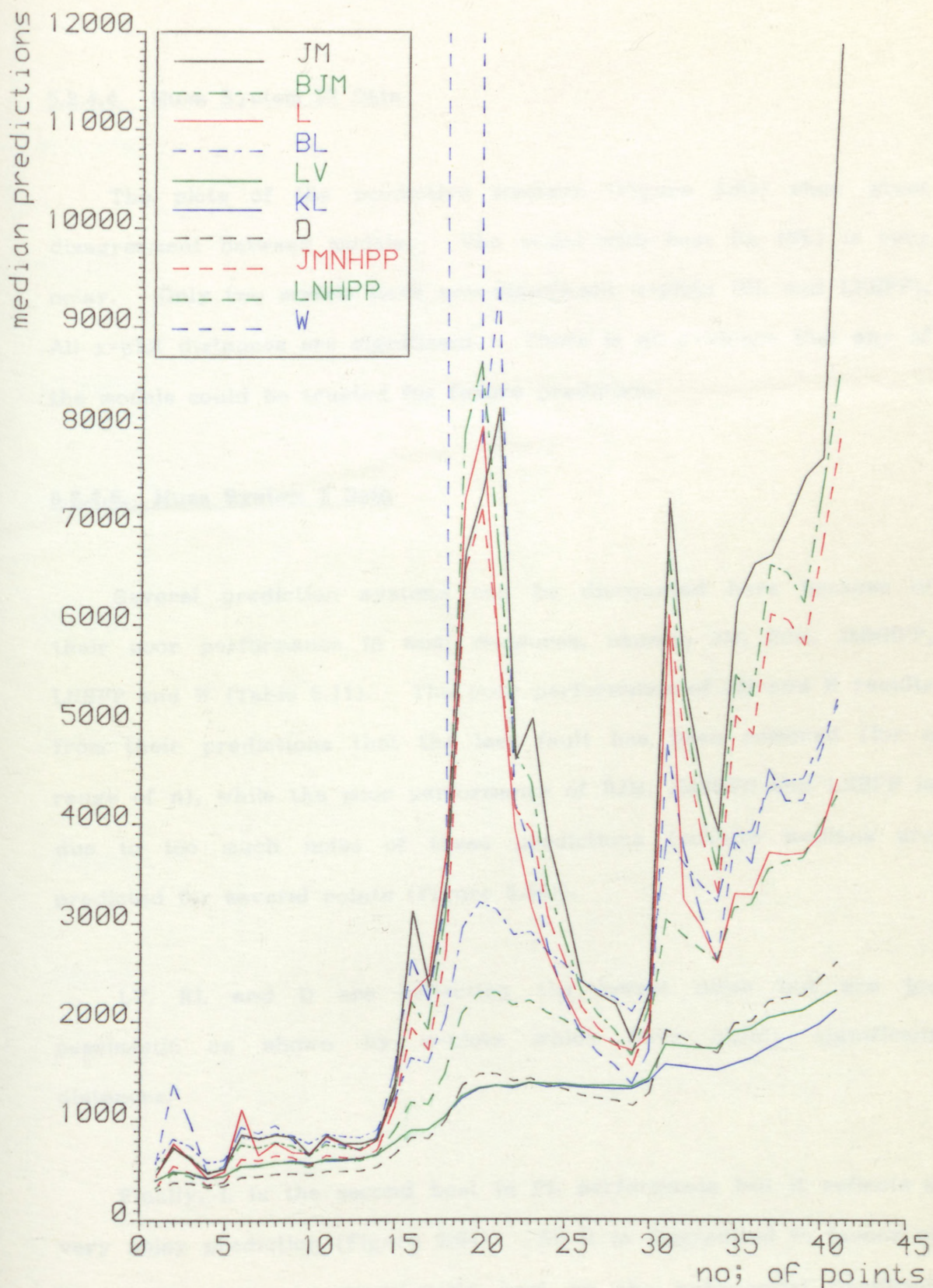
FIG.5.62. The plots of predictive medians for Musa's system 2 data
