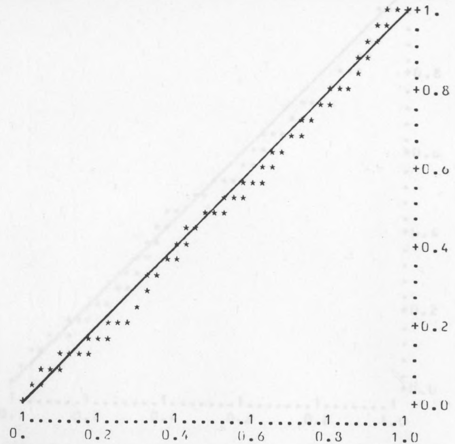
FIG. 5.42. KL u-plots, data in Table 5.4, the plots based on the line printer output.
