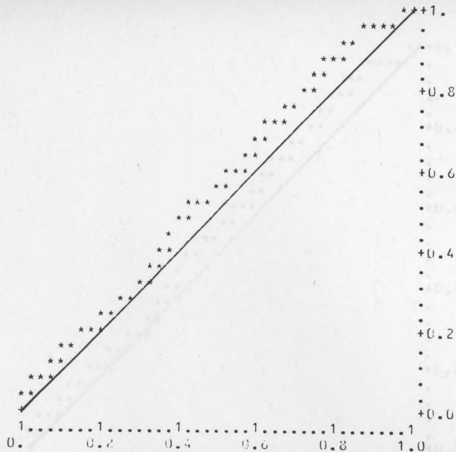
FIG. 5.41. LV y-plots, data in Table 5.4., the plots based on the line printer output.
