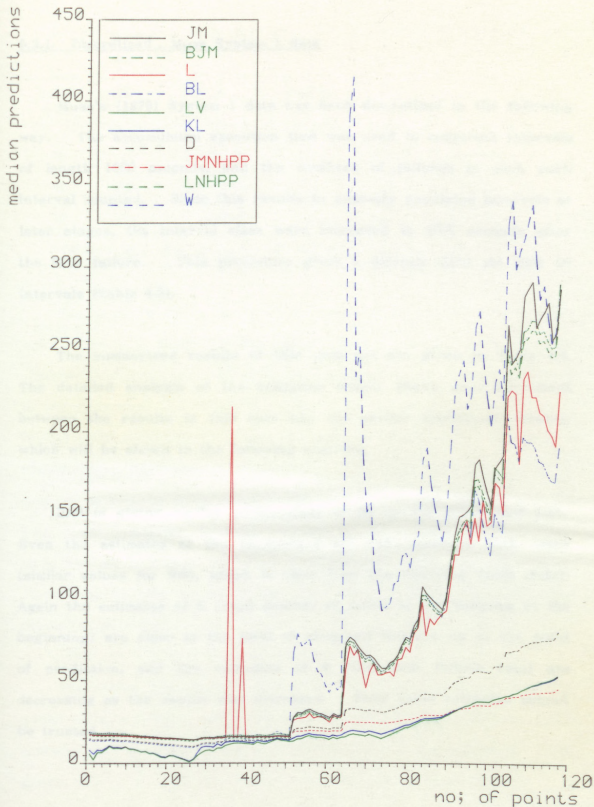
FIG.5.74. The plots of predictive medians for project B data
