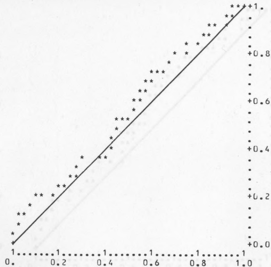
FIG. 5.10. L u-plots, data in Table 4.1, the plots based on the line printer output.
