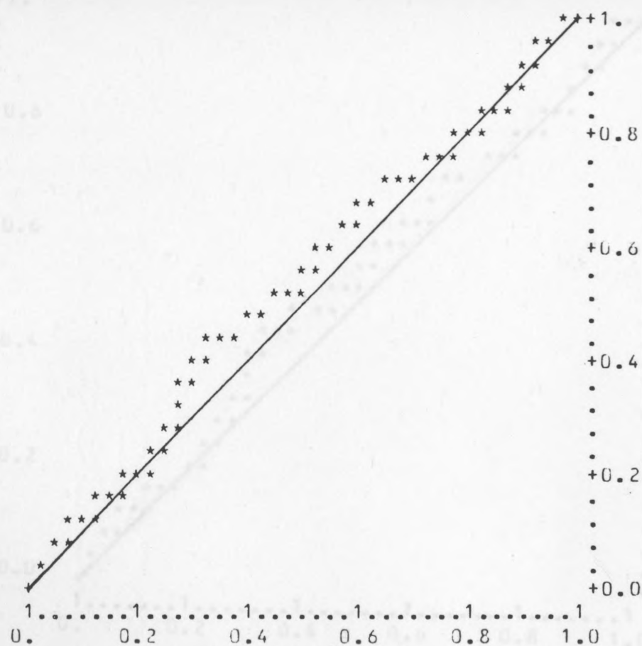
FIG.5.50. L u-plots, data in Table 5.4, the plots based on the line printer output.
