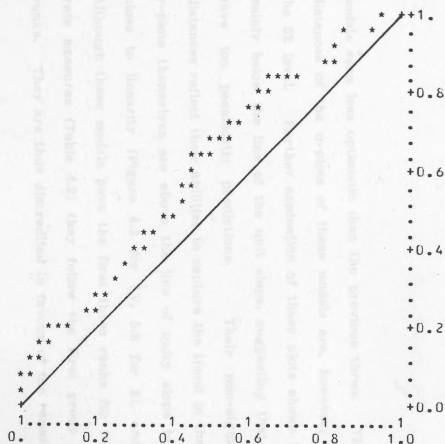
FIG. 5.4. JMNHPP u-plots, data in Table 4.1., the plots based on the line printer output.
