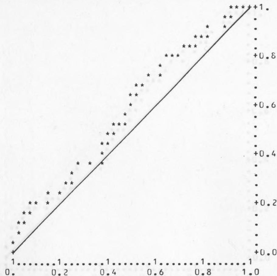
FIG.5.12. BL u-plots, data in Table 4.1., the plots based on the line printer output.
