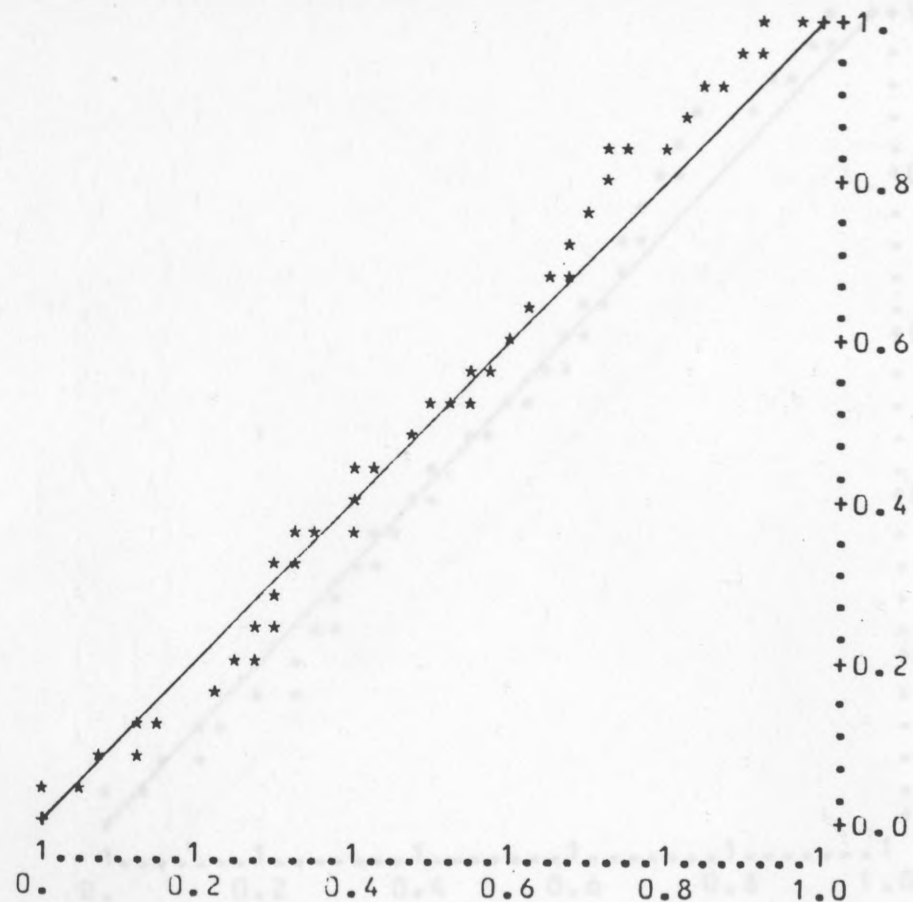
FIG. 5.31. BJM u-plots, data in Table 5.2, the plots based on the line printer output.
