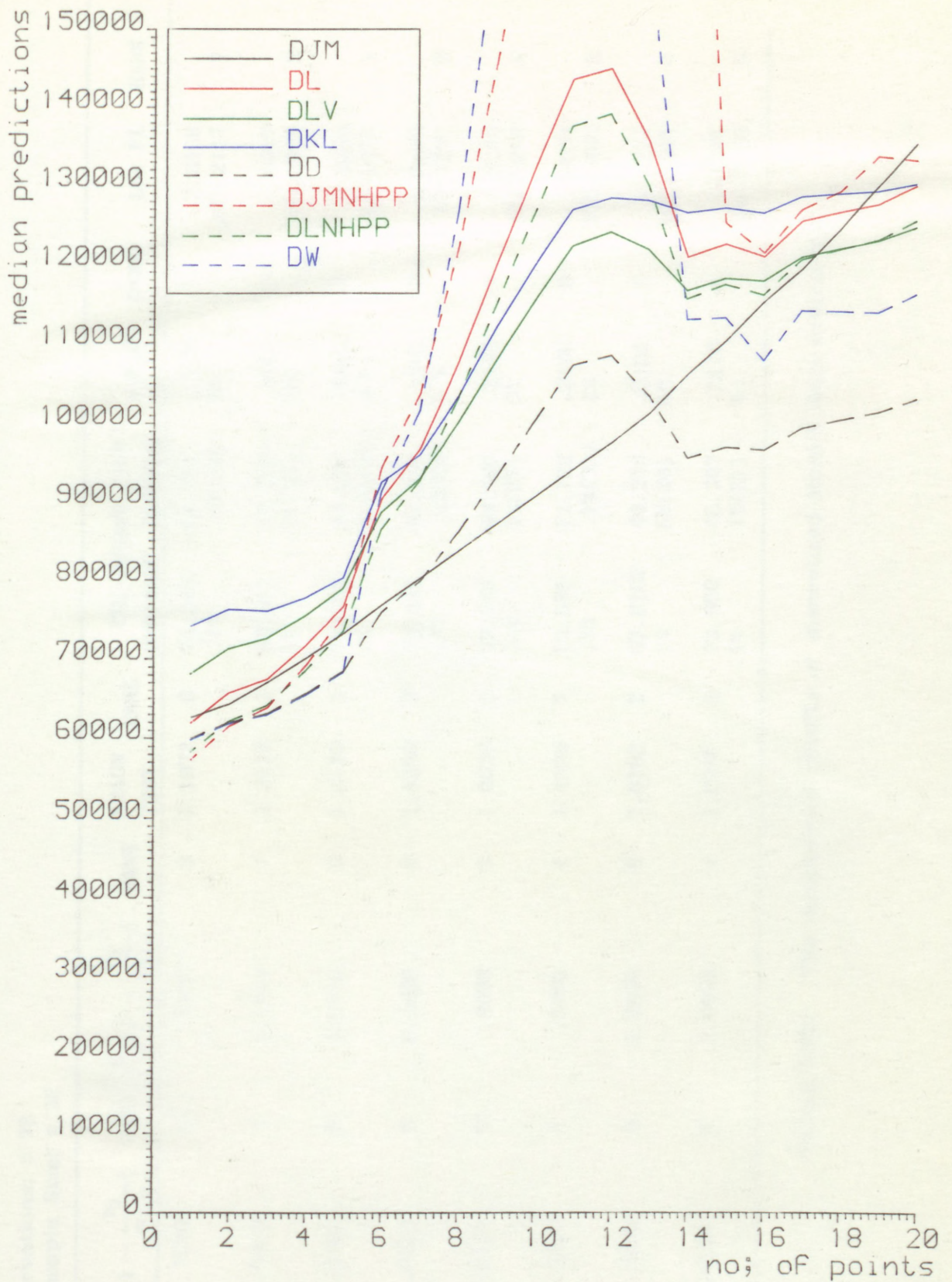
FIG.5.101. The plots of predictive median time to 1st Failure in each prediction interval For discretized Musa system SS1C data
