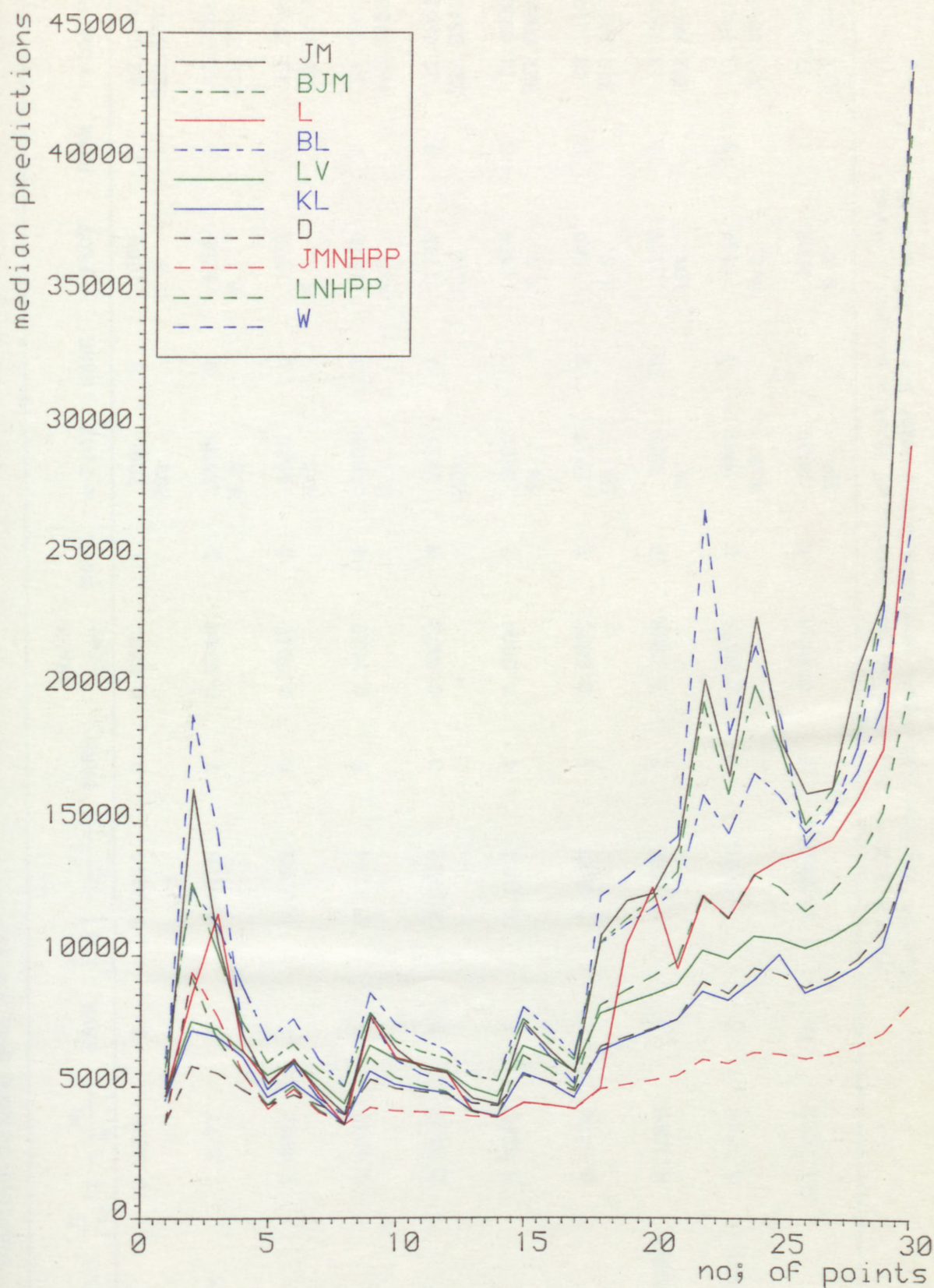
FIG.5.70. The plots of predictive medians for Moek's project 1 data
