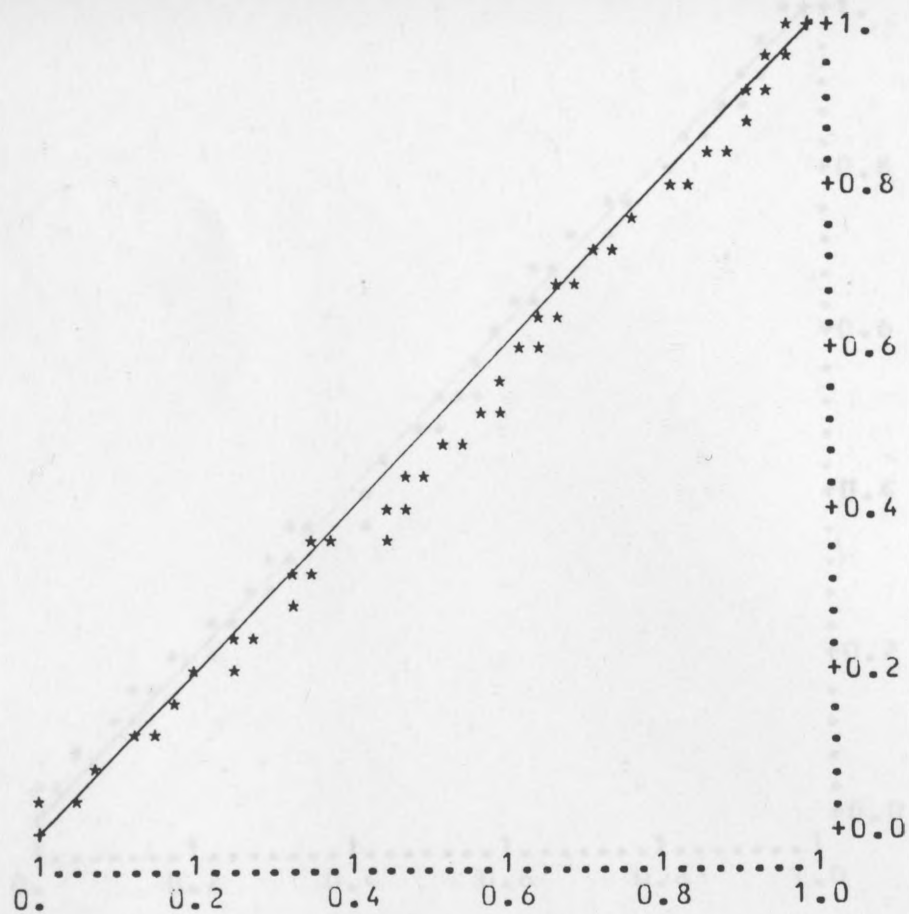
FIG. 5.30 JM y-plots, data in Table 5.2, the plots based on the line printer output.
