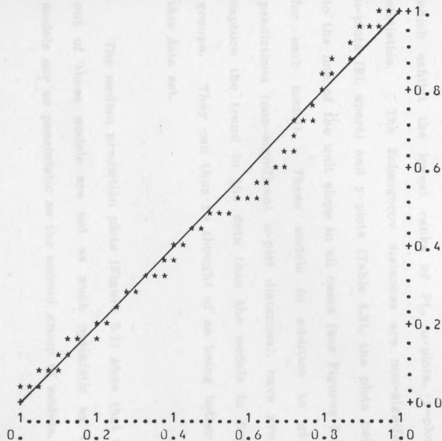
FIG. 5.5. JMNHPP y-plots, data in Table 4.1., the plots based on the line printer output.
