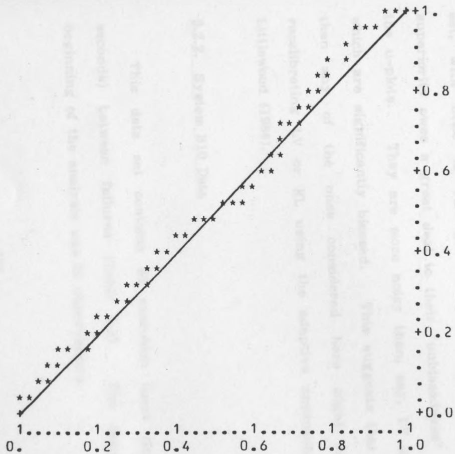
FIG.5.17. W y-plots, data in Table 4.1., the plots based on the line printer output.
