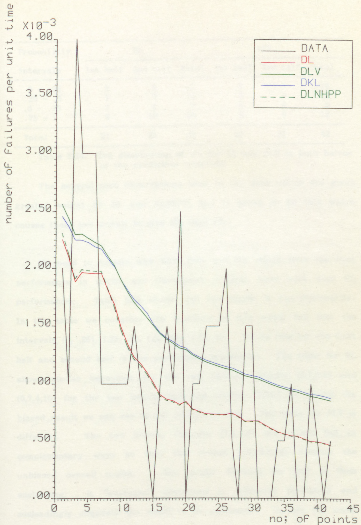
FIG.5.84. The plots of observed and predictive expected numbers of Failures per time unit for the data in Table 4.3
