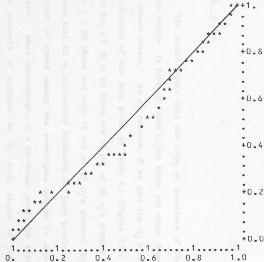
FIG.4.3. LV u-Plots, data of Table 4.1, the plots based on the line printer output.
