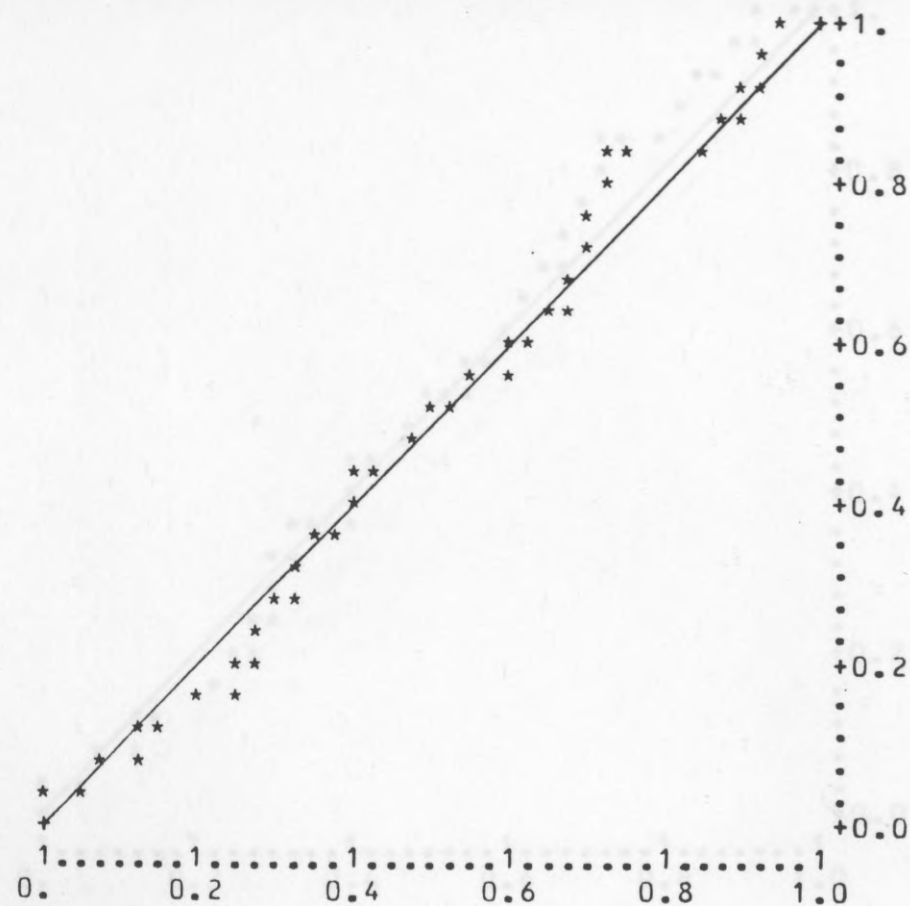
FIG. 5.29. JM u-plots, data in Table 5.2, the plots based on the line printer output.
