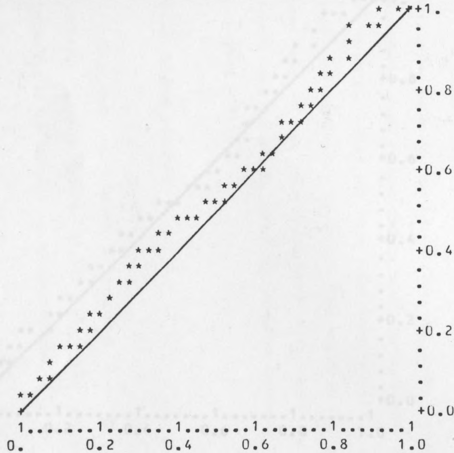
FIG.5.15. LNHPP y-plots, data in Table 4.1, the plots based on the line printer output.
