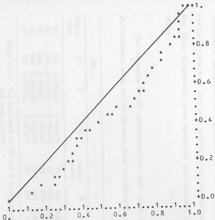
FIG.5.79. DLNHPP u-plots. data in Table 4.3., the plots based on the line printer output.
