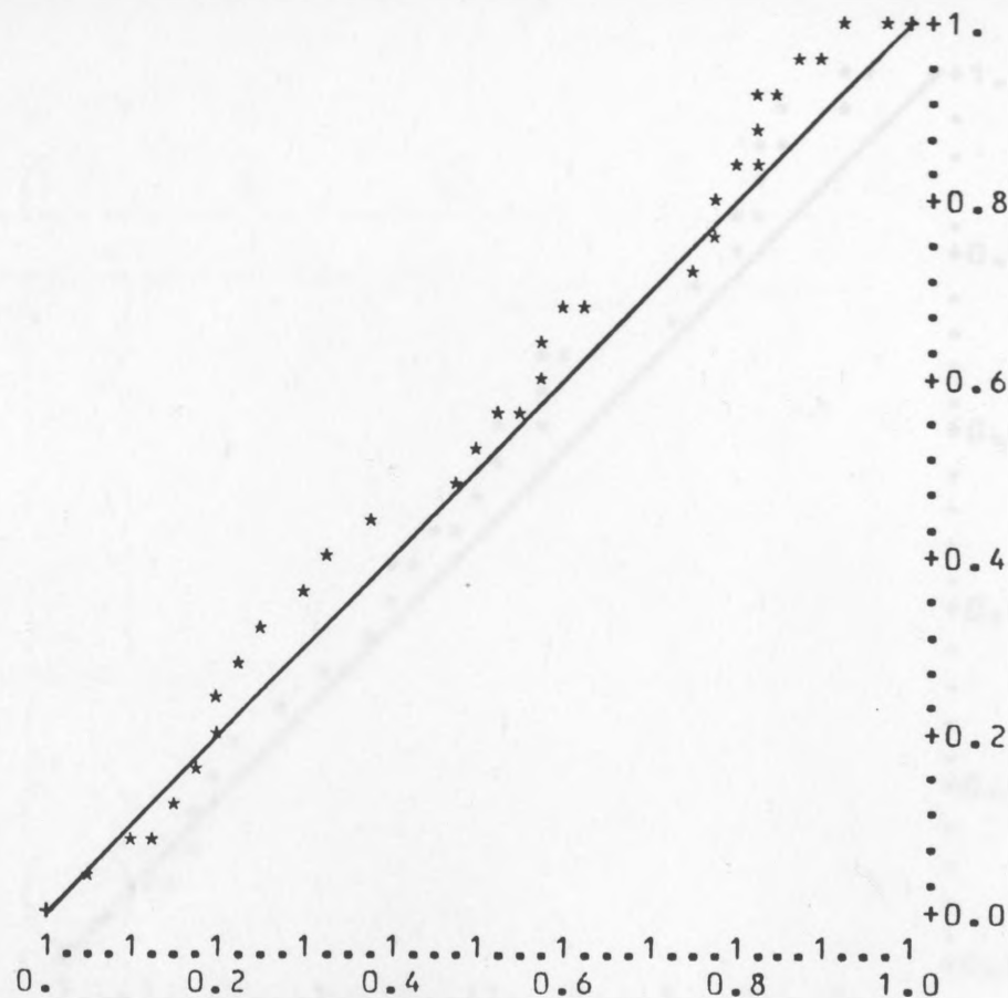
FIG. 5.80. DD u-plots, data in Table 4.3, the plots based on the line printer output.
