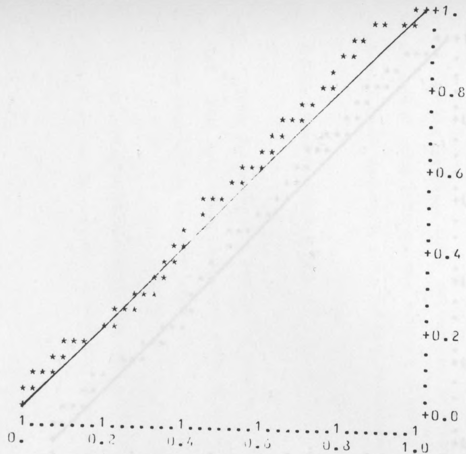
FIG.5.57. LNHPP y-plots, data in Table 5.4, the plots based on the line printer output.
