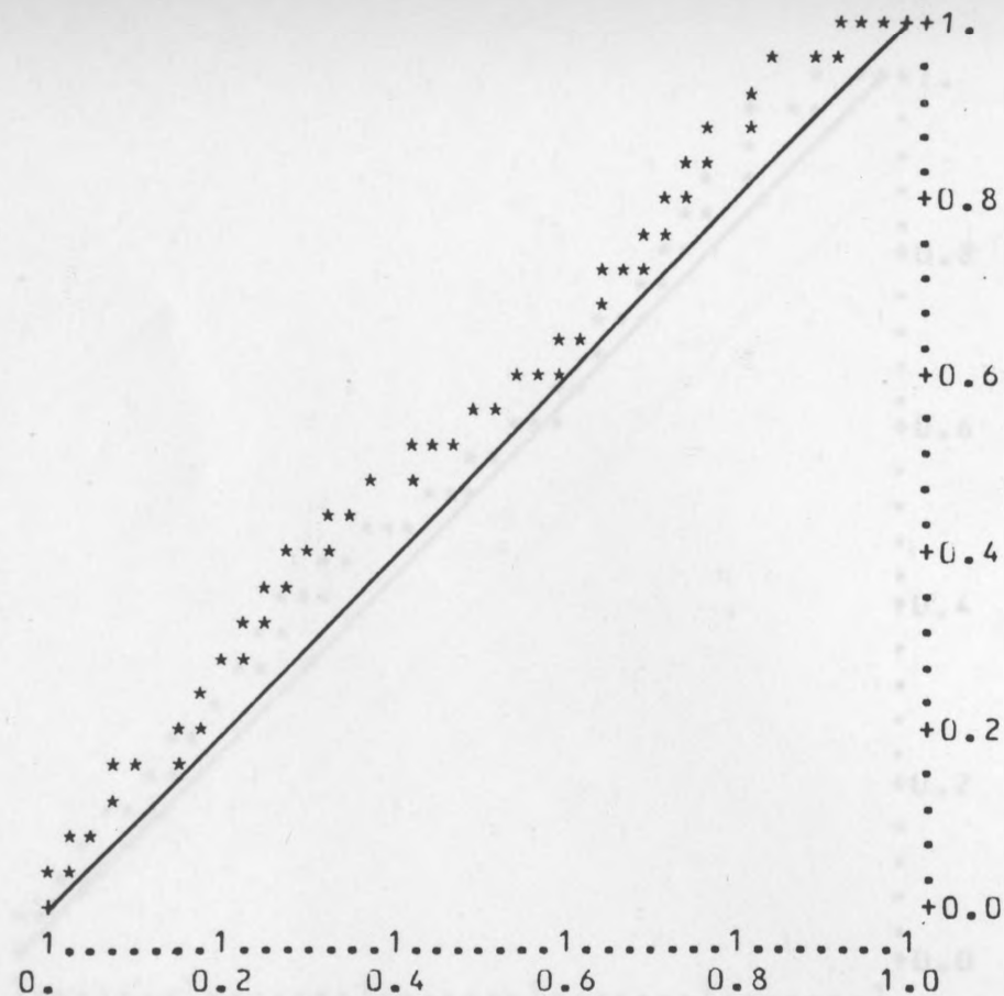
FIG.5.9 D y-plots, data in Table 4.1, the plots. based on the line printer output.
