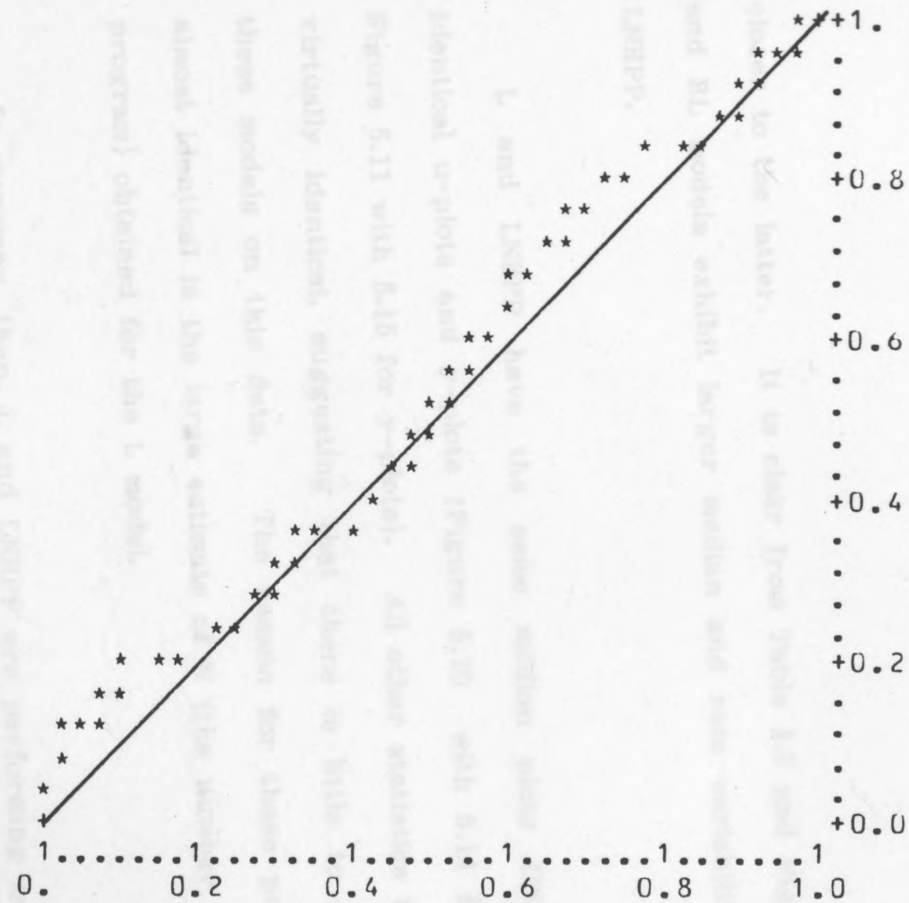
FIG.5.16. W u-plots, data in Table 4.1., the plots based on the line printer output.
