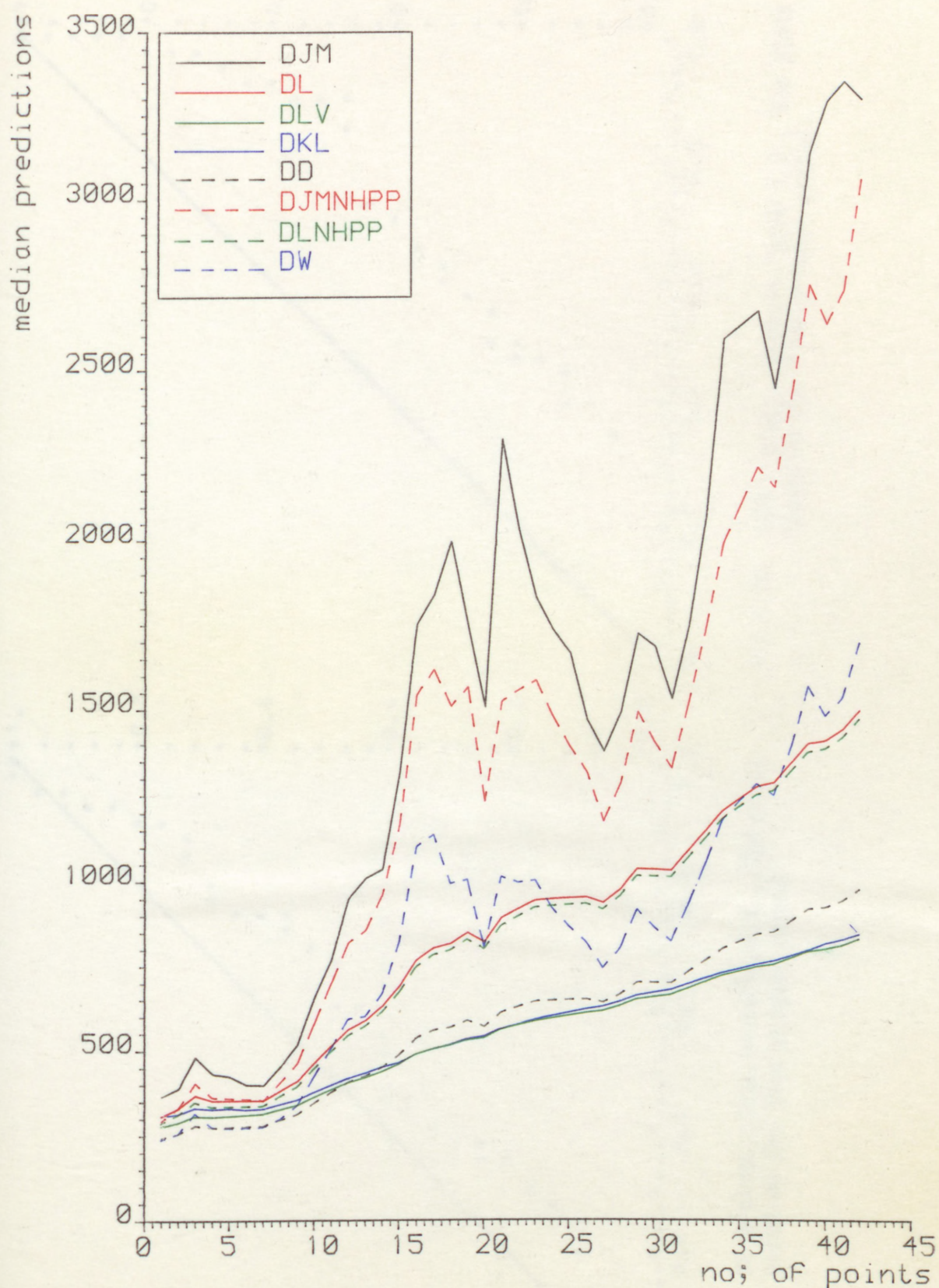
FIG.5.75. The plots of predictive median time to 1st Failure in each prediction interval for the data in Table 4.3
