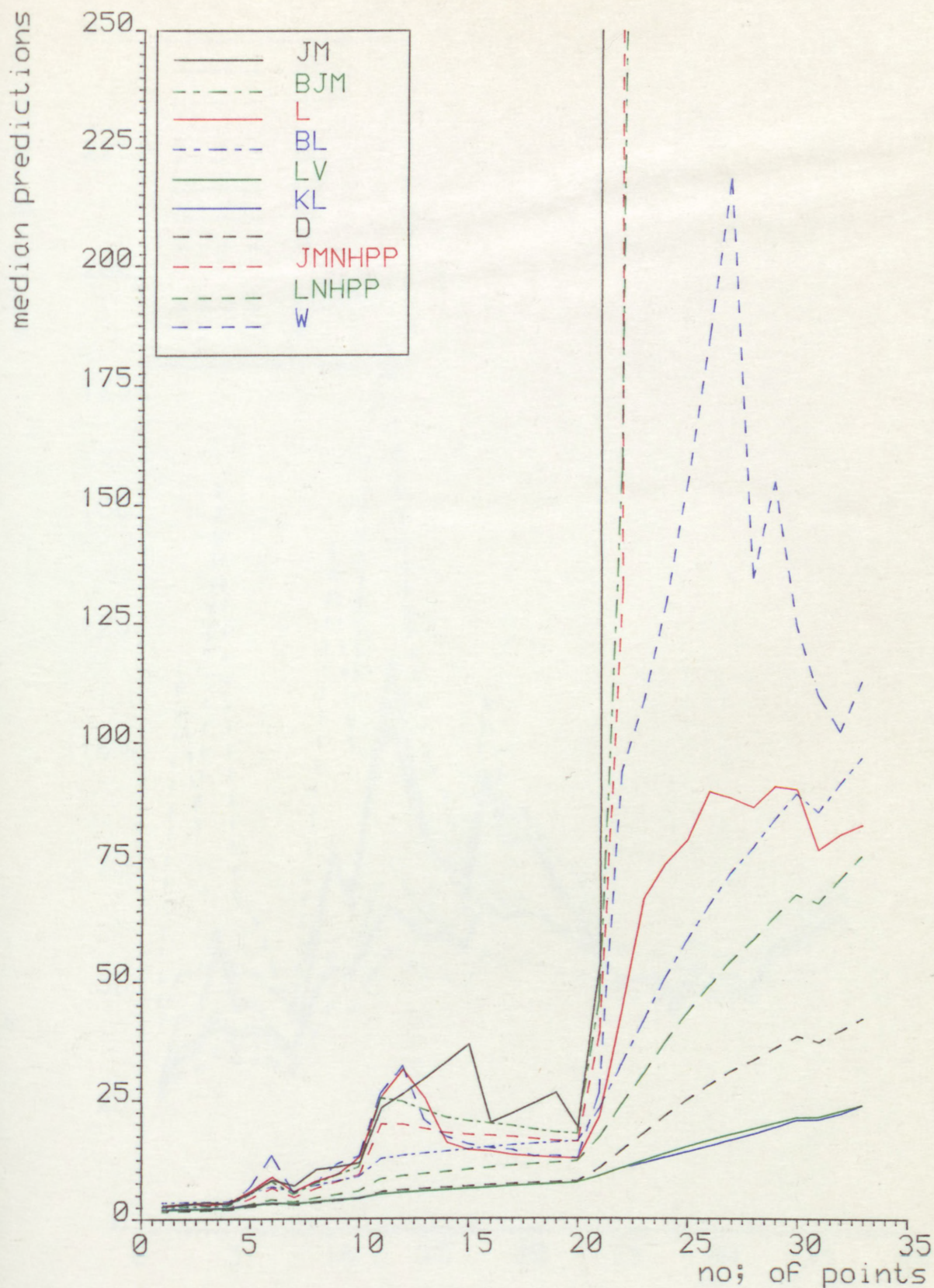
FIG.5.71. The plots of predictive medians for Moek's project 2 data
