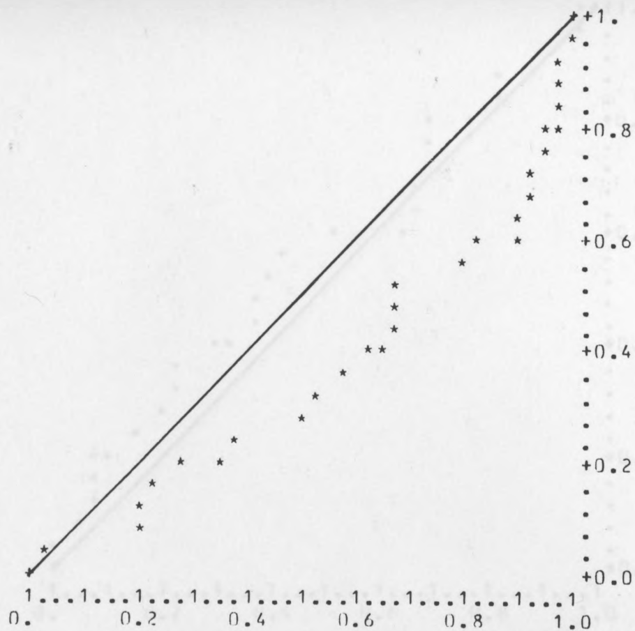
FIG.5.89. DLNHPP u-plots, data in Table 5.25, the plots based on the line printer output.
