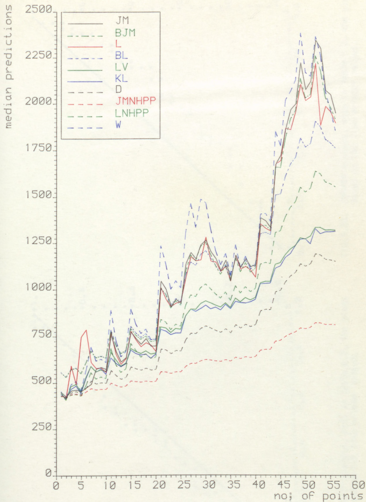
FIG.5.22. The plots of predictive medians for the data in Table 5.2
