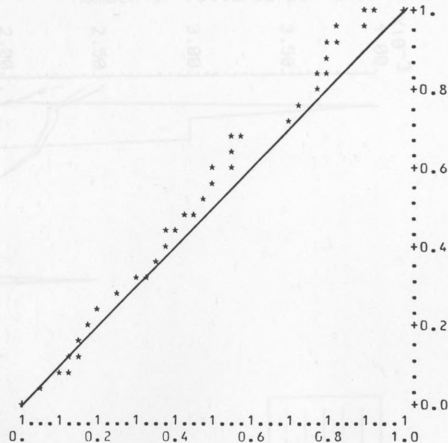
FIG.5.82. DLV u-plots, data in Table 4.3, the plots based on the line printer output.
