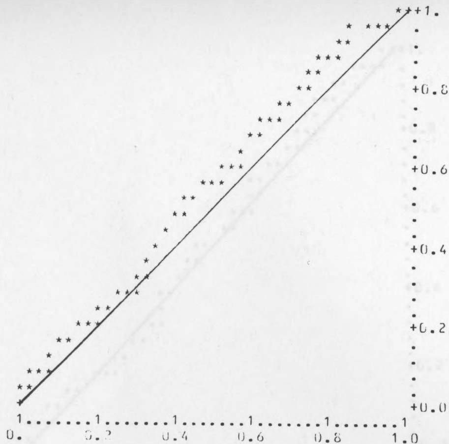
FIG. 5.45. D y-plots, data in Table 5.4, the plots based on the line printer output.
