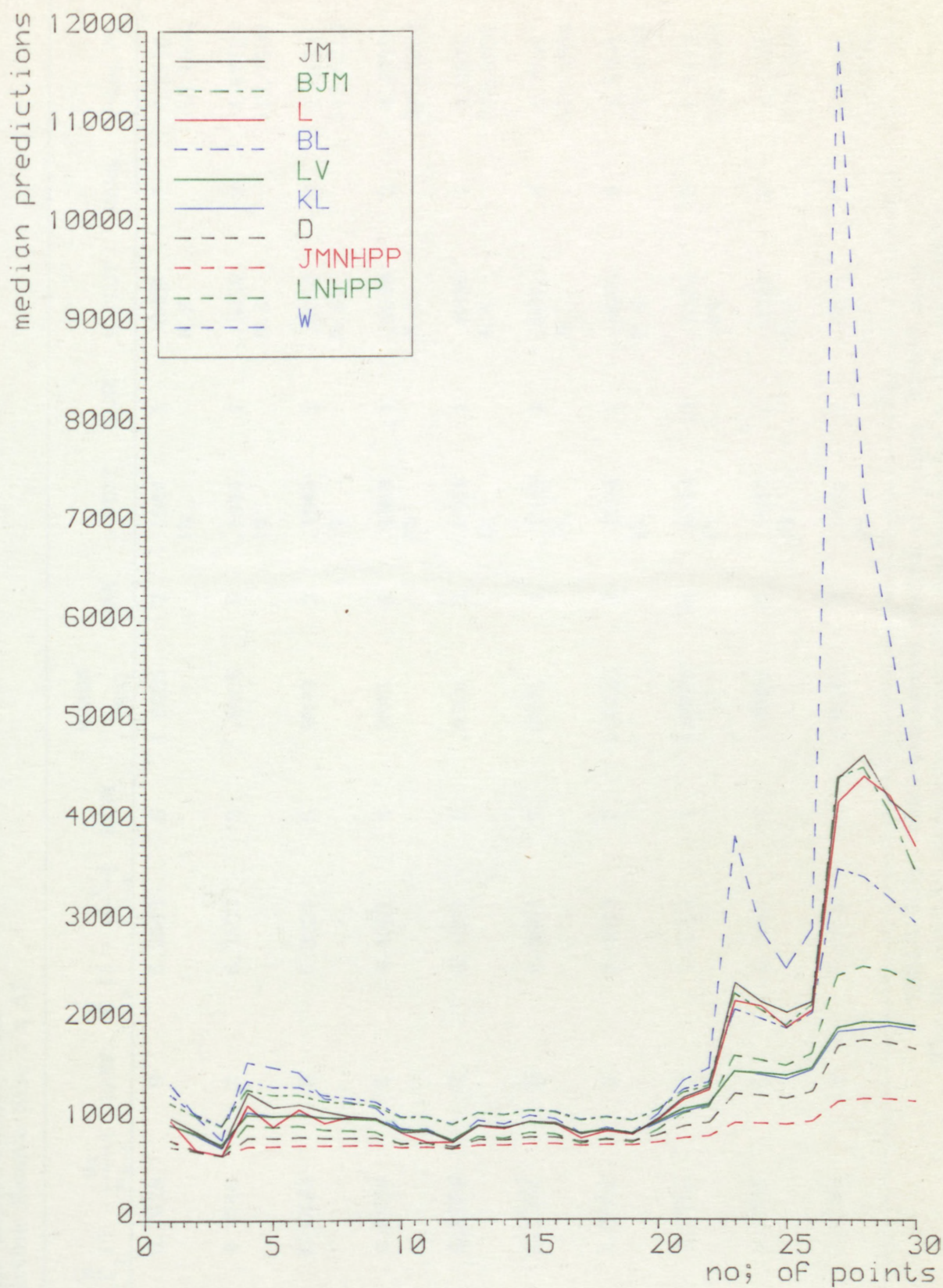
FIG.5.68. The plots of predictive medians For data-B7 HH60D 2FNS
