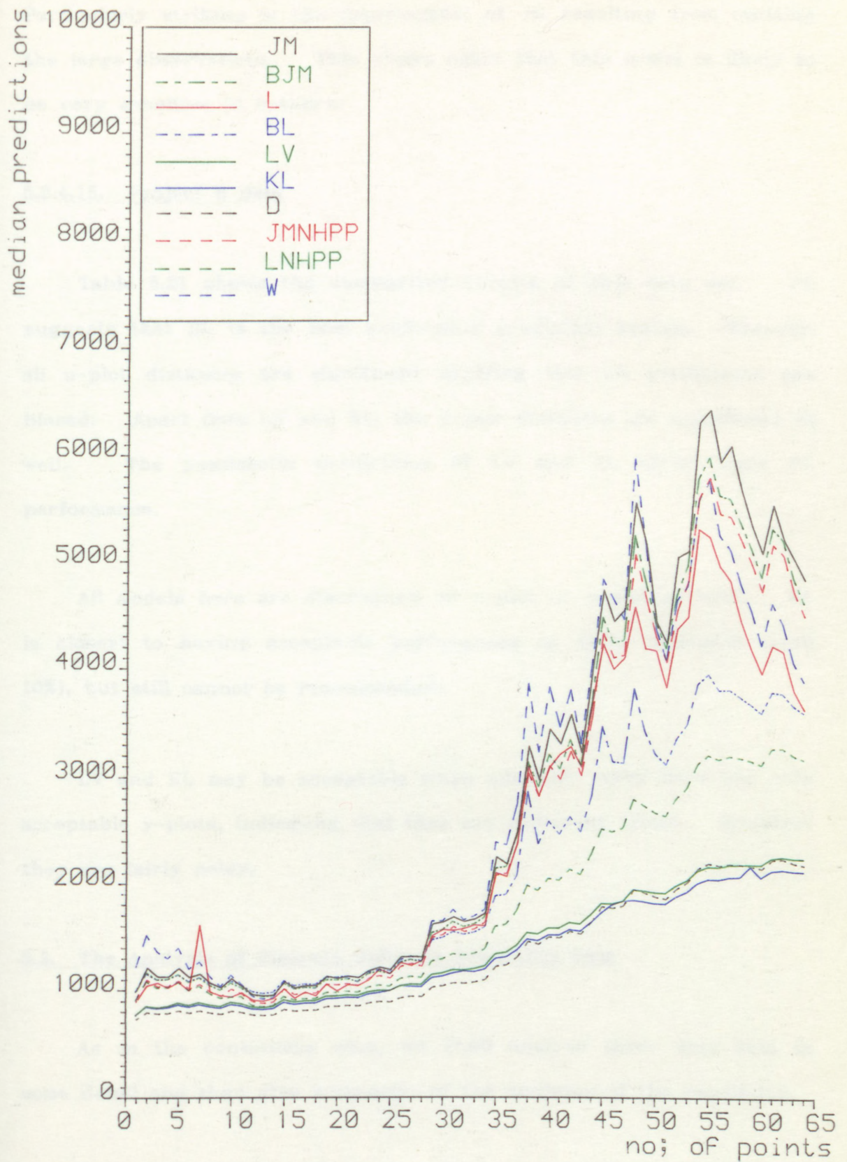
FIG.5.73b. The plots of predictive medians for system MDSIM data without the large obs; which equal to 33340.
