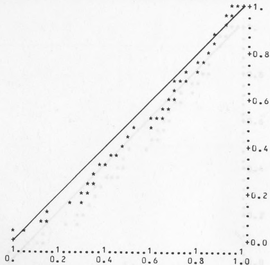
FIG.5.18. LV u-plots, data in Table 5.2, the plots based on the line printer output.
