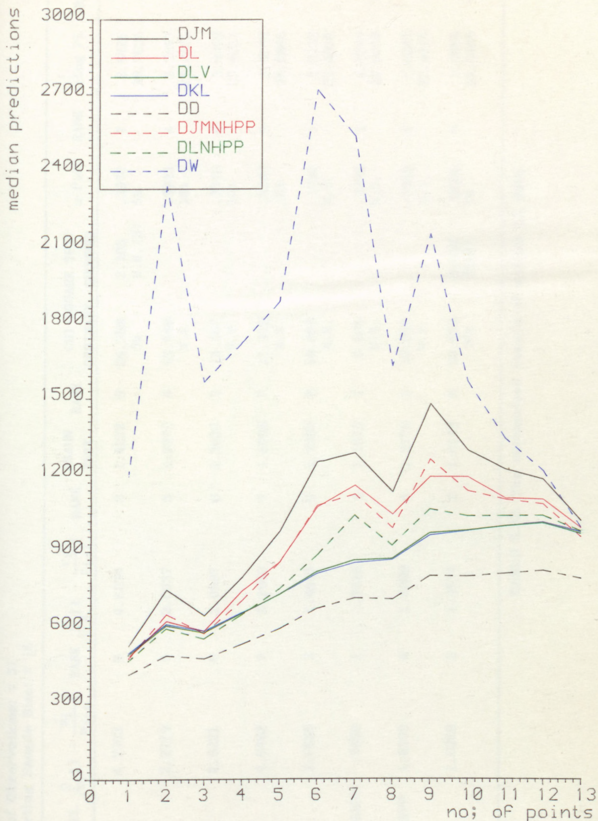
FIG.5.95. The plots of predictive median time to 1st failure in each prediction interval for system L1 data(AD-L1)
