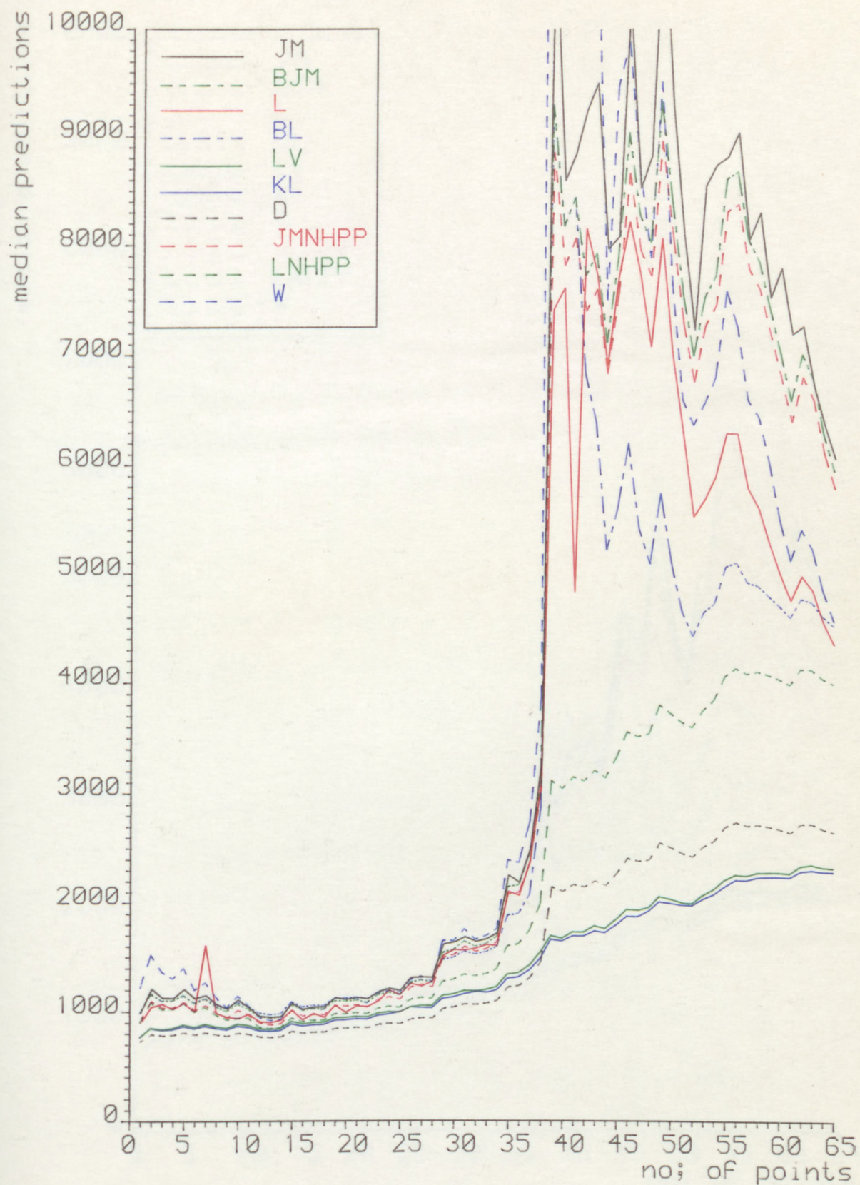
FIG.5.73a. The plots of predictive medians for system MDSIM data
