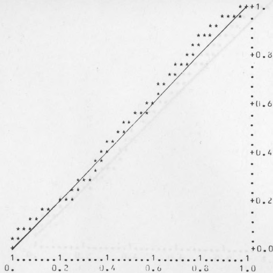
FIG.5.51. L y-plots, data in Table 5.4, the plots based on the line printer output.
