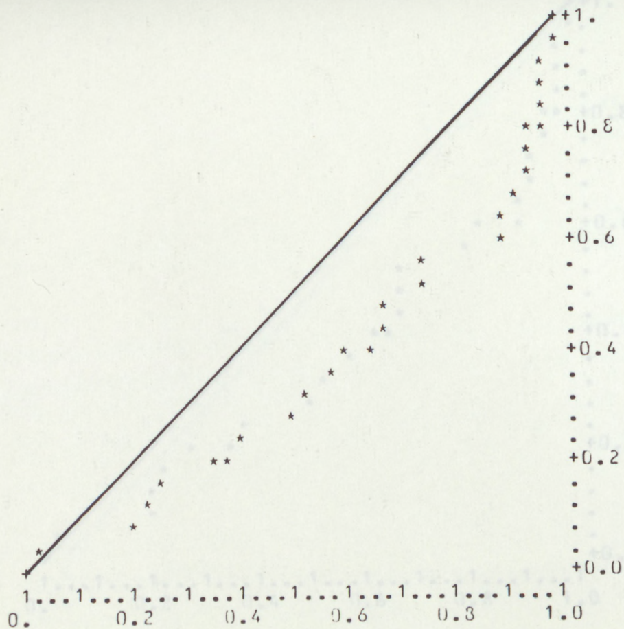
FIG.5.87. DL u-plots, data in Table 5.25, the plots based on the line printer output.
