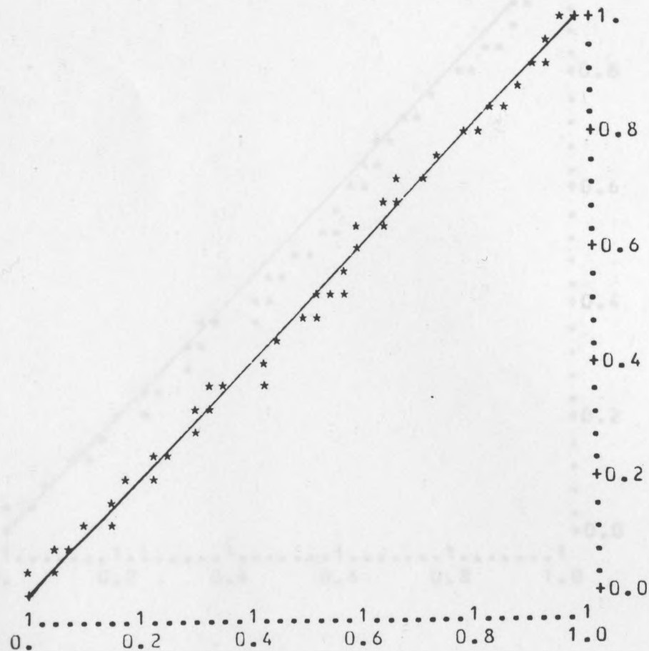
FIG.5.28. LNHPP y-plots, data in Table 5.2, the plots based on the line printer output.
