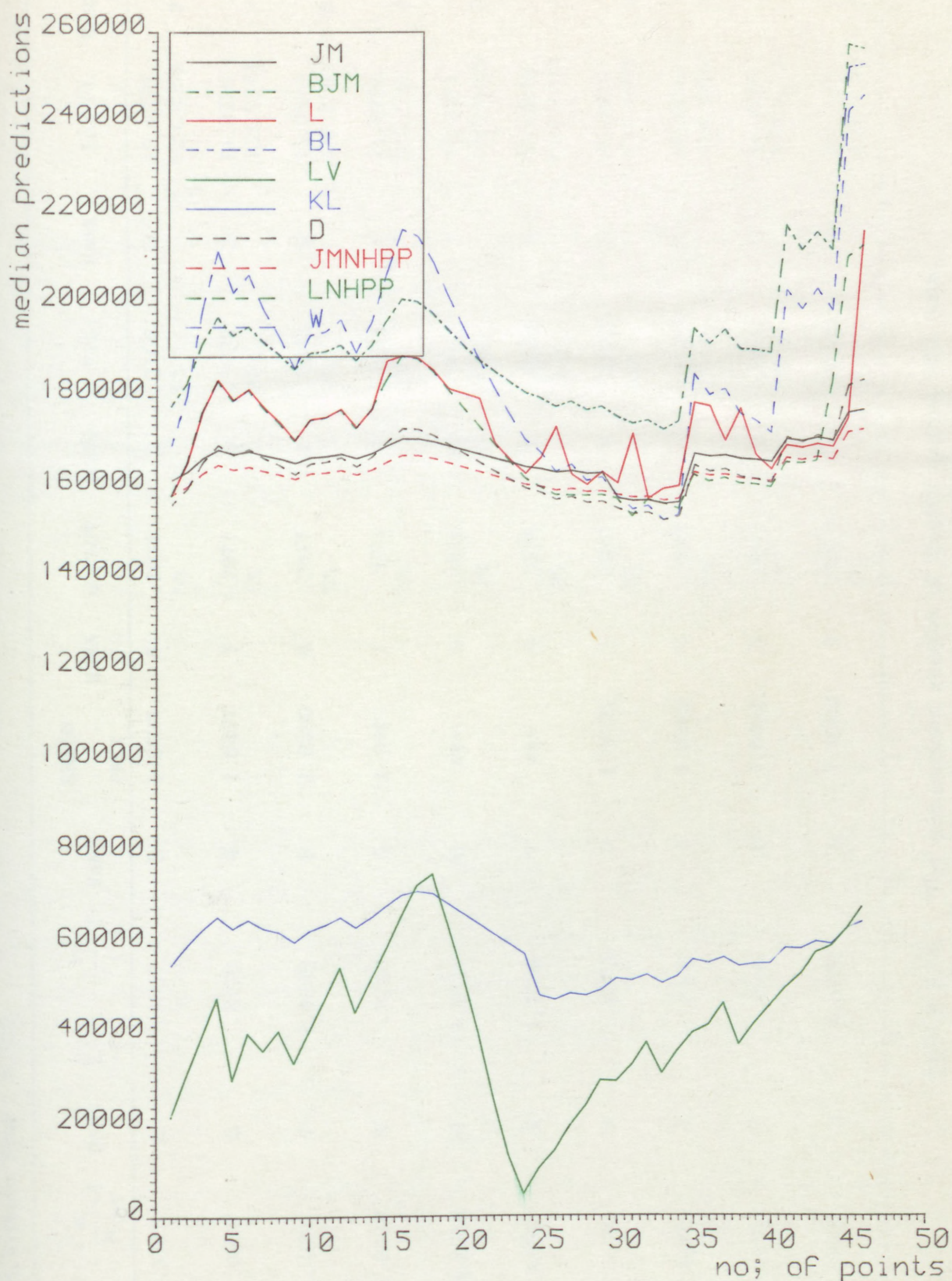
FIG.5.67. The plots of predictive medians for Musa's system ss4 data
