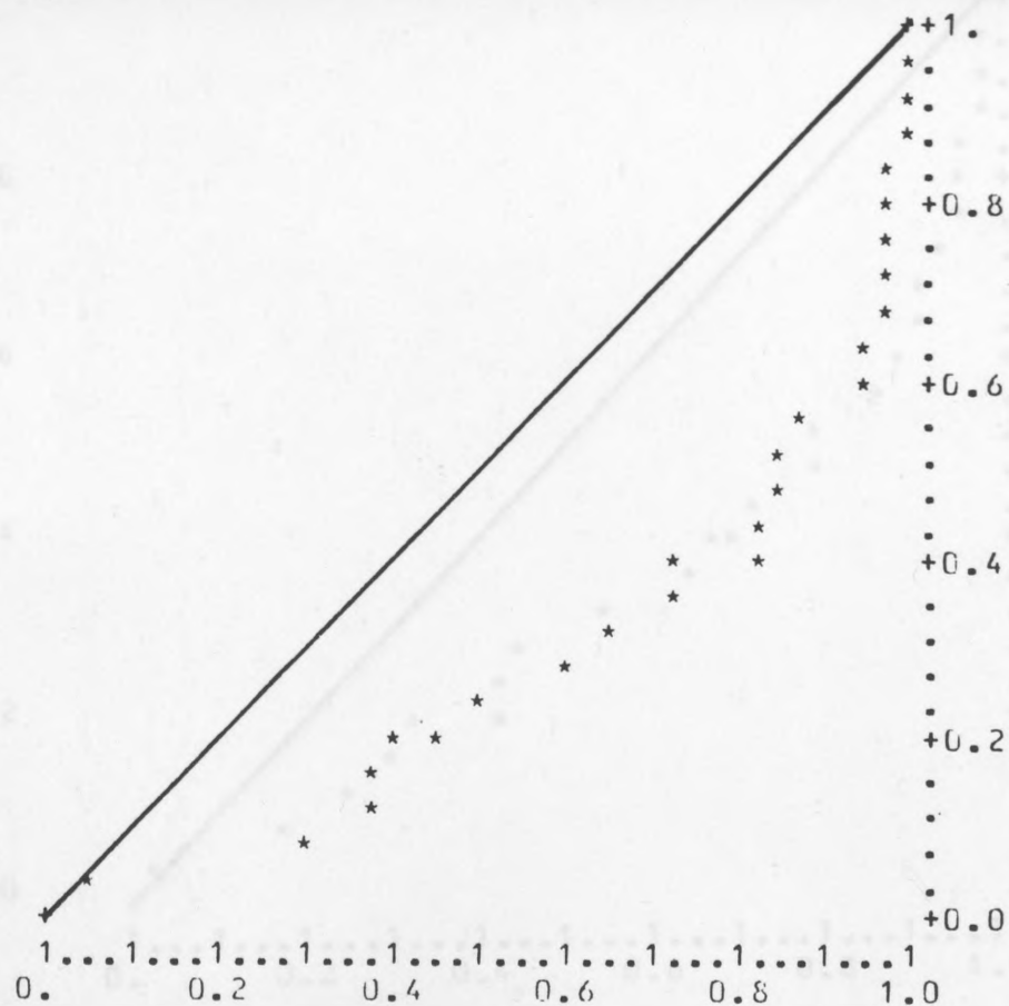
FIG. 5.88. DJMNHPP u-plots, data in Table 5.25, the plots based on the line printer output.
