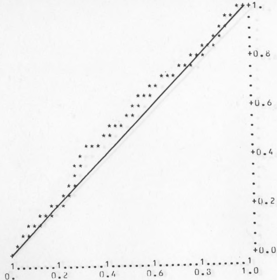
FIG. 5.46. JM u-plots, data in Table 5.4, the plots based on the line printer output.
