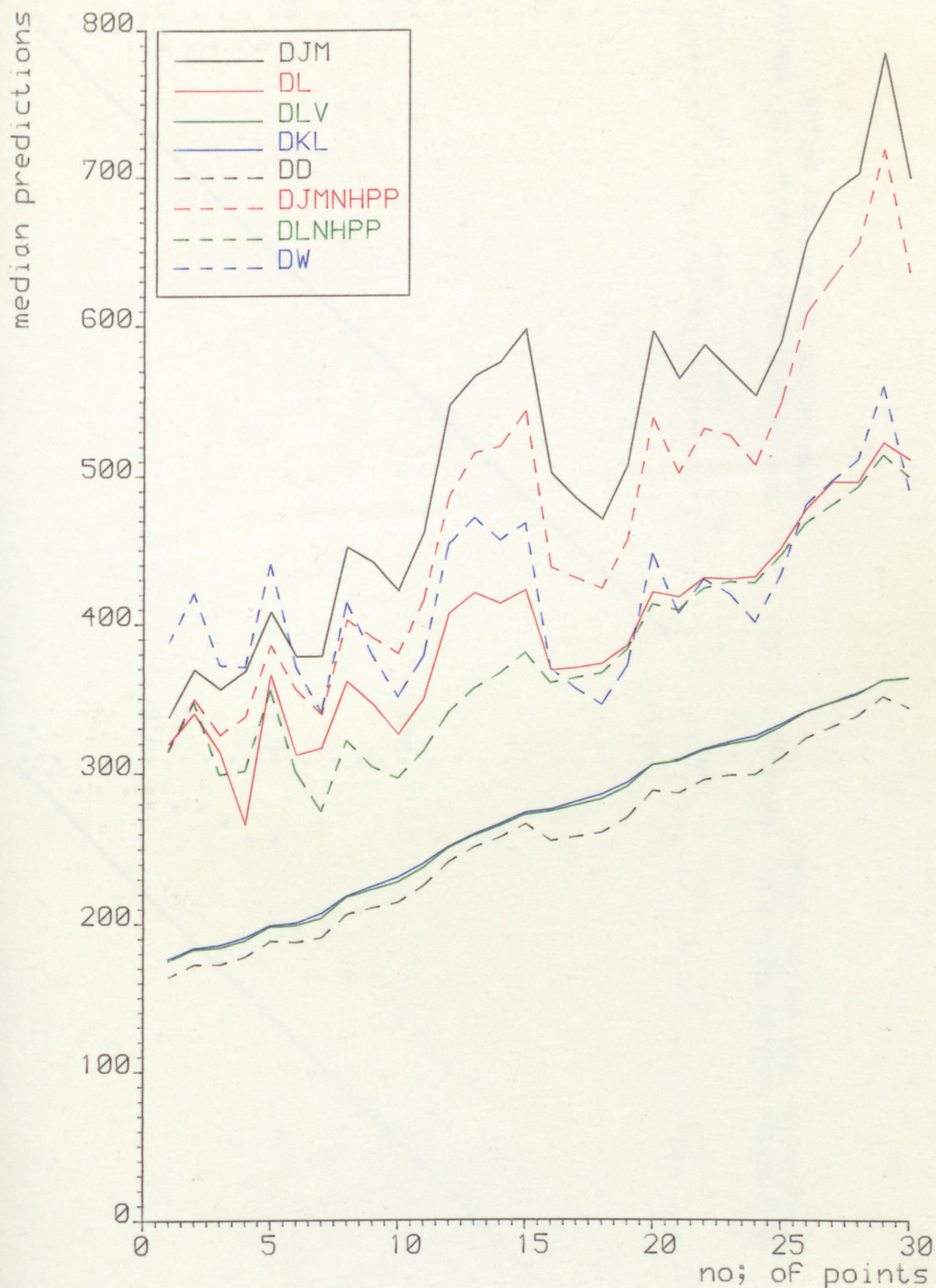
FIG.5.85. The plots of predictive median time to 1st Failure in each prediction interval For the data in Table 4.25
