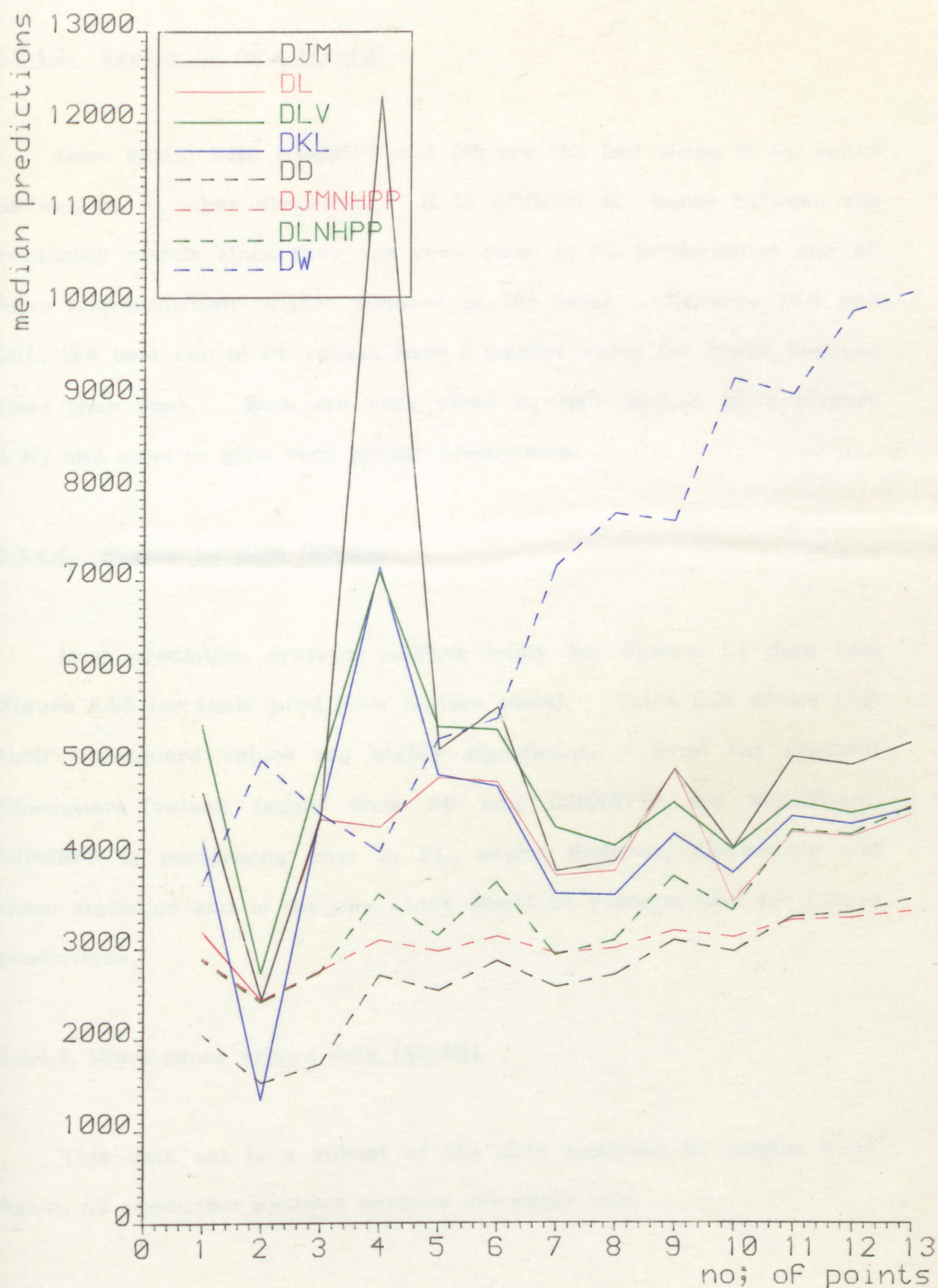
FIG.5.96. The plots of predictive median time to 1st failure in each prediction interval for system L2 data(AD-L2)
