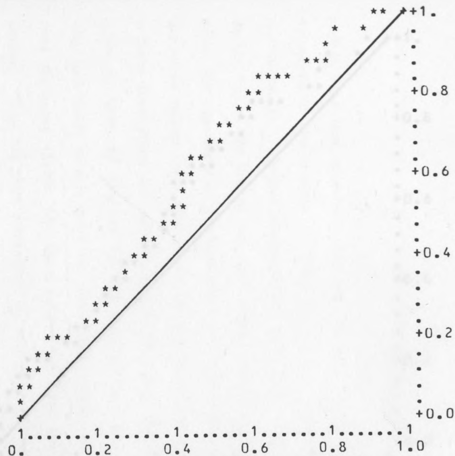
FIG. 5.2. BJM u-plots, data in Table 4.1, the plots based on the line printer output.
