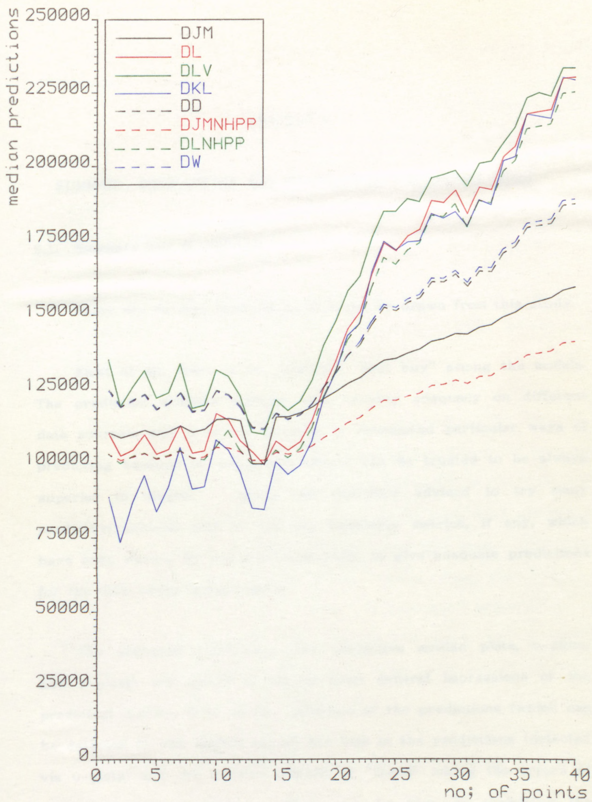
FIG.5.102. The plots of predictive median time to 1st Failure in each prediction interval for discretized Musa system SS3 data
