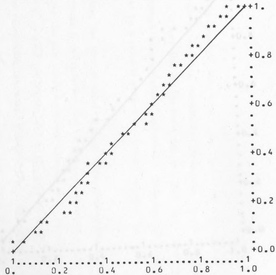
FIG.5.35. BL u-plots, data in Table 5.2, the plots based on the line printer output.
