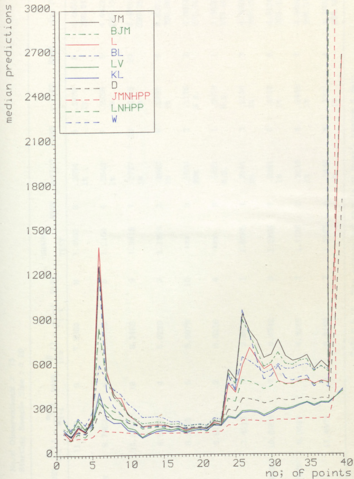
FIG.5.65. The plots of predictive medians for Musa's system 4 data
