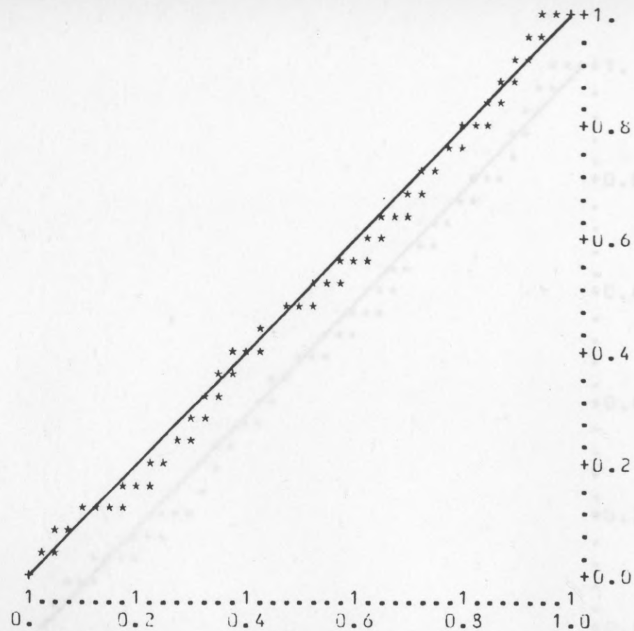
FIG. 5.40. LV u-plots, data in Table 5.4, the plots based on the line printer output.
