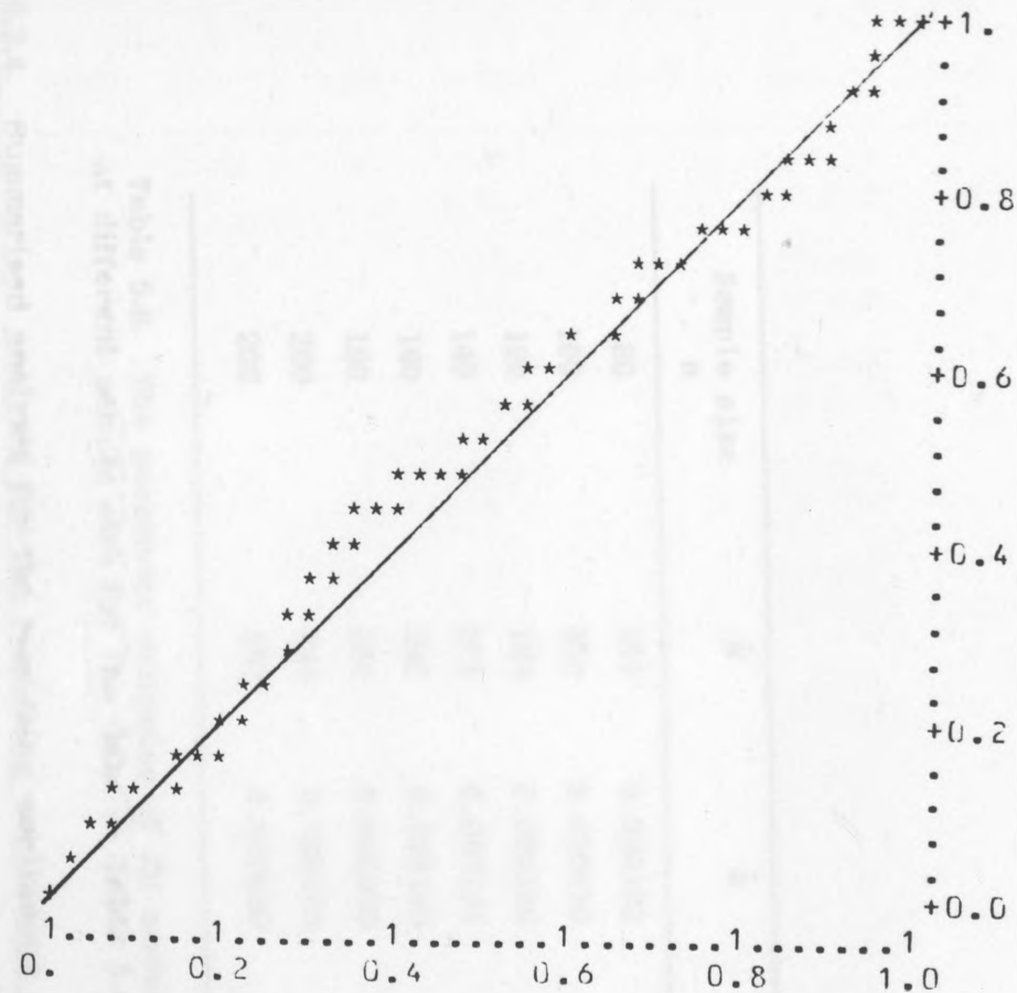
FIG. 5.58. W u-plots, data in Table 5.4, the plots based on the line printer output.
