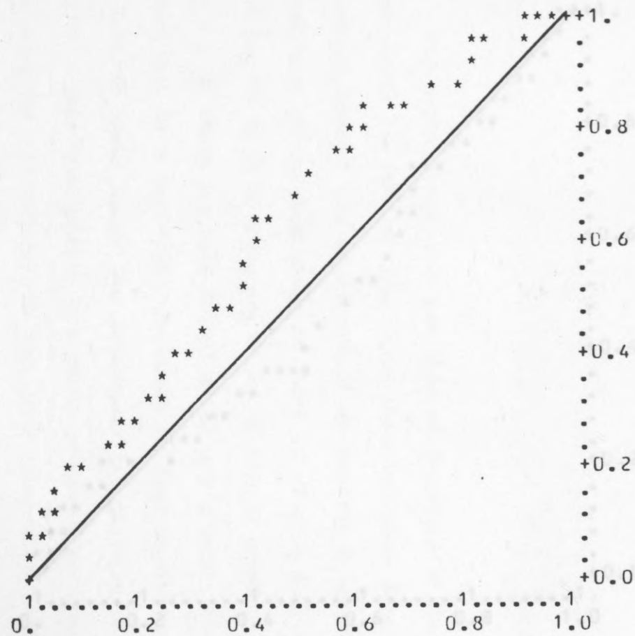
FIG.4.1. JM u-Plots, data of Table 4.1, the plots based on the line printer output.
