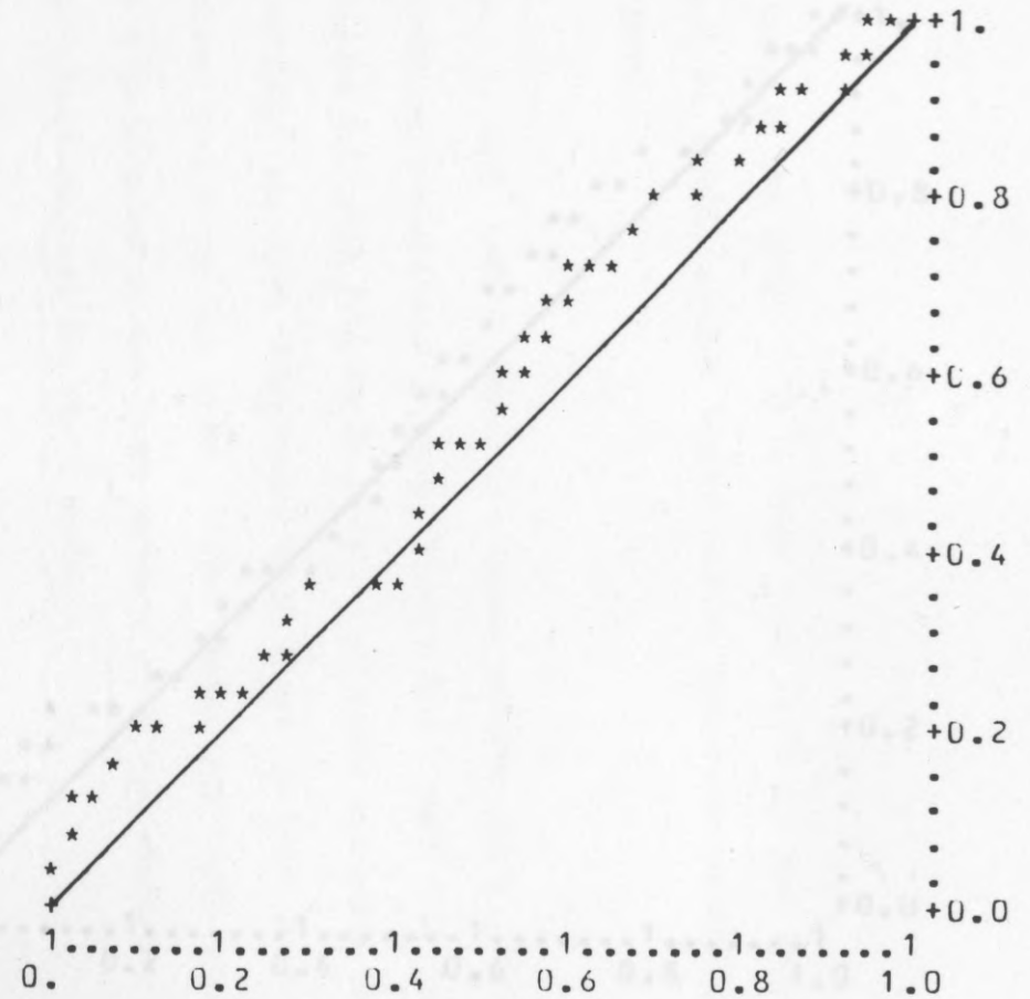
FIG.5.14. LNHPP u-plots, data in Table 4.1, the plots based on the line printer output.
