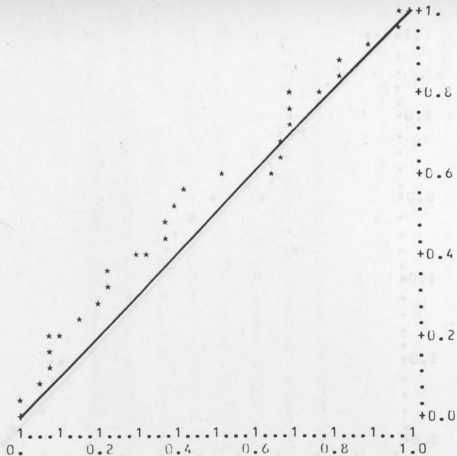
FIG.5.91. DD u-plots, data in Table 5.25, the plots based on the line printer output.
