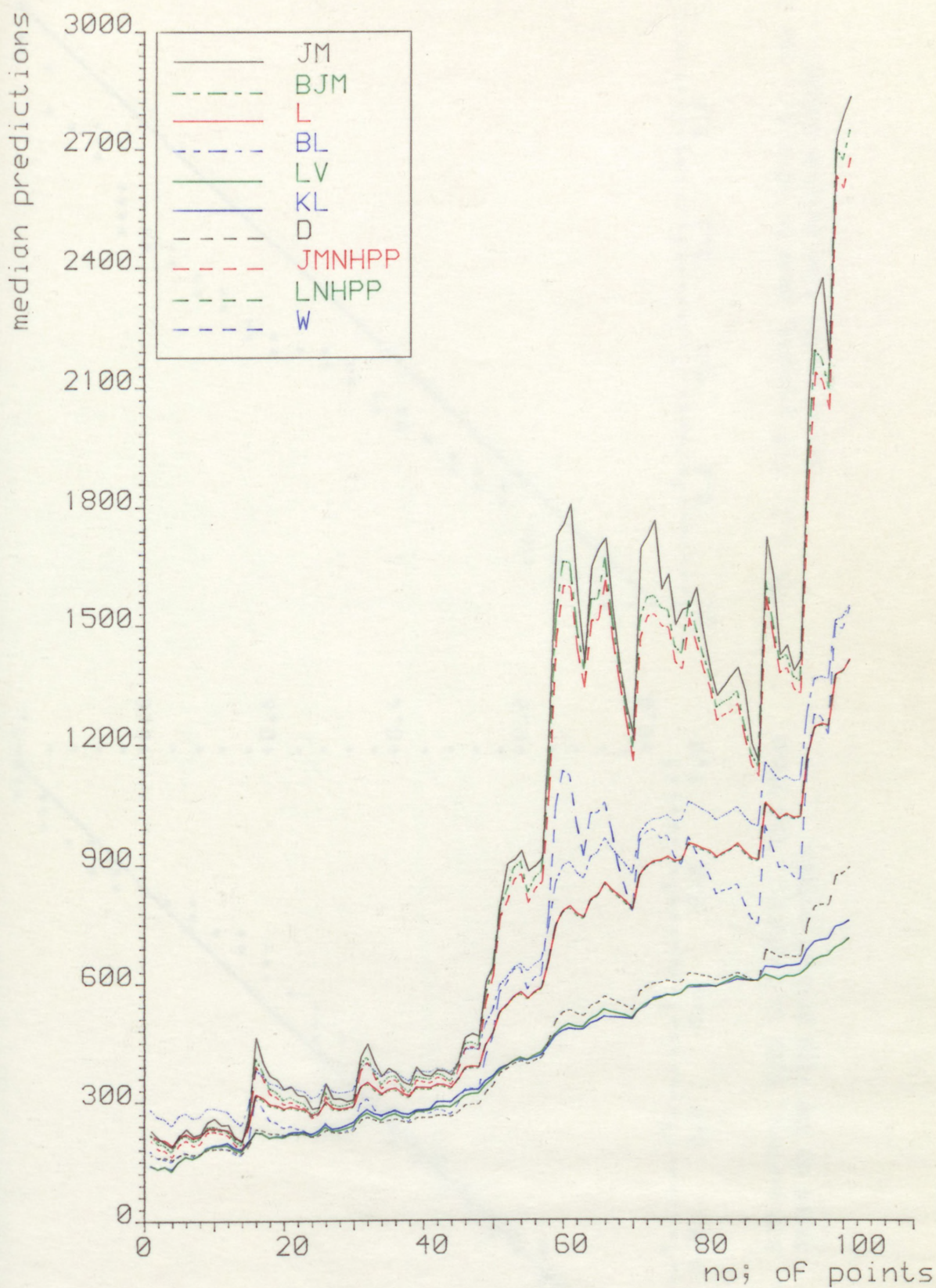
FIG.5.1. The plots of predictive medians for the data in Table 4.1
