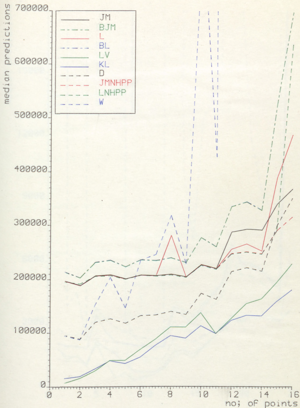
FIG.5.60. The plots of predictive medians for Musa's system 14c data
