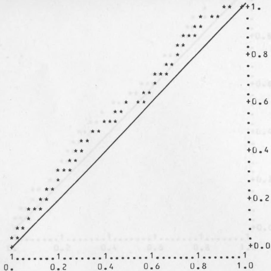
FIG. 5.7. KL y-plots, data in Table 4.1, the plots based on line printer output.
