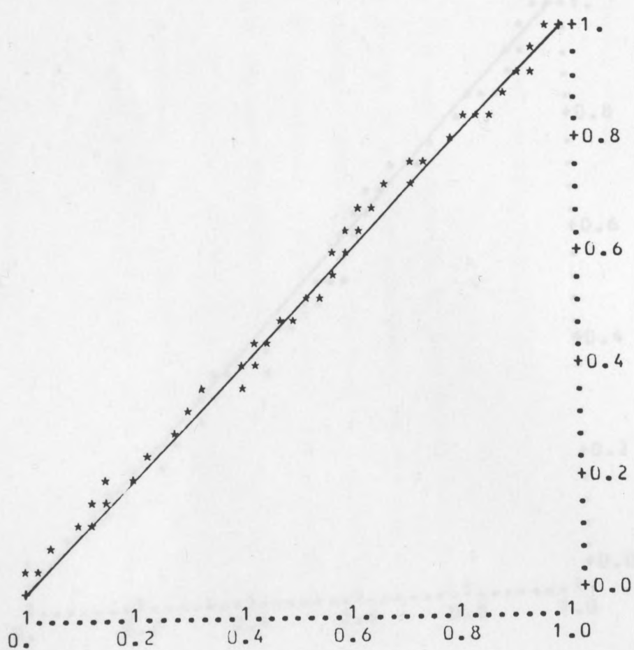
FIG.5.36. BL y-plots, data in Table 5.2, the plots based on the line printer output.
