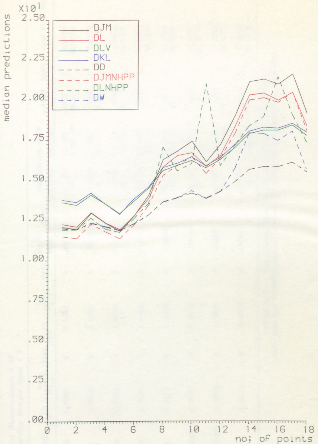
FIG.5.99. The plots of predictive median time to 1st failure in each prediction interval For Misra minor errors data(AD-MI)
