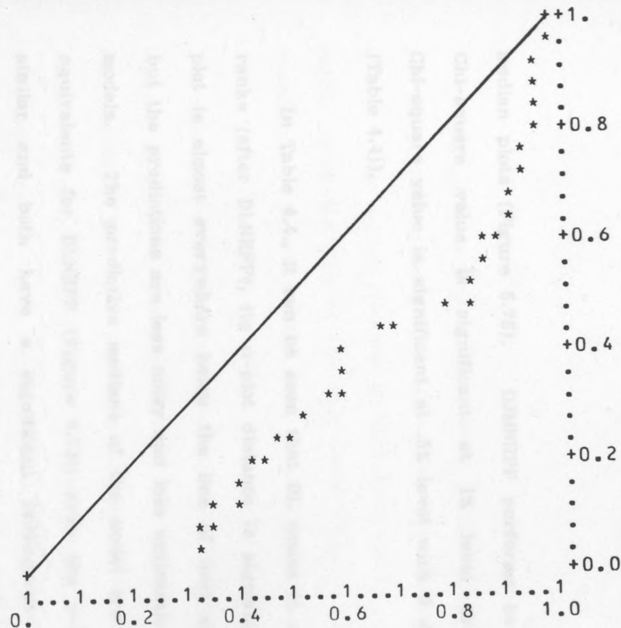
FIG.5.78. DJMNHPP u-plots, data in Table 4.3, the plots based on the line printer output.
