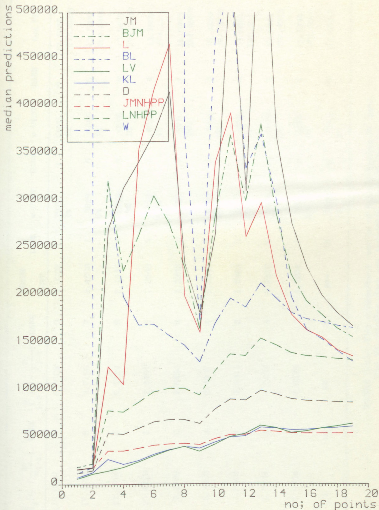
FIG.5.63. The plots of predictive medians for Musa's system 27 data
