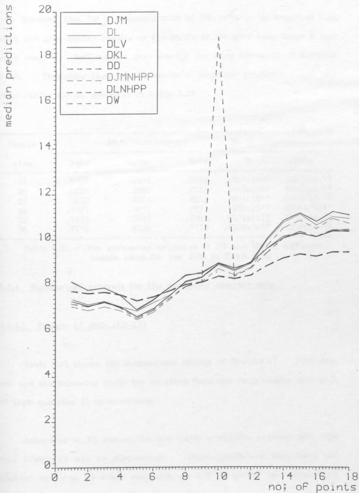
FIG.5.94. The plots of predictive median time to 1st Failure in each prediction interval For the data in Table 4.28
