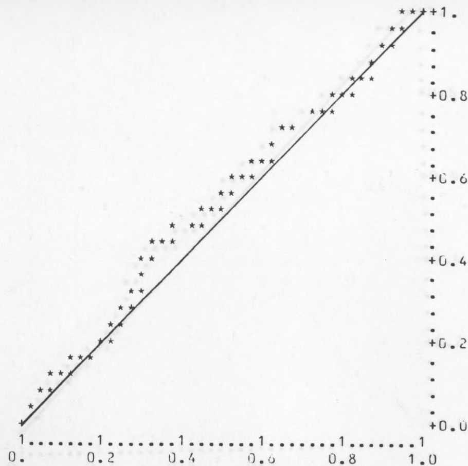
FIG. 5.52. BL u-plots, data in Table 5.4, the plots based on the line printer output.
