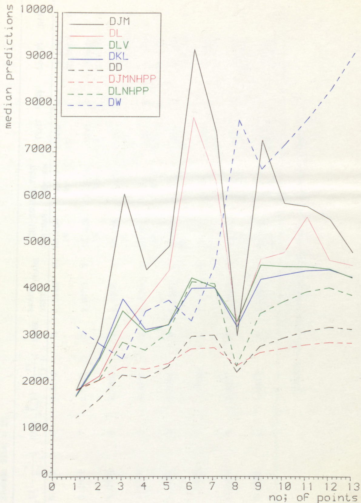
FIG.5.98. The plots of predictive median time to 1st failure in each prediction interval for system L4 data(AD-L4)
