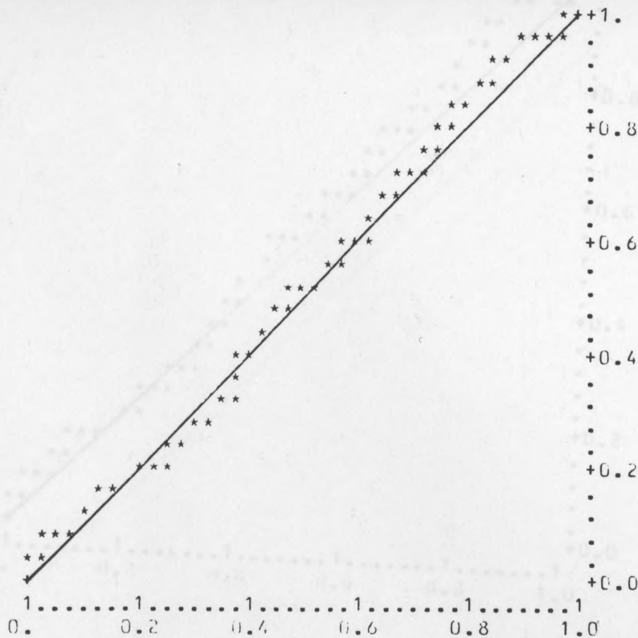
FIG. 5.55 JMNHPP y-plots, data in Table 5.4, the plots based on the line printer output.
