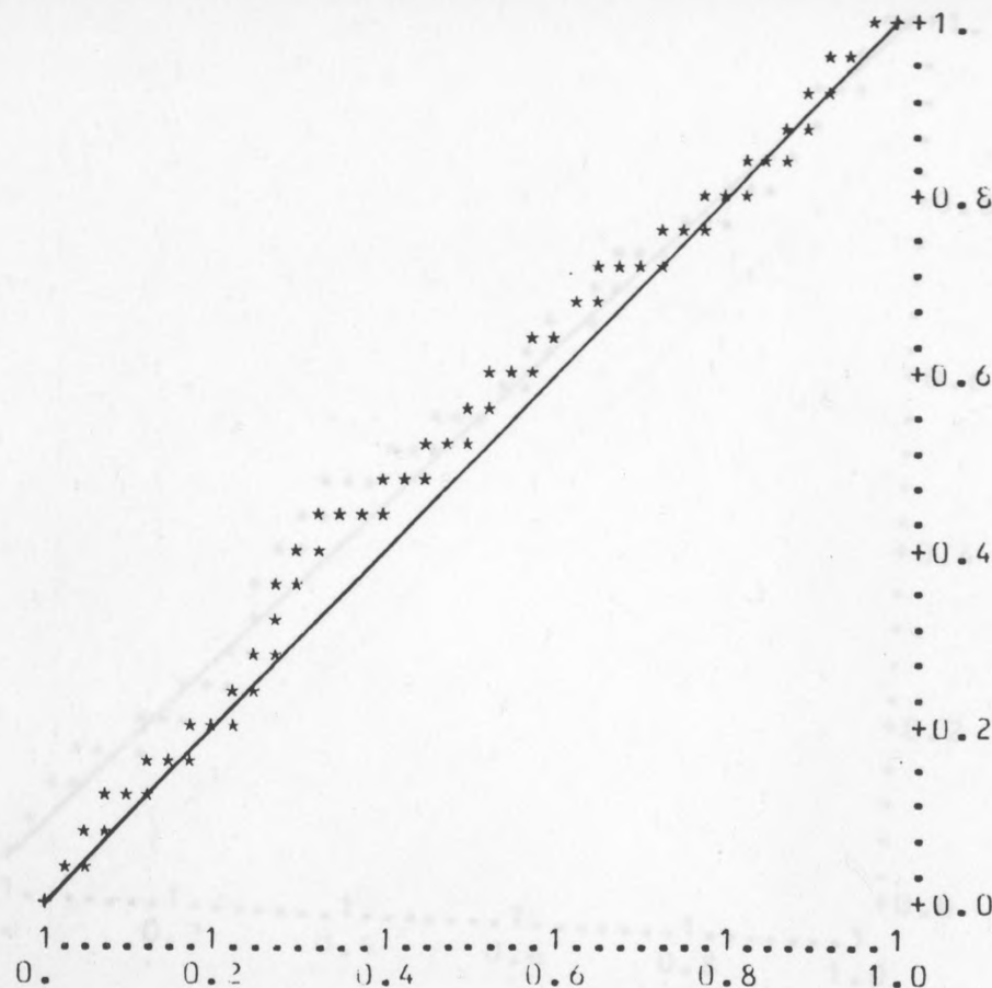
FIG. 5.54. JMNHPP u-plots, data in Table 5.4, the plots based on the line printer output.
