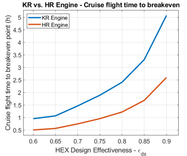
FIGURE 7: CRUISE FLIGHT TIME TO REACH BREAKEVEN POINT FOR DIFFERENT ENGINE CONFIGURATIONS.
