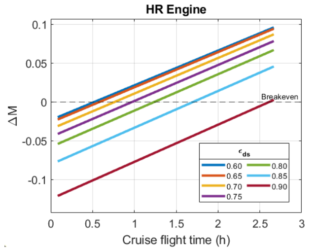
FIGURE 6: THE VARIATION OF \Delta M VERSUS CRUISE FLIGHT TIME FOR HYDROGEN RECUPERATED ENGINE.
