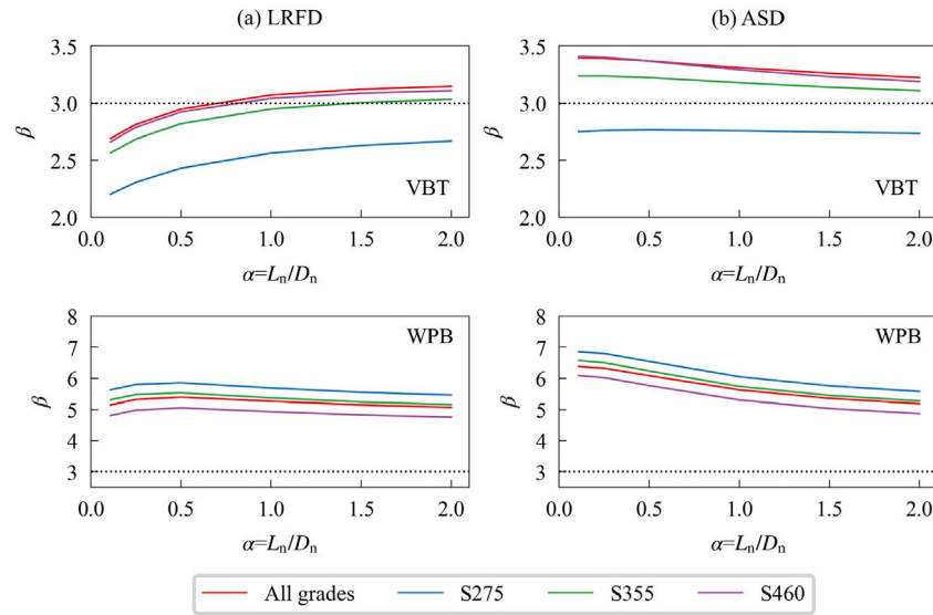
Fig. 14. iHL-RF method analysis results for AISC DG31 [2].
