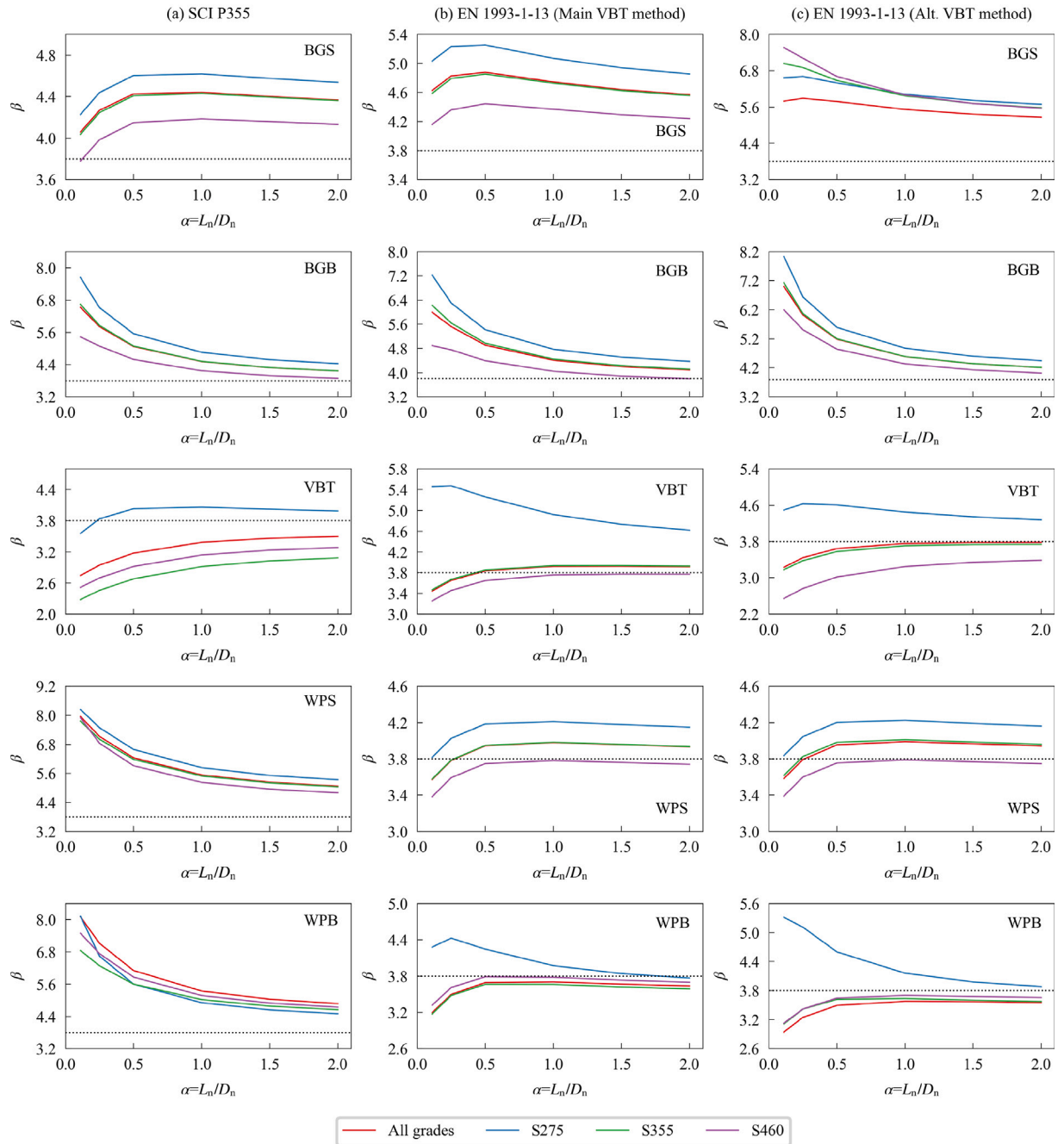
Fig. 13. iHL-RF method analysis results for SCI P355 [1] and EN 1993-1-13 [23].
