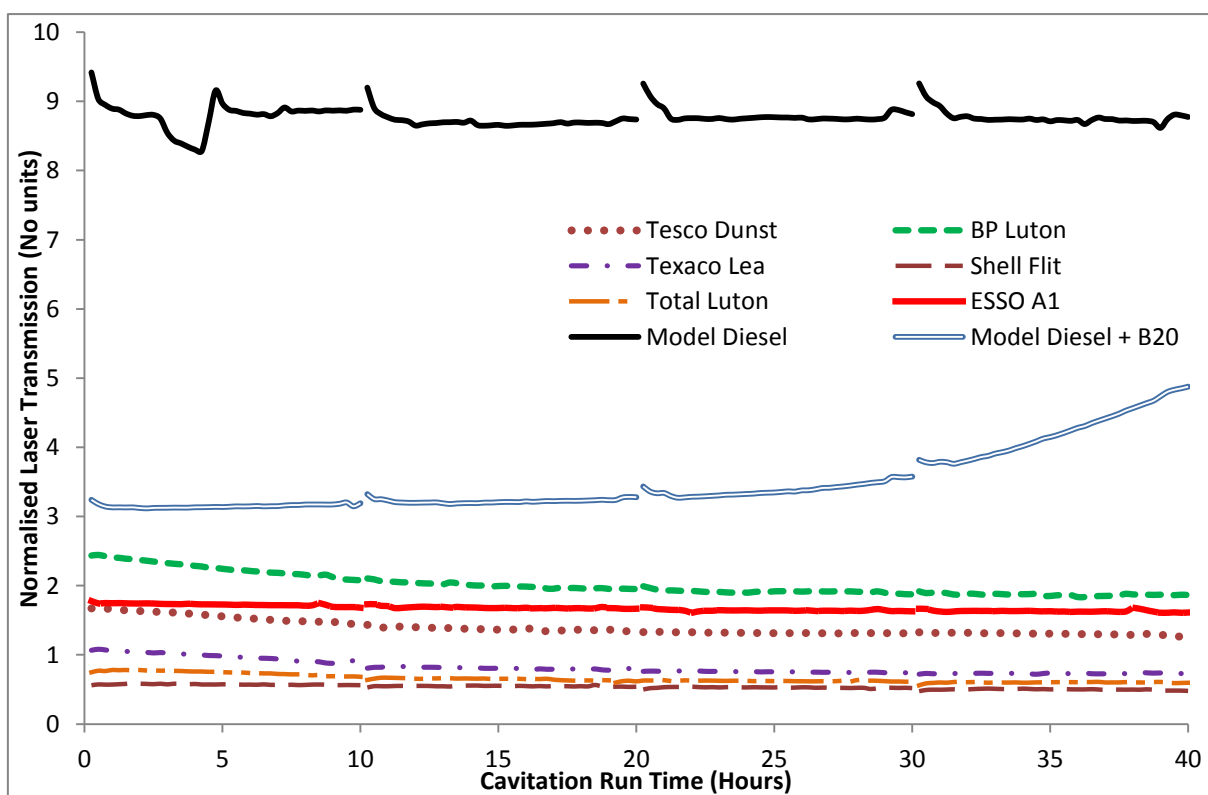
Figure 4.9 Normalised transmitted laser power as a function of cavitation time (hours) for 6 NEW commercial diesels samples and two paraffin-based model diesels
