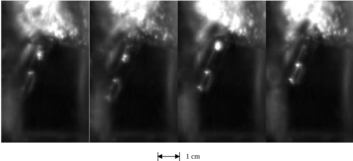
Figure 7.12 Observations showing bubbles re- entering the sac volume in the bottom hole taken from 6.3 ms – 7.8 ms (on needle seal) in steps of 0.5ms (left to right) [Image scale 1cm =0.248mm]
