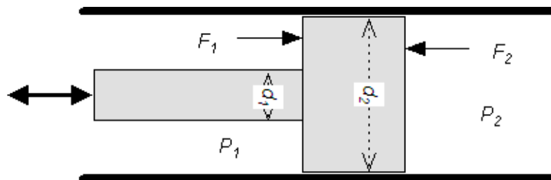
Figure 5.15 Principles of a compact cylinder
