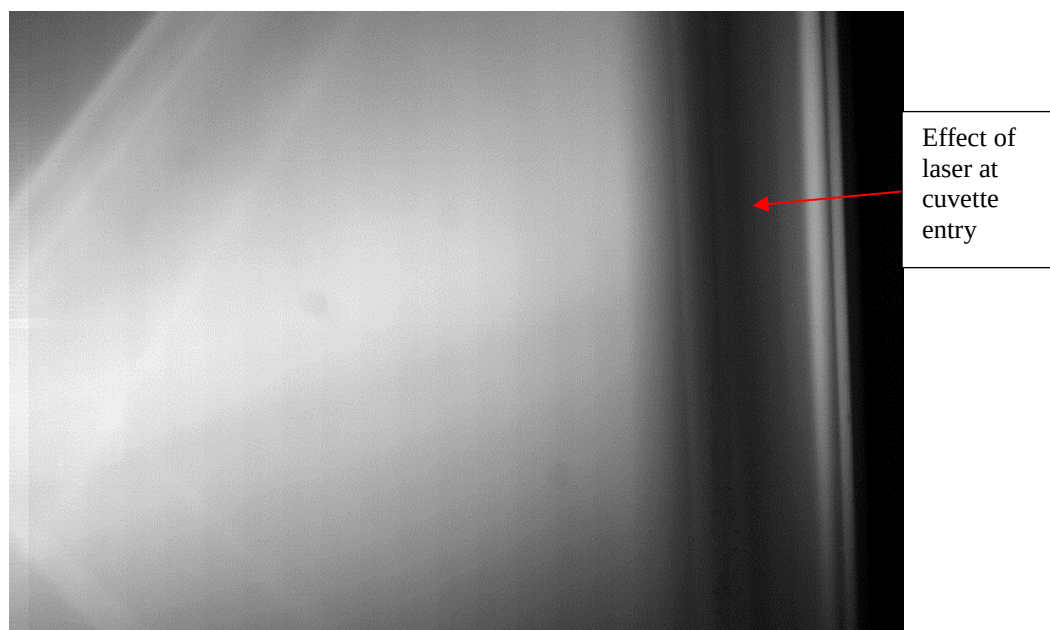
Figure 6.4 Mean laser profile at 10 kHz, 1mJ/pulse laser power.
