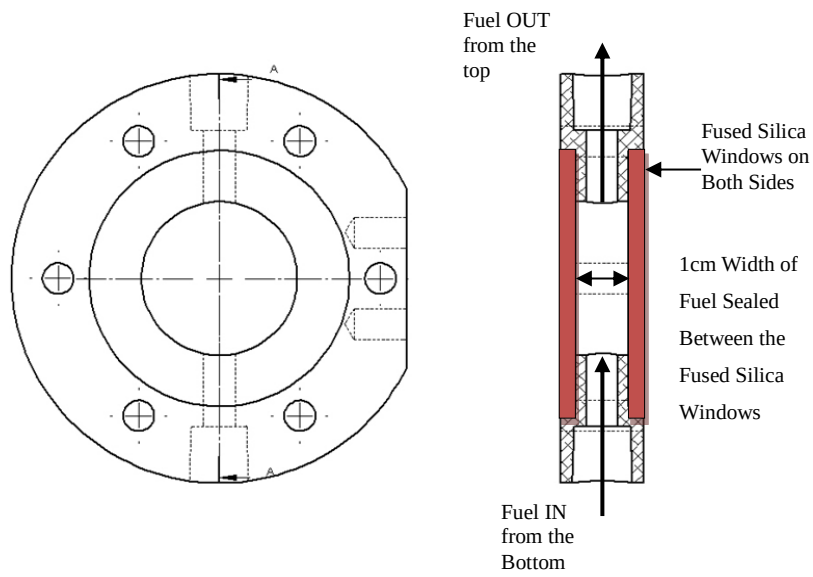
Figure 3.3 A section view of the optical cylinder
