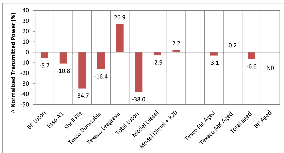
Figure 4.18 Percentage change in normalised transmitted laser power as a result of 40 hours discontinuous heat test
