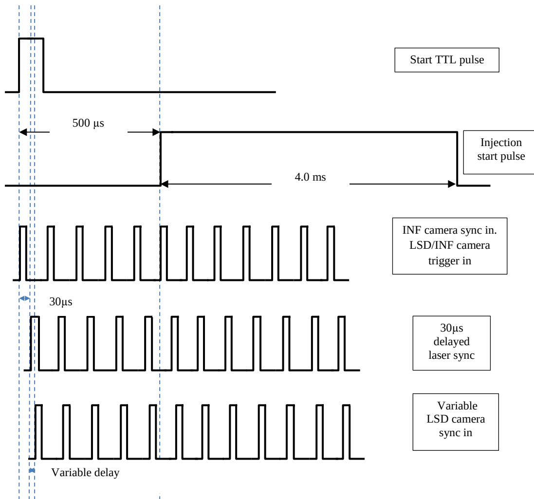
Figure 5.28 Start, injection, camera and laser synchronisation signals
