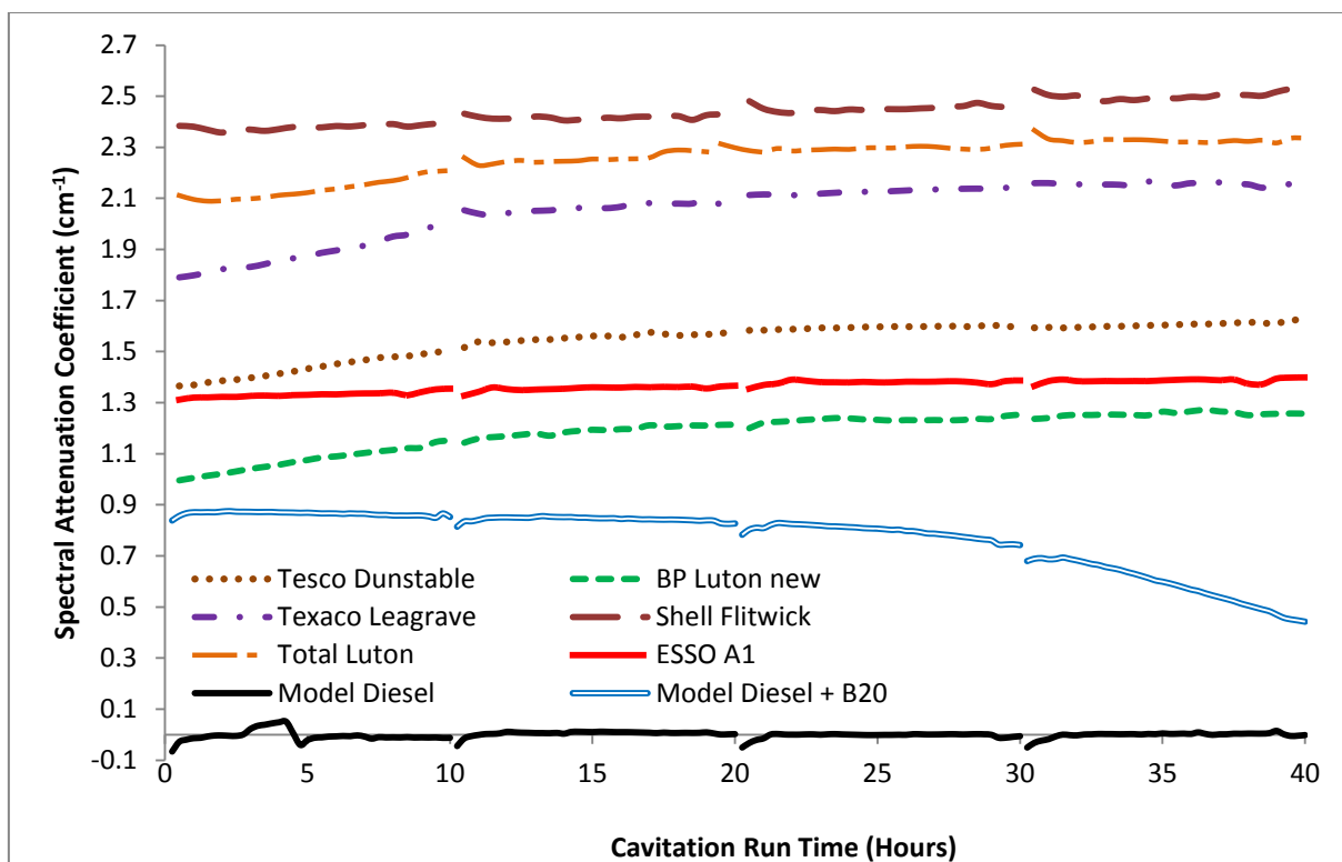
Figure 4.16 The Spectral Attenuation Coefficient ( \text{cm}^{-1} ) as a function of cavitation run time (hours) for New Commercial diesel Samples and the Paraffin based Model Sample
