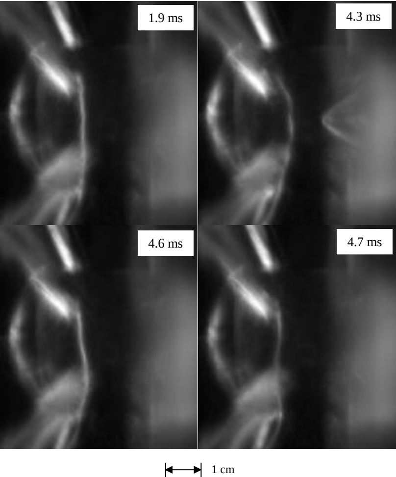
Figure 7.22 Hole to hole String cavitation observed at 350 bar injection pressure at 1.9 ms, 4.3ms, 4.6ms and 4.7ms after needle rise begun occurring during a single injection event [Image scale 1cm=0.227]
