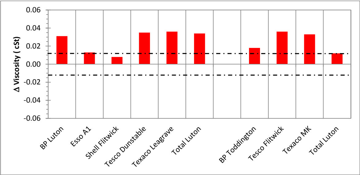
Figure 4.29 Change in Viscosity (cSt) for commercial fuels as a result of forty hours of cavitating flow
