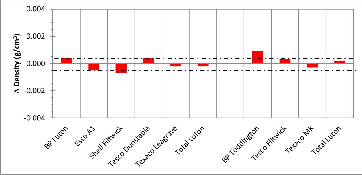
Figure 4.23 Change in Density ( \text{g/cm}^{-3} ) for commercial fuels as a result of forty hours of cavitating flow
