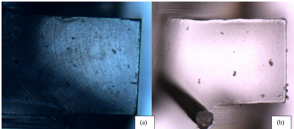
Figure 5.11 (a) unpolished side showing grains (b) polished side
