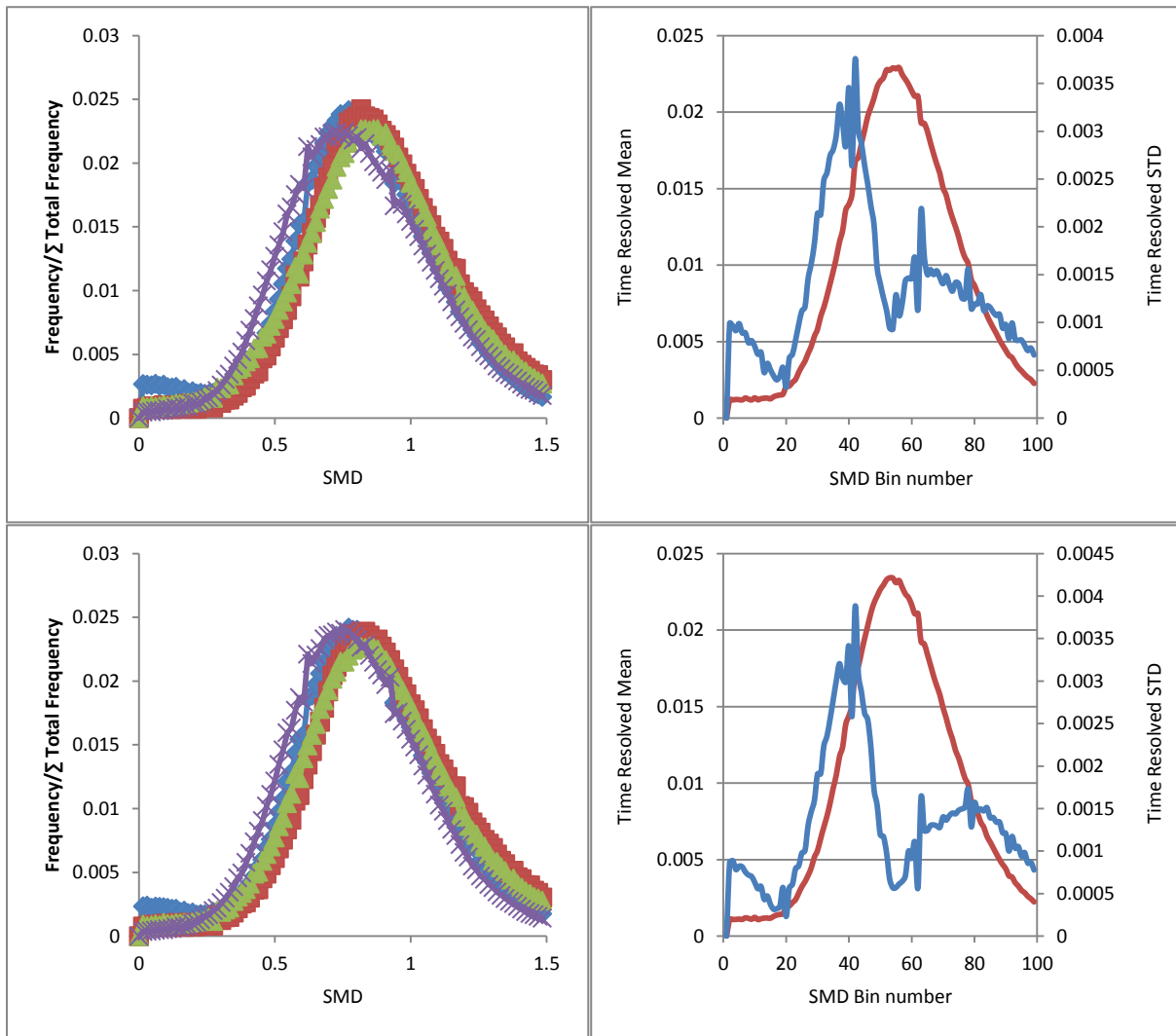
Figure C.2 Sum of BIN frequency relative SMD distributions obtained at the peak needle lift between 3.9 – 4.5 ms (top to bottom) for cases 1 – 4 and their corresponding mean and standard deviation
