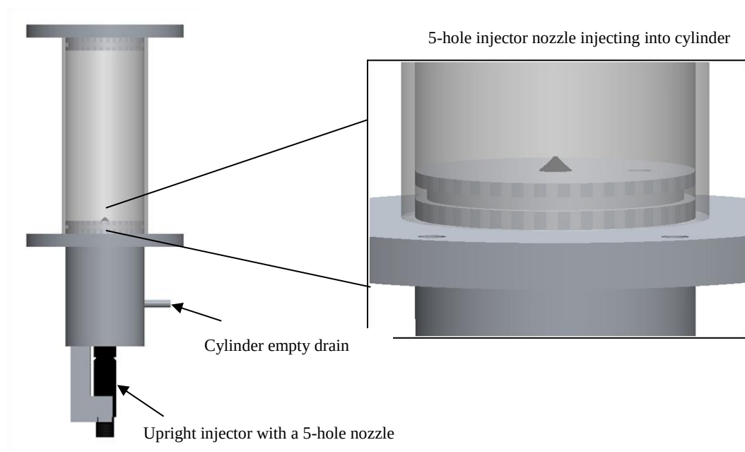
Figure 3.2 Injector setup
