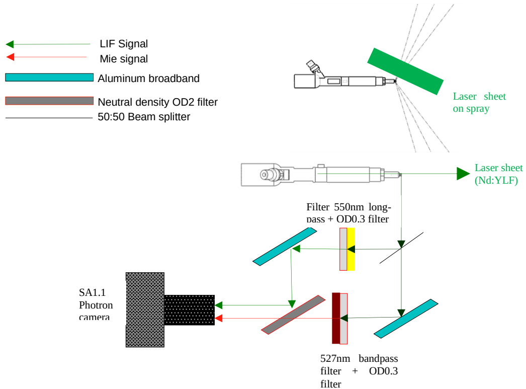
Figure 5.23 The image doubler, filter and camera setup
