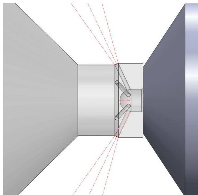
Figure 5.26 Image the INF camera would capture.
