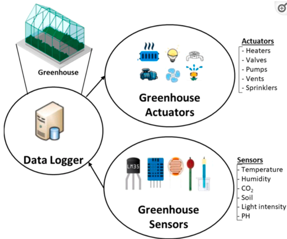
Fig. 2. Data sources in a smart greenhouse with multiple IoT sensors [13].
