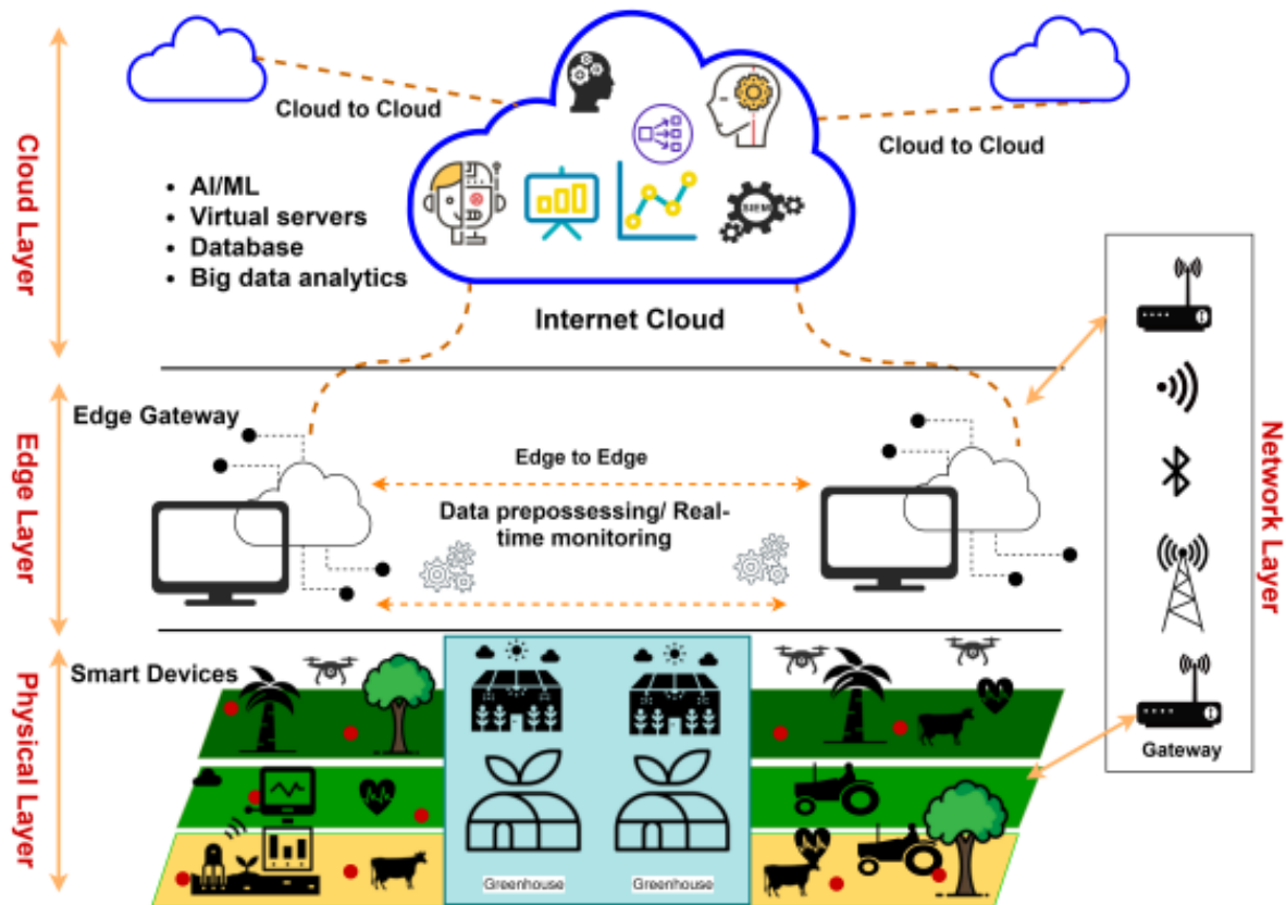
Figure 14. Smart agricultural system infrastructure (Yazdinejad et al., 2021).
