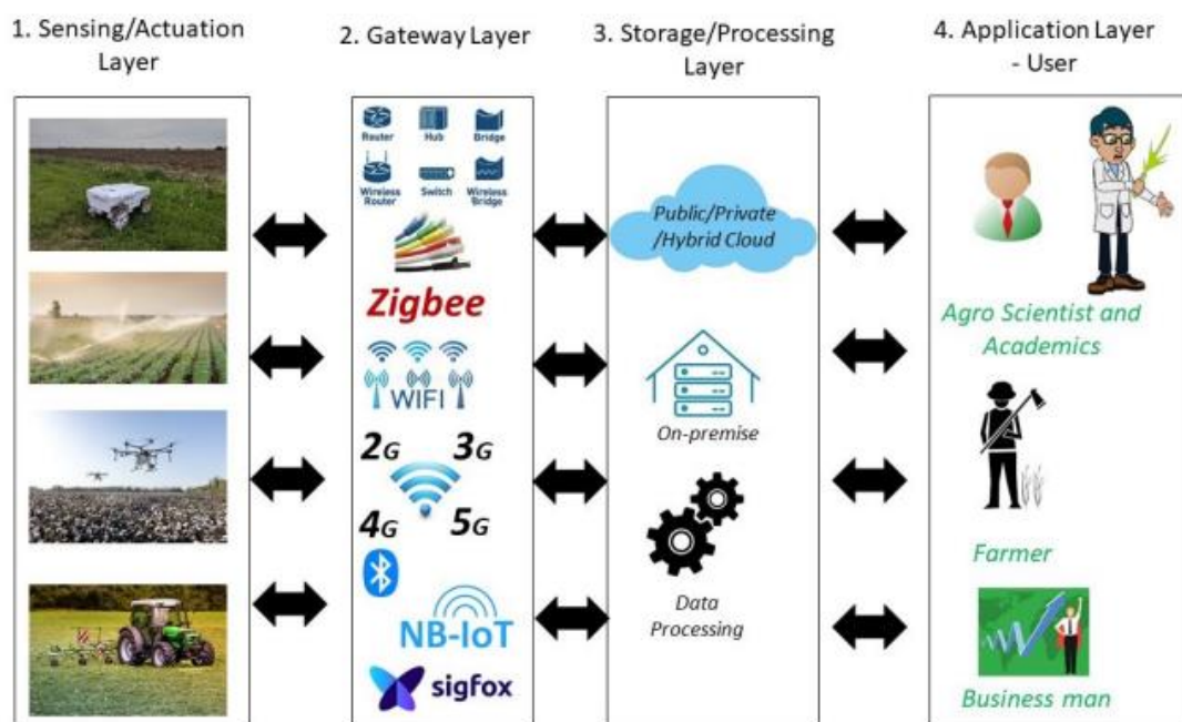
Figure 5. Layers targeted during attacks on smart agricultural systems (Alahmadi et al., 2022)
